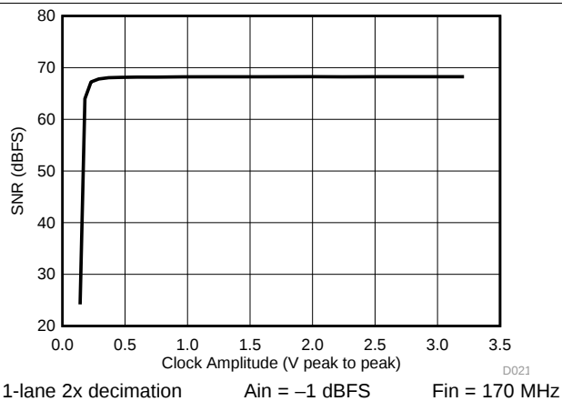
FIG 25. SNR vs. Clock Amplitude
