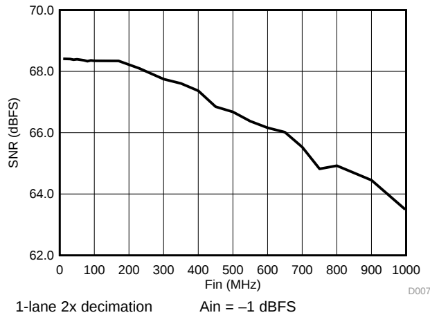
FIG 11. SNR vs. Frequency
