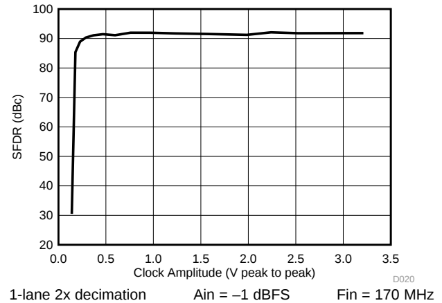
FIG 24. SFDR vs. Clock Amplitude
