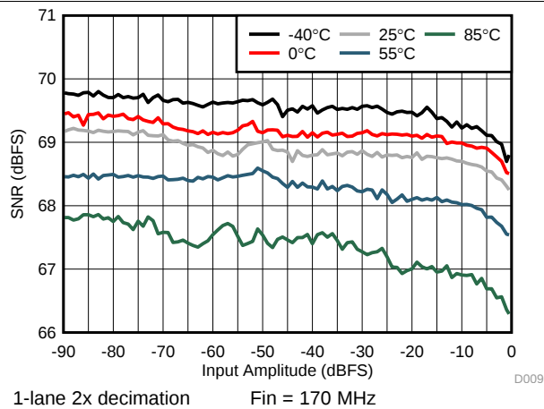
FIG 13. SNR vs. Amplitude
