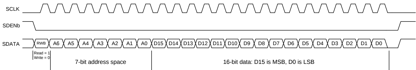
図 71. Serial Register Read Timing Diagram
