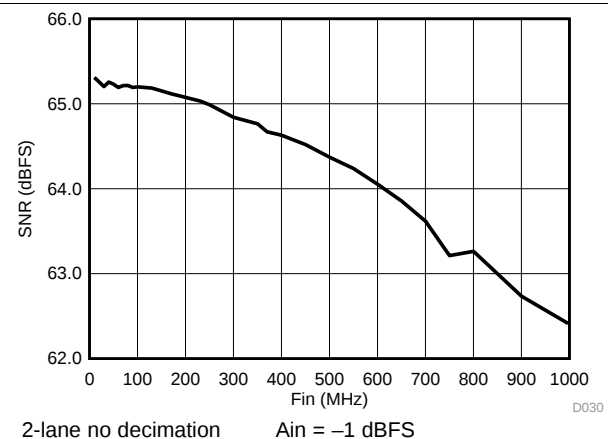
图 34. SNR vs Frequency
