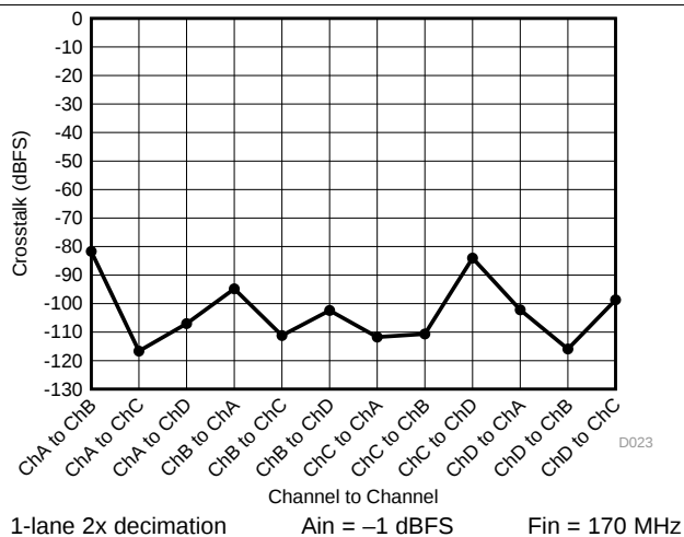
FIG 27. Crosstalk by Channel
