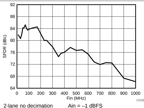
图 33. SFDR vs Frequency
