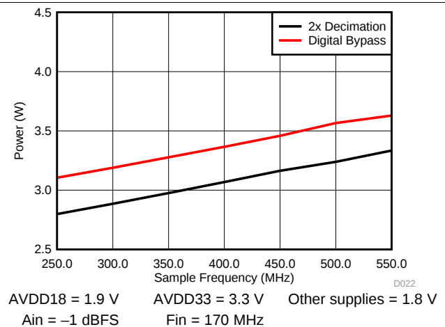
FIG 26. Power vs Sample Frequency
