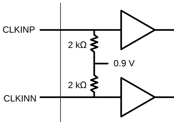
FIG 68. Equivalent Clock Input Circuit
