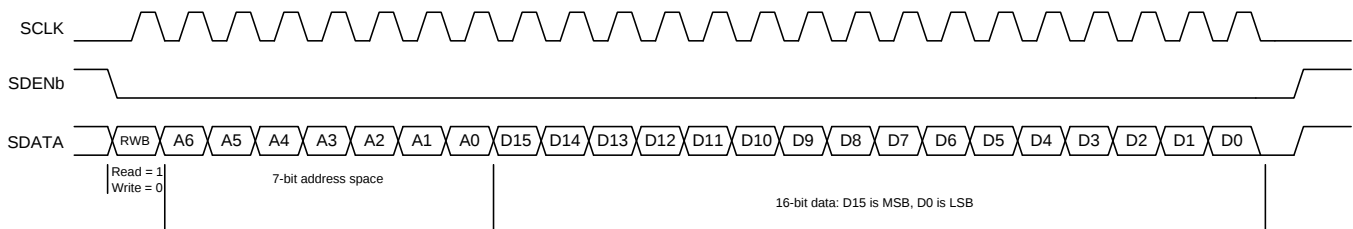
図 70. Serial Register Write Timing Diagram
