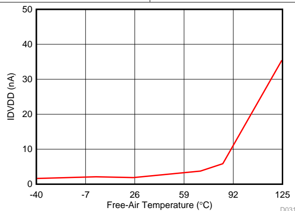
图 27. I_{DVDD} in Manual Mode with SCL
