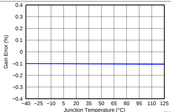
Figure 15. PA Gain Error vs Temperature
