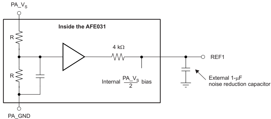
Figure 35. REF1 Functional Diagram
