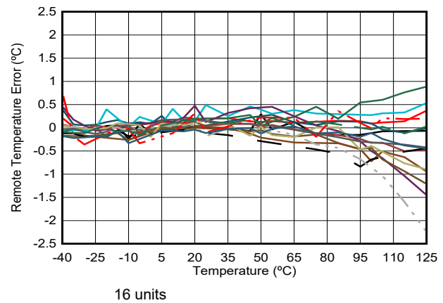
図 6-49. Remote Temperature Error vs Temperature
