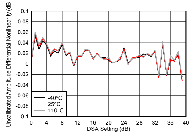
6-189. TX DSA Uncalibrated Amplitude Differential Nonlinearity at 8.11 GHz
