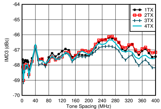
f_{\text{DAC}} = 11796.48\text{MSPS} , interleaved mode, matching at 4.9 GHz, f_{\text{CENTER}} = 4.9\text{GHz} , -13\text{ dBFS} each tone
