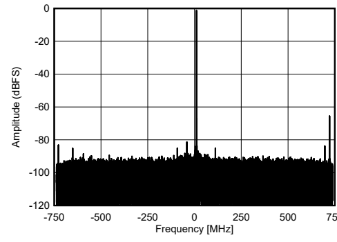
6-482. RX Single Tone Output FFT at 9.61 GHz
