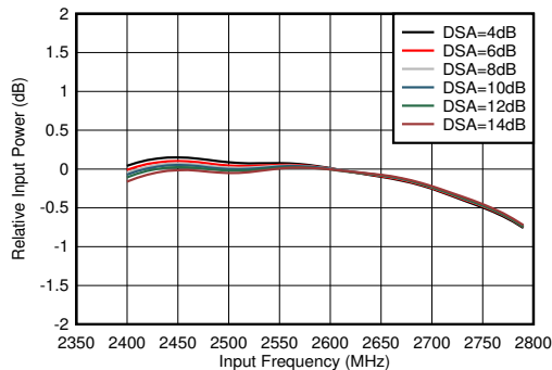
FIG 6-348. RX Inband Gain Flatness, f_{IN} = 2600\text{ MHz}
