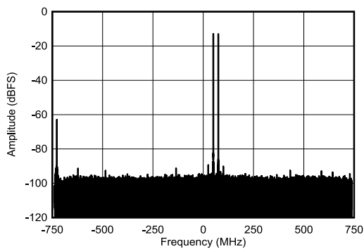
External clock mode, -13dBFS each tone
