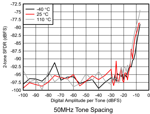
6-456. RX 2-tone SFDR vs Digital Amplitude at 8.11GHz
