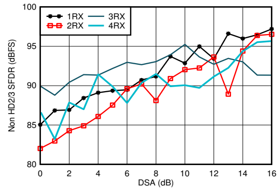
6-314. RX Non-HD2/3 vs DSA Setting at 0.8 GHz
