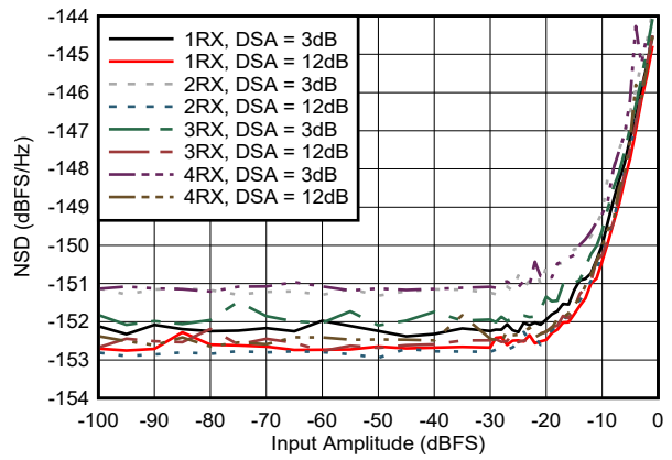
6-449. RX NSD vs Digital Amplitude at 8.1GHz
