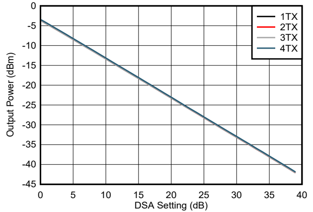
6-185. TX Output Power vs DSA Setting at 8.11 GHz
