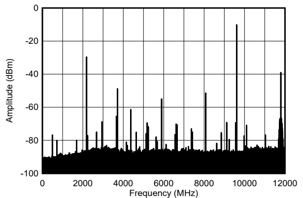
6-266. TX Single Tone Spectrum at 9.61 GHz and -1dBFS (wideband)
