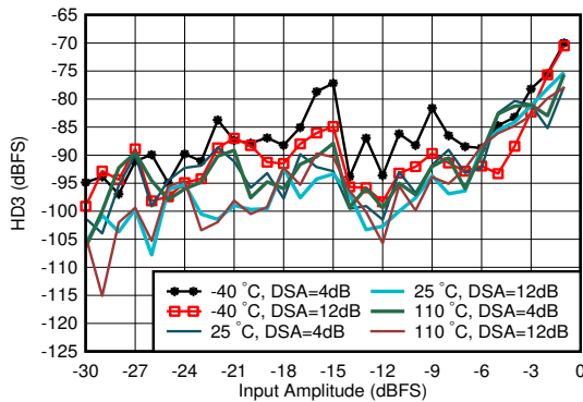
6-313. RX HD3 vs Input Level and Temperature at 0.8 GHz
