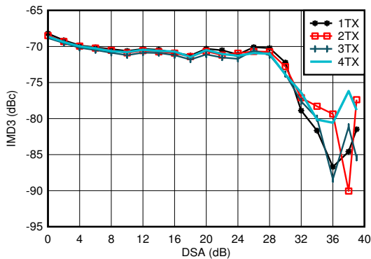
f_{\text{DAC}} = 11796.48\text{MSPS} , interleaved mode, matching at 4.9 GHz, f_{\text{CENTER}} = 4.9\text{GHz} , -13\text{ dBFS} each tone
