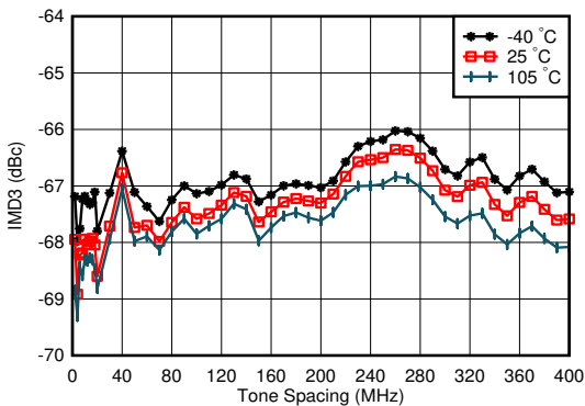
f_{\text{DAC}} = 11796.48\text{MSPS} , interleaved mode, matching at 4.9 GHz, f_{\text{CENTER}} = 4.9\text{GHz} , -13\text{ dBFS} each tone, worst channel
