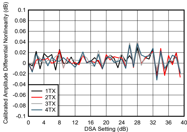
6-188. TX DSA Calibrated Amplitude Differential Nonlinearity at 8.11 GHz
