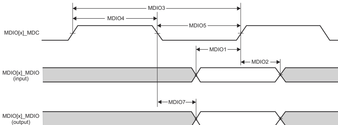
CPSW2G_MDIO_TIMING_01
