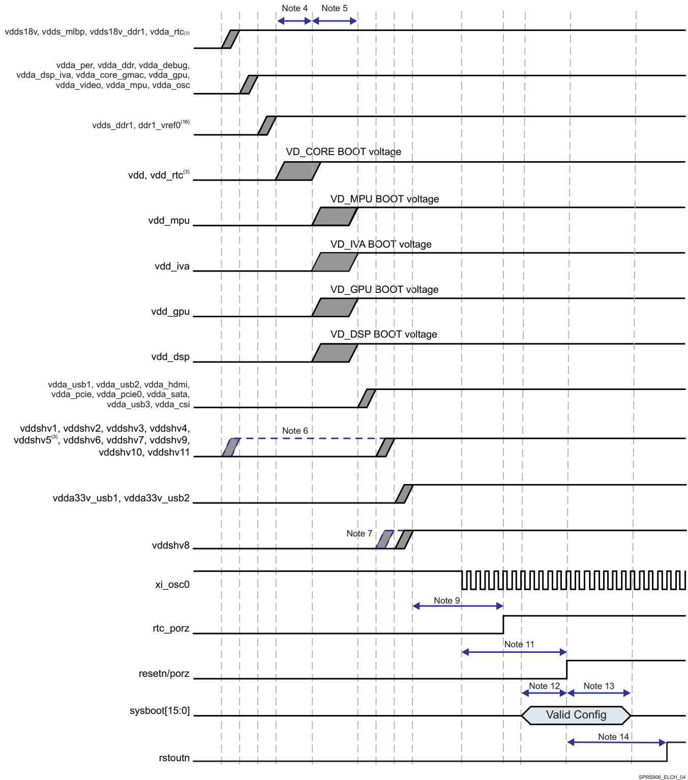
Figure 5-2. Power-Up Sequencing
