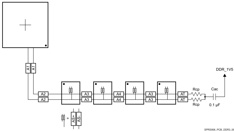
Figure 8-8. CK Routing for Four Single-Side DDR3 Devices
