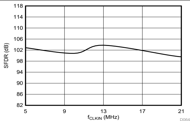
FIG 6-31. Spurious-Free Dynamic Range vs Clock Frequency
