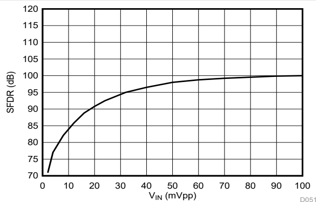
FIG 6-33. Spurious-Free Dynamic Range vs Input Signal Amplitude
