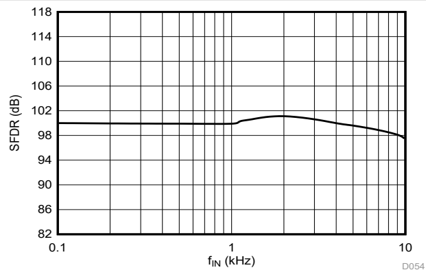
FIG 6-32. Spurious-Free Dynamic Range vs Input Signal Frequency
