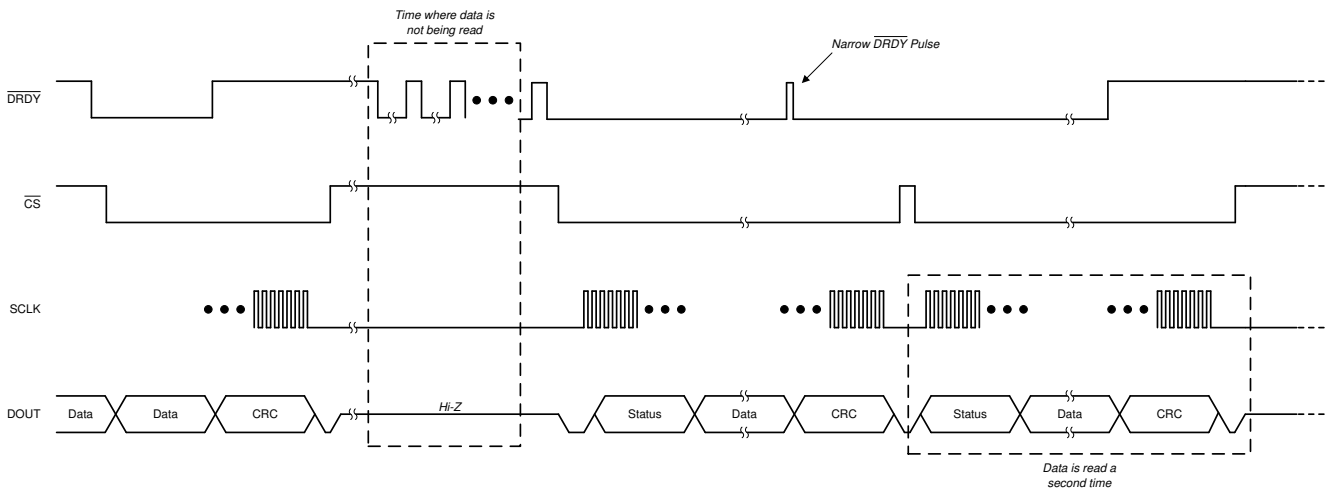
图 8-32. Collecting Data After a Pause by Reading Data Twice
