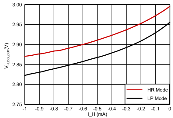
6-23. HLDO Output Voltage vs Load Current
