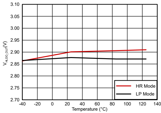
6-22. HLDO Output Voltage vs Temperature
