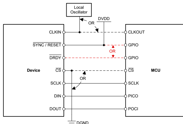
9-2. Minimum Connections Required to Operate the AMC131M03-Q1
