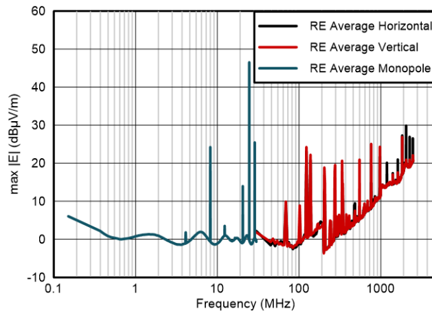
9-5. AMC131M03-Q1 Radiated Emission CISPR25 Measurement
