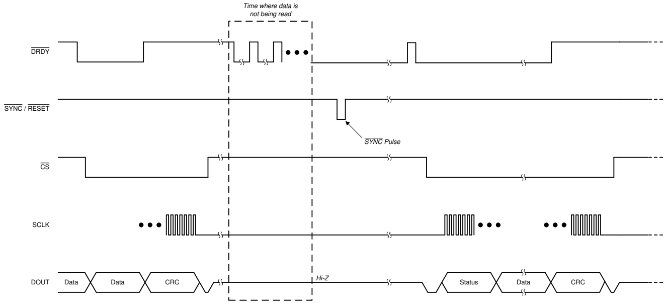
图 8-31. Collecting Data After a Pause Using the SYNC/RESET Pin
