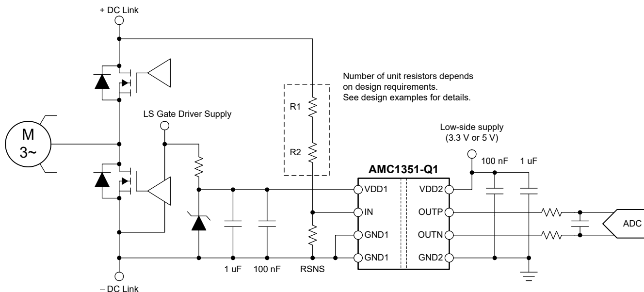
8-1. Using the AMC1351-Q1 for DC Link Voltage Sensing in Frequency Inverters
