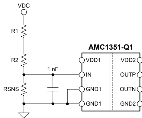
Figure 8-2. Input Filter
