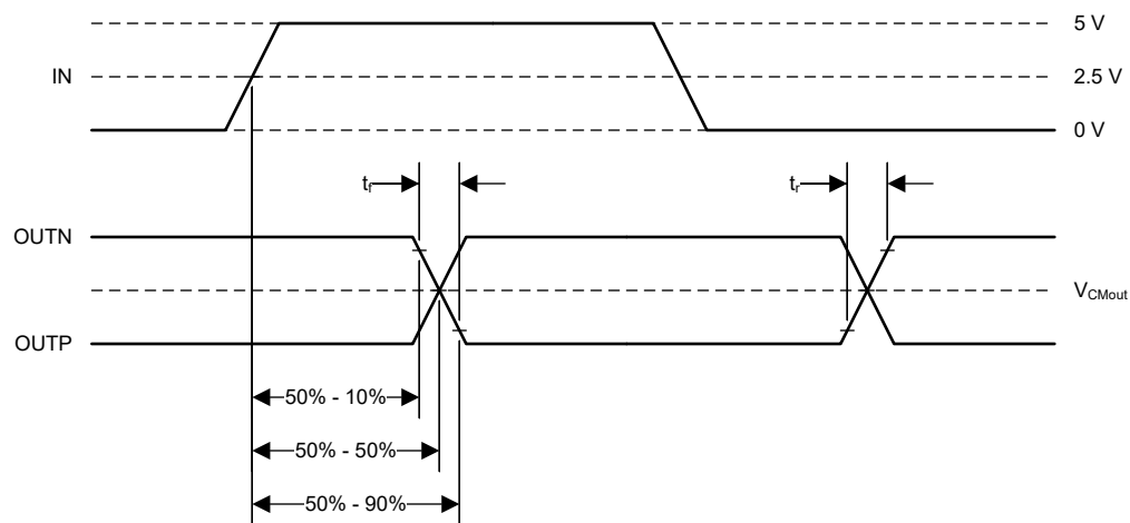
FIG 6-1. Rise, Fall, and Delay Time Definition
