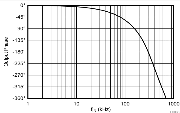
图 6-35. Output Phase vs Input Frequency
