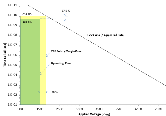
图 6-4. Reinforced Isolation Capacitor Lifetime Projection
