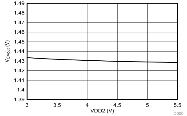
图 6-32. Common-Mode Output Voltage vs Supply Voltage
