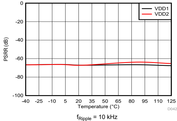
图 6-31. Power-Supply Rejection Ratio vs Temperature
