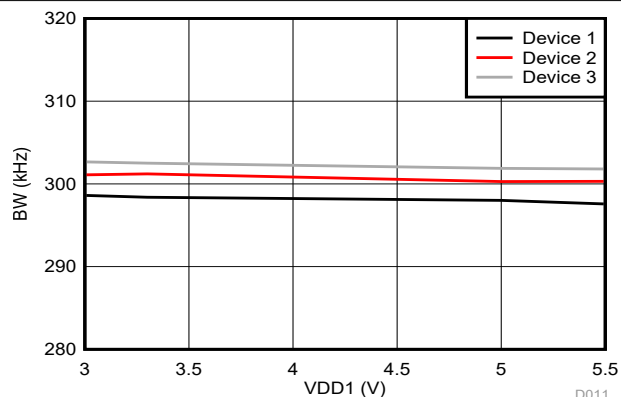
图 6-36. Bandwidth vs Supply Voltage
