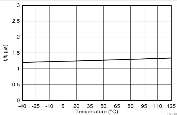
FIG 6-41. Output Rise and Fall Time vs Temperature
