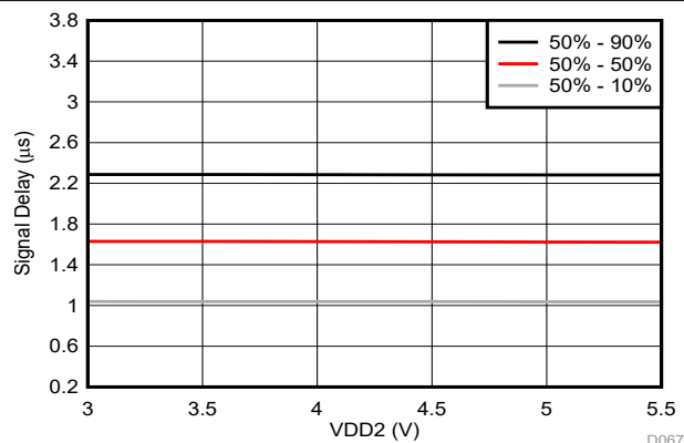
FIG 6-42. Input to Output Signal Delay vs Supply Voltage
