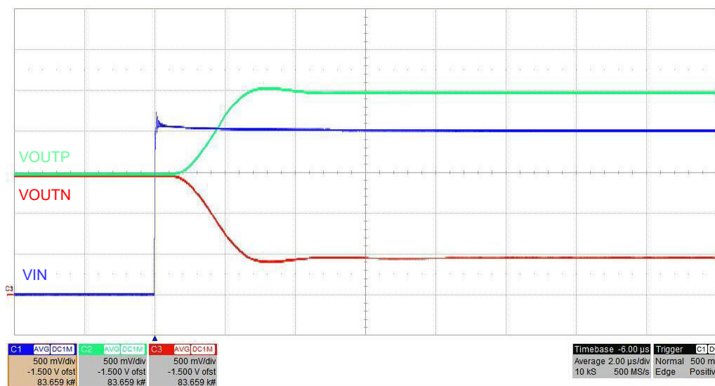
Figure 8-4. Step Response of the AMC3311
