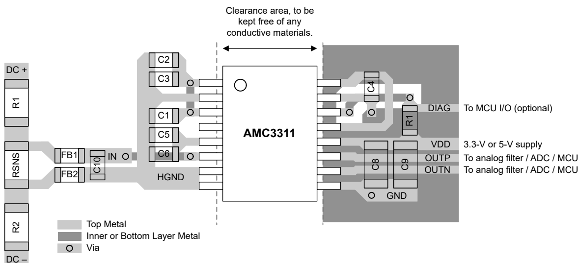
✎ 8-6. Recommended Layout of the AMC3311
