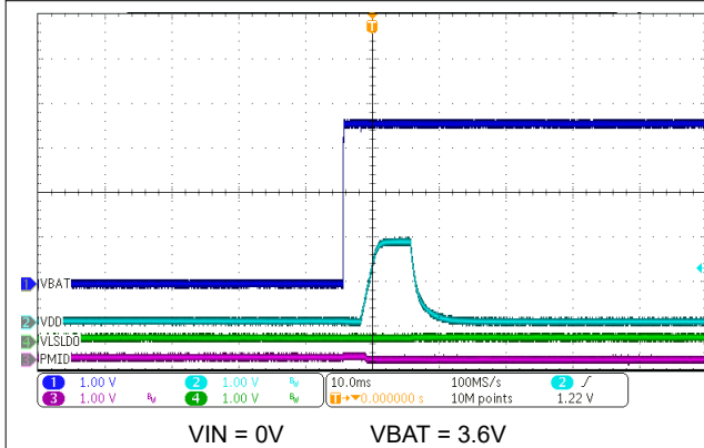
8-4. Wake In To Ship Mode on Battery Insertion with No IN Supply
