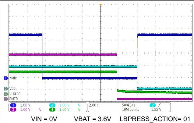
8-7. Ship Mode Entry with \overline{MR} Long Button Press
