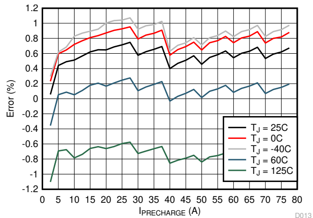
6-4. Pre-Charge Current Accuracy vs. IPRECHARGE Setting (ICHARGE_RANGE = 1)
