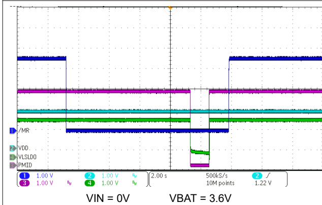
8-6. HW Reset on \overline{MR} Long Button Press
