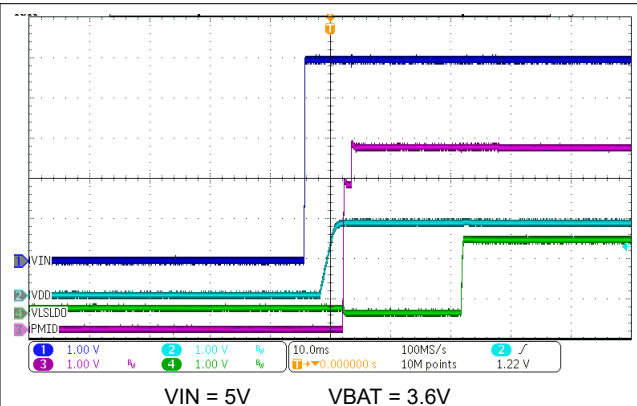
8-3. Power Up from Ship Mode with IN Supply Insertion
