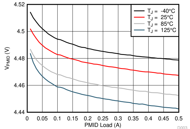
6-14. PMID Load Regulation vs. Temperature
