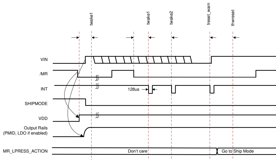
Fig 7-4. MR Wake from Ship Mode – VIN Dependencies
