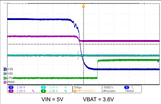
8-11. \overline{\text{PG}} Power Good Function - IN Supply Removal
