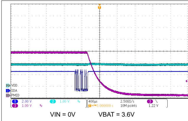
8-8. HW Reset Through I 2 C Command
