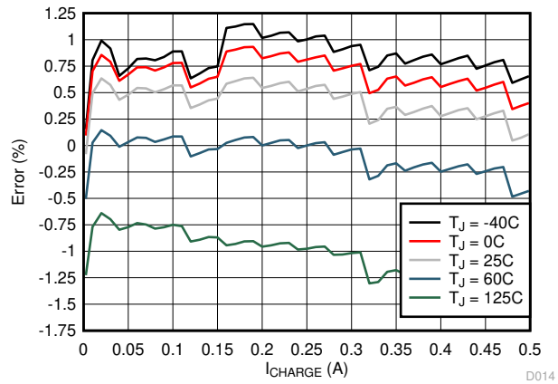
6-2. Charge Current Accuracy vs. ICHARGE Setting
