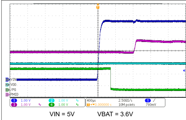
8-10. \overline{\text{PG}} Power Good Function - IN Supply Insertion
