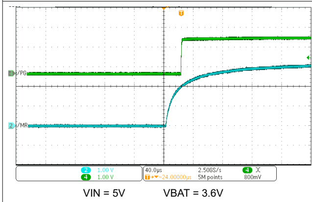
8-12. \overline{\text{PG}} \overline{\text{MR}} Level Shift Function - \overline{\text{MR}} Rising
