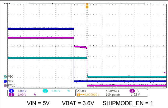
8-9. Ship Mode Entry on IN Supply Removal
