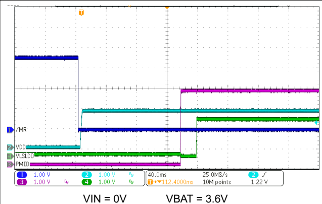
8-5. Power Up from Ship Mode with \overline{MR} Press
