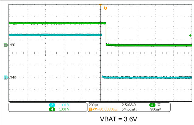
8-13. \overline{\text{PG}} \overline{\text{MR}} Level Shift Function - \overline{\text{MR}} Falling
