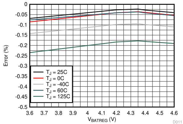
6-1. Battery Regulation Voltage Accuracy vs. VBATREG Setting
