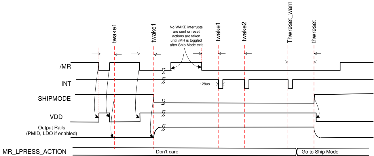
Fig 7-3. MR Wake from Ship Mode (MR_LPRESS_ACTION = Ship Mode, VIN not valid)
