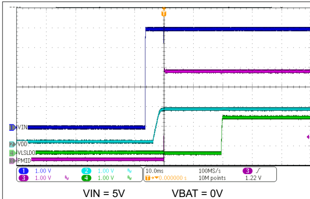
8-2. Power Up from IN Supply Insertion with No Battery
