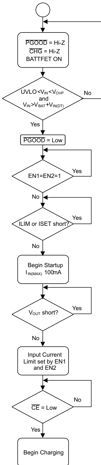
19. Startup Flow Diagram
