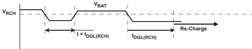
⊠ 3. Recharge – t_{DGL(RCH)}
