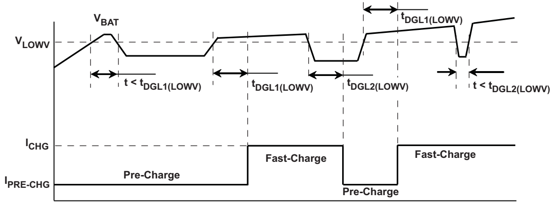
⊠ 2. Pre- to Fast-Charge, Fast- to Pre-Charge Transition – t_{DGL1(LOWV)} , t_{DGL2(LOWV)}
