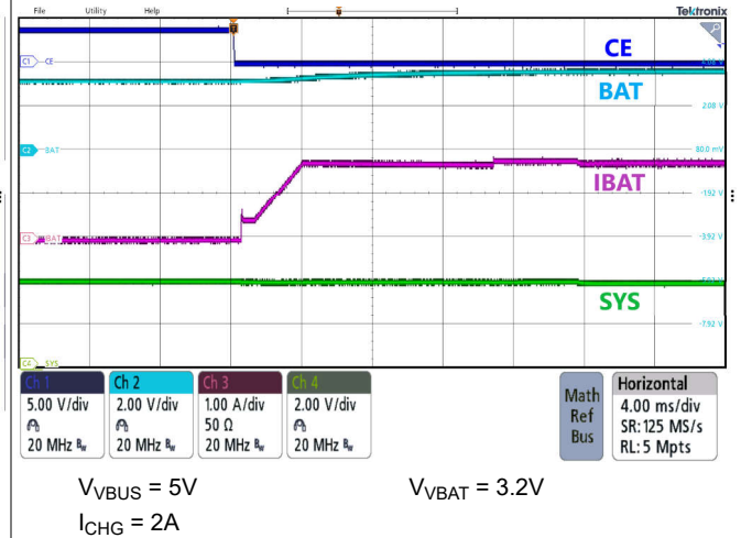
Figure 8-5. Charge Enable
