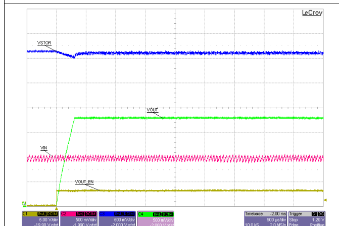
VIN_DC = 2.0 V power supply 100Ω series resistance VBAT = 3.1-V charged Li coin cell
