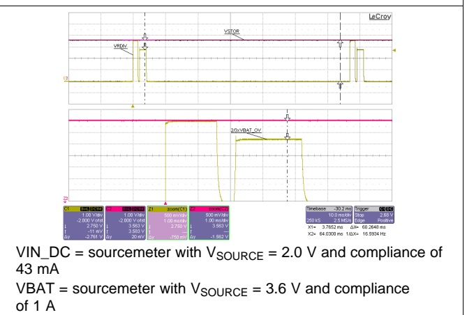
Figure 28. VRDIV Waveform
