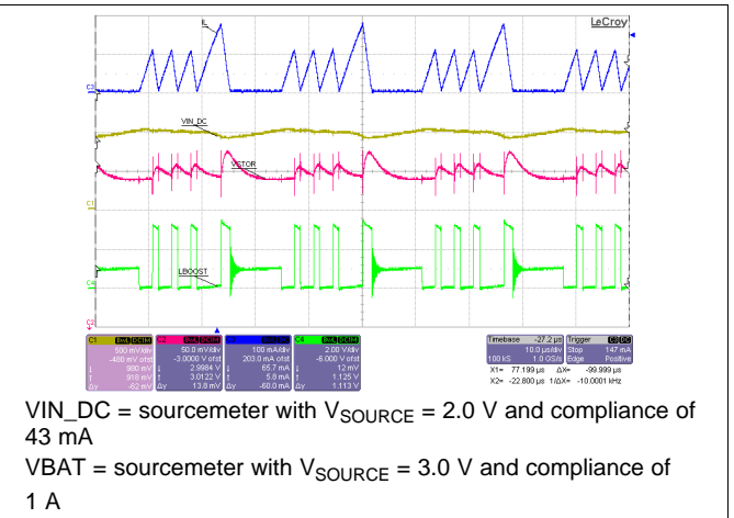
Figure 26. Boost Charger Operational Waveforms
