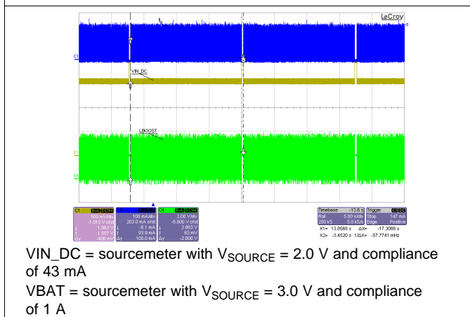
Figure 27. MPPT Operation
