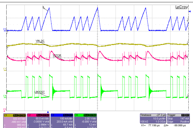
VIN_DC = sourcemeter with V_{SOURCE} = 2.0\text{ V} and compliance of 43 mA VBAT = sourcemeter with V_{SOURCE} = 3.0\text{ V} and compliance of 1 A
