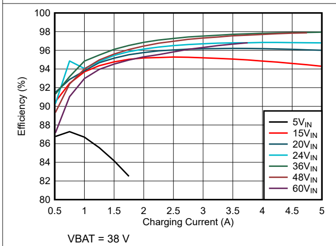
Figure 6-3. Charge Efficiency vs Charge Current (10s battery configuration)
