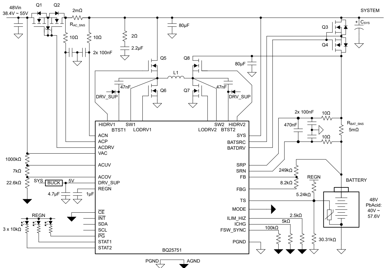
Figure 8-1. BQ25751: Standalone, 48VAC with 48V Lead-Acid Battery and 10A Charge Current
