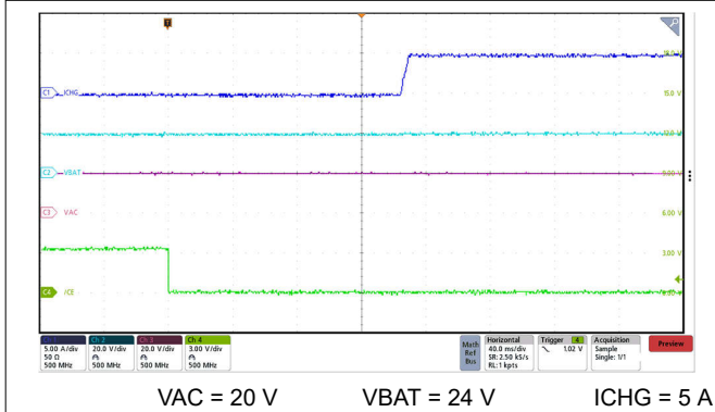
Figure 8-7. Charge Enable via \overline{CE} Pin with 5-A ICHG
