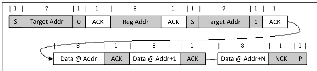
Figure 7-14. Multi-Read
