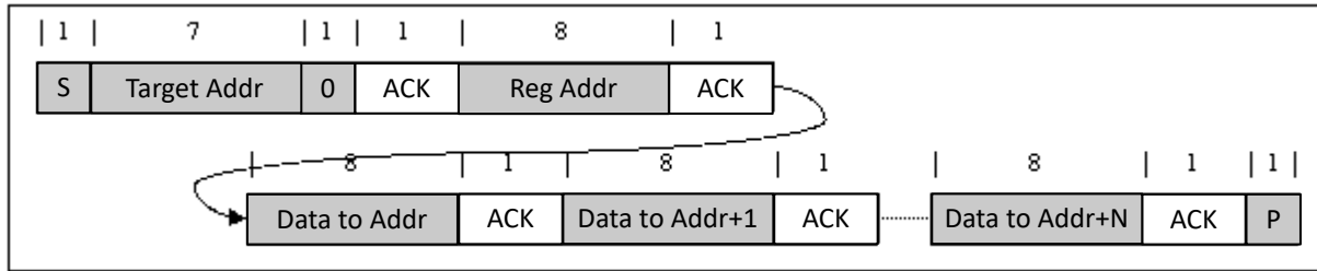
Figure 7-13. Multi-Write
