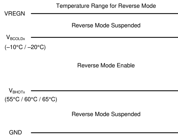
Figure 7-4. TS Pin Thermistor Sense Threshold in Reverse Mode
