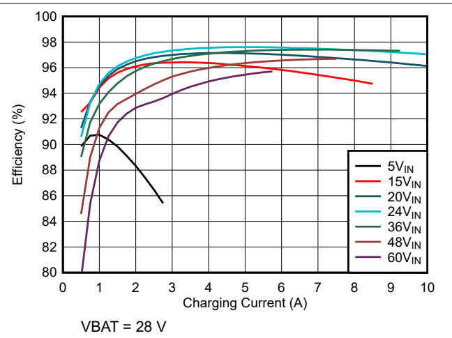
Figure 6-2. Charge Efficiency vs Charge Current (7s battery configuration)
