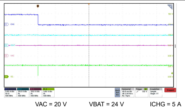
Figure 8-6. Charge Disable via I 2 C with 5-A ICHG
