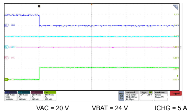
Figure 8-8. Charge Disable via \overline{CE} Pin with 5-A ICHG
