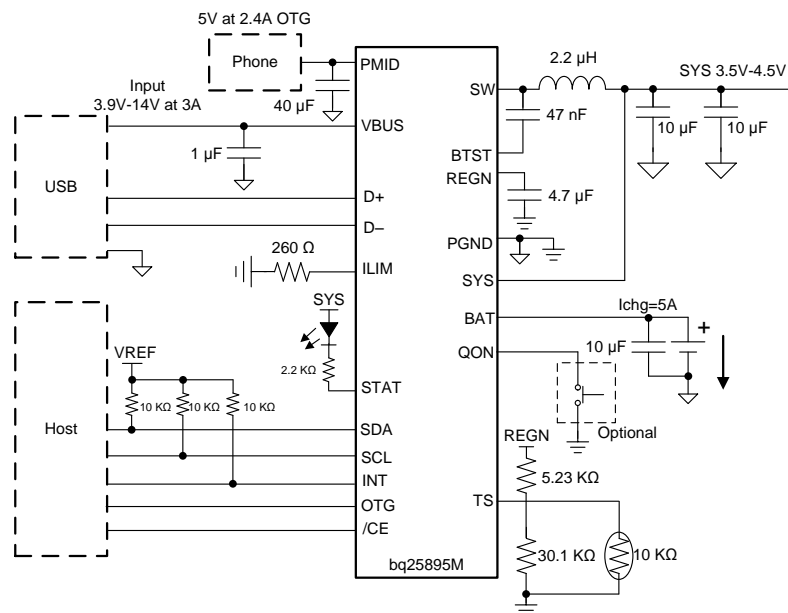
图 47. bq25895M with D+/D- Interface and 2.4 A Boost Mode Output
