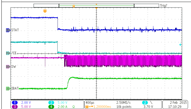
48. Power Up with Charge Disabled
