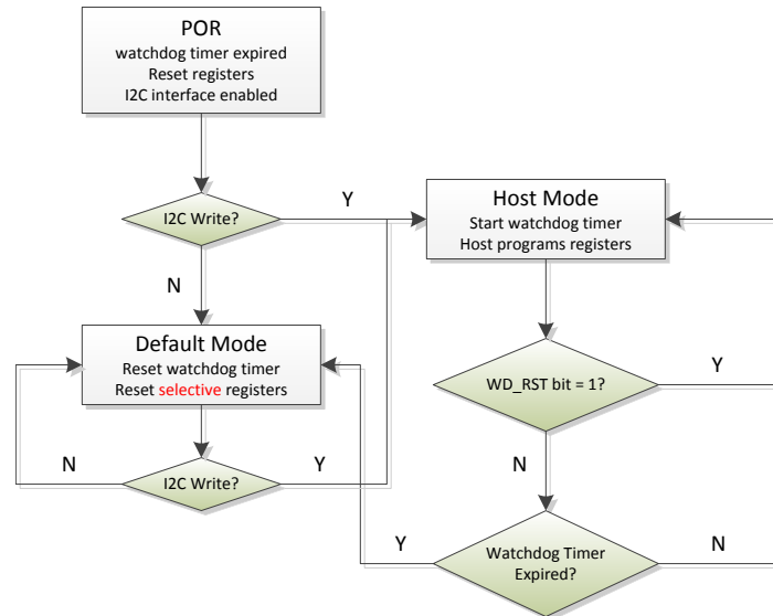
25. Watchdog Timer Flow Chart
