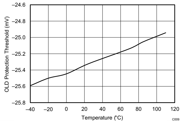
7-7. Overcurrent Discharge Protection Threshold vs Temperature Threshold setting is 25 mV.
