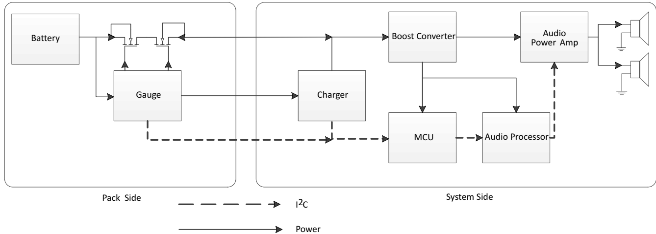
9-2. Wireless (Bluetooth) Speaker Application Block Diagram
