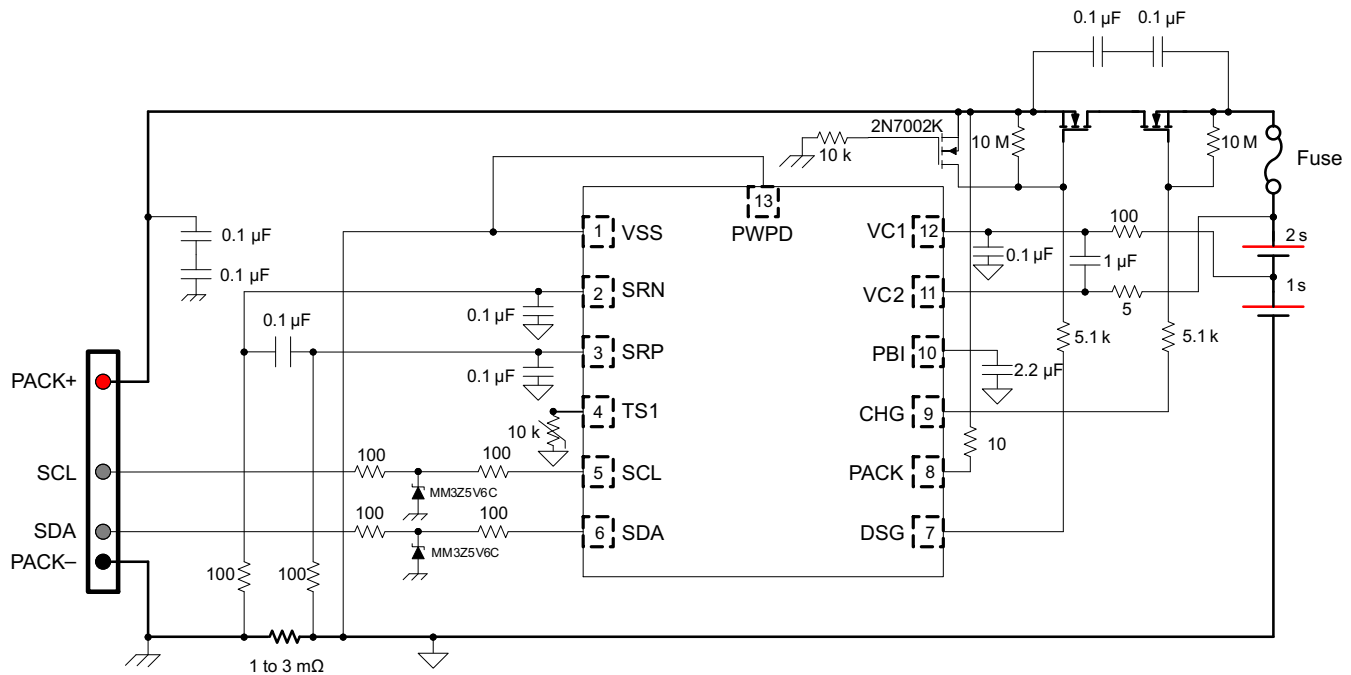
図 9-1. BQ28Z610-R1 2-Series Cell Typical Implementation
