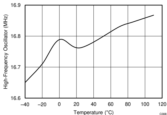
FIG 8-6. High-Frequency Oscillator vs. Temperature
