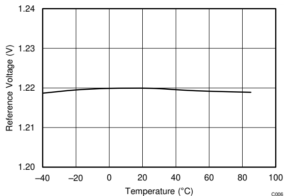
FIG 8-4. Reference Voltage vs. Temperature
