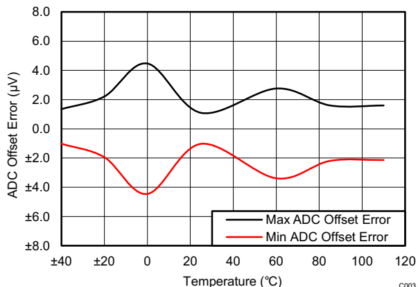
FIG 8-3. ADC Offset Error vs. Temperature
