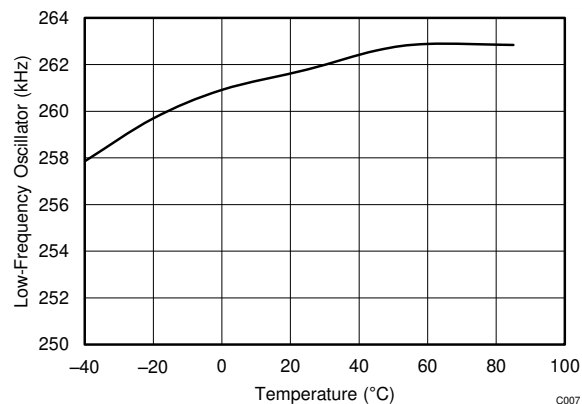
FIG 8-5. Low-Frequency Oscillator vs. Temperature
