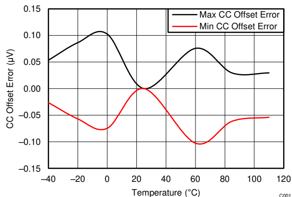
FIG 8-2. CC Offset Error vs. Temperature
