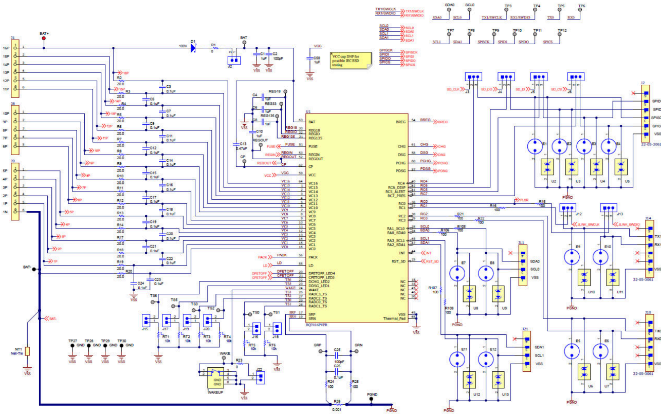
図 8-1. Typical Applications
