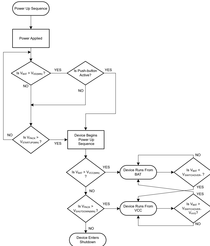
7-1. Power-Up Sequence
