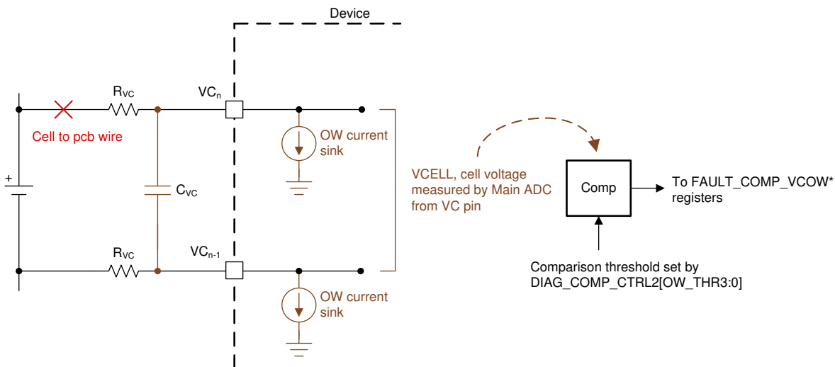
图 8-51. Open Wire Detection
