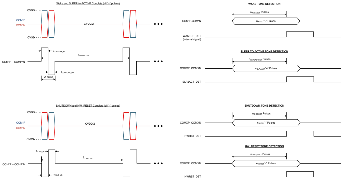
8-63. Communication Tones
