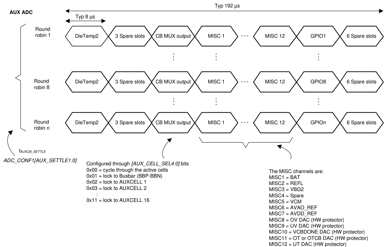
8-9. AUX ADC Round Robin Measurements
