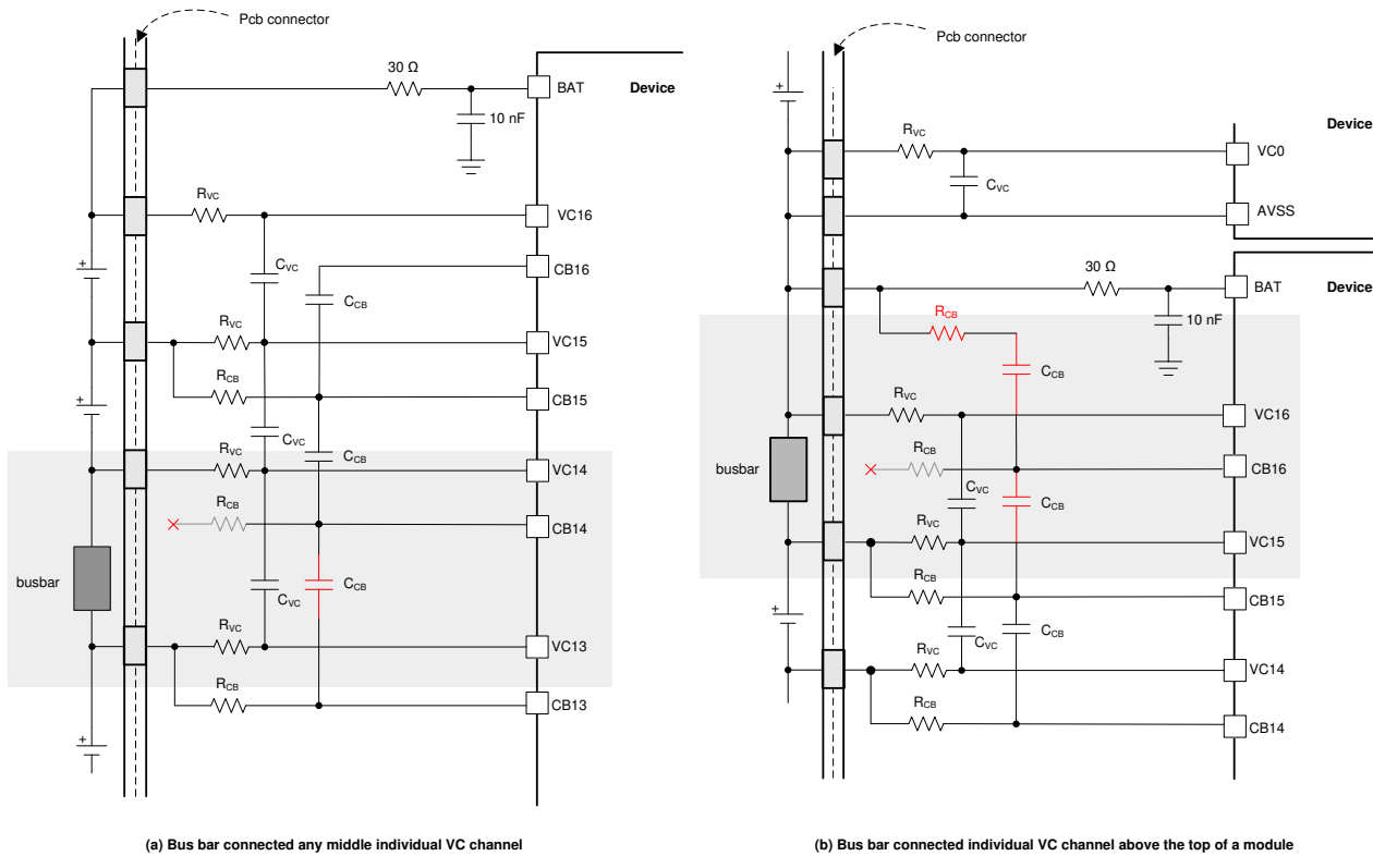
8-56. Bus Bar Connected to Individual VC Channel
