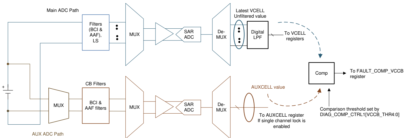
8-47. Cell Voltage Measurement Diagnostic
