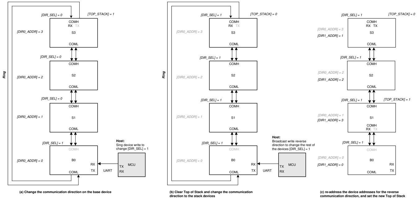
8-37. Example to Change Communication Direction in Daisy Chain
