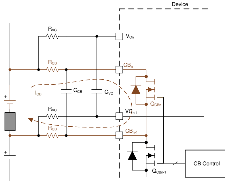
8-53. Cell Balancing with Bus Bar (Through BBP/N) Sharing a Cell Channel
