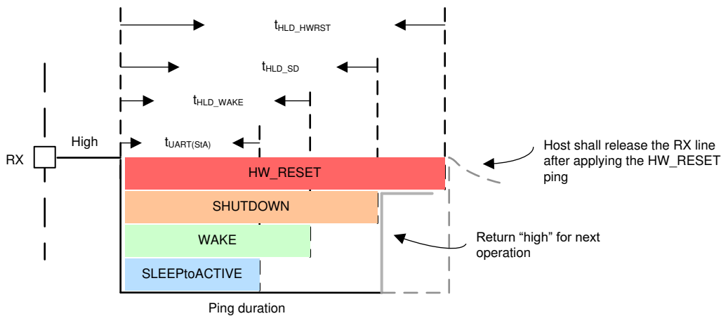
8-62. Communication Pings
