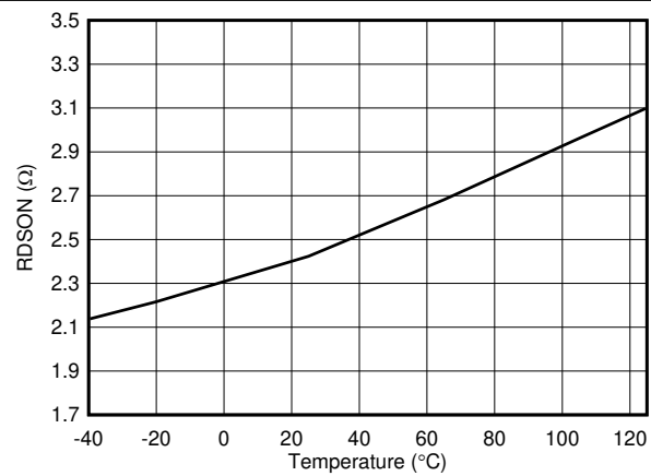
7-3. CBFET RDSON vs Temperature
