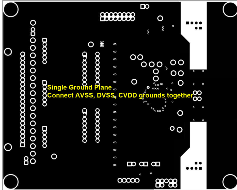
11-6. Thrd Layer with Single Ground Plane
