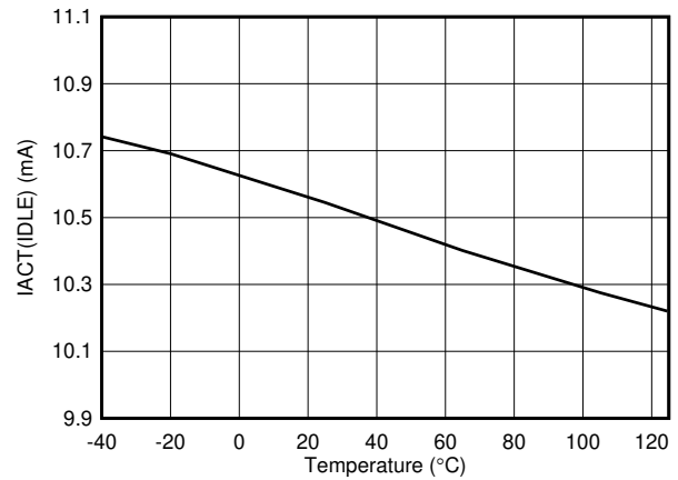
7-2. IACT (IDLE) vs Temperature
