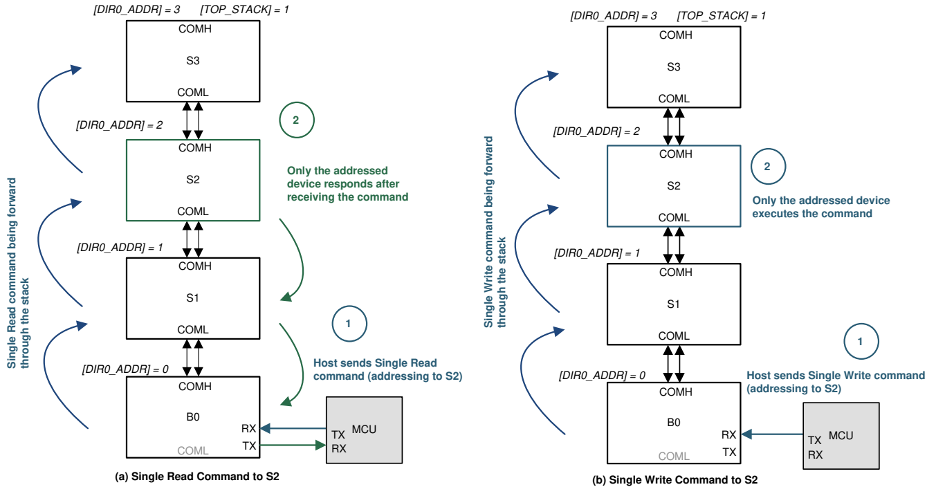
图 8-28. Single Device Read/Write
