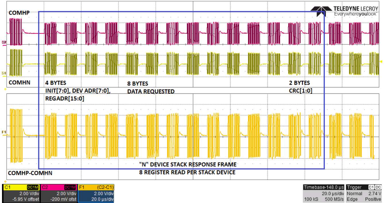
☒ 9-10. Response Frame for 8 Registers Read from Stack Devices
