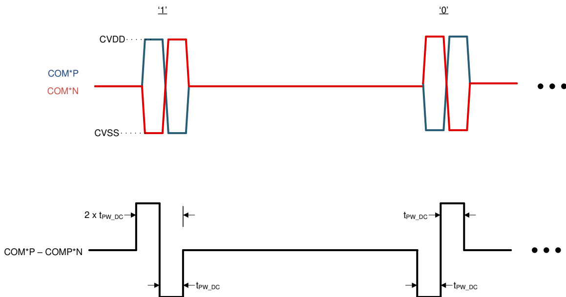
图 8-32. Daisy Chain Bit Definition
