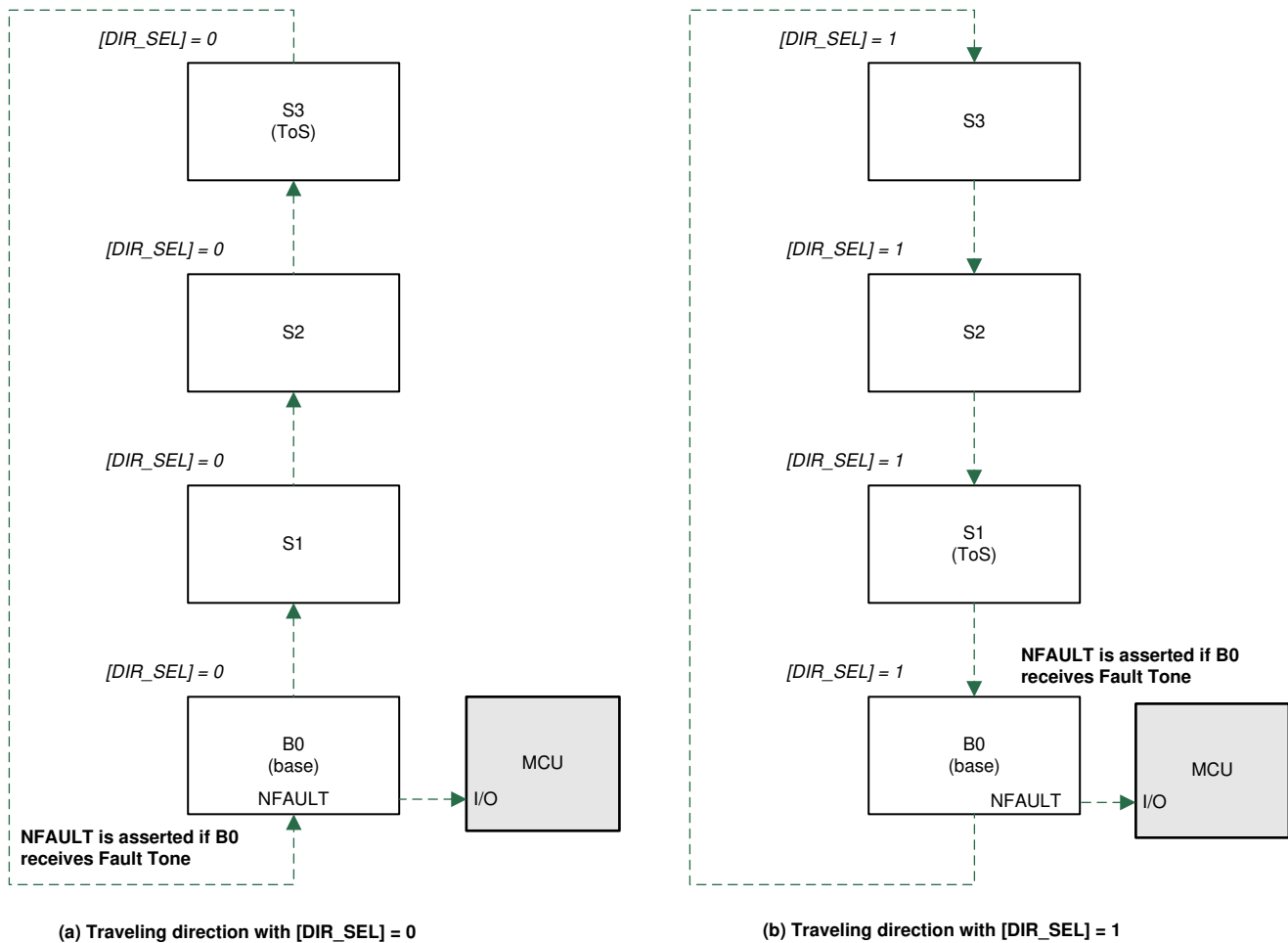
8-44. Heartbeat or Fault Tone Traveling Direction
