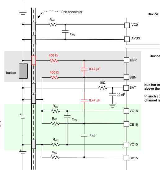
(b) BBP/N connection with bus bar connected above the top of a module
