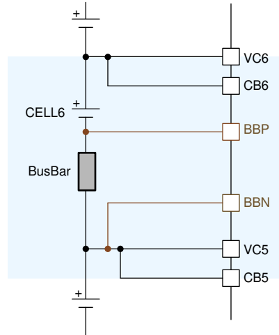
图 8-5. Simplified BBP and BBN Connections
