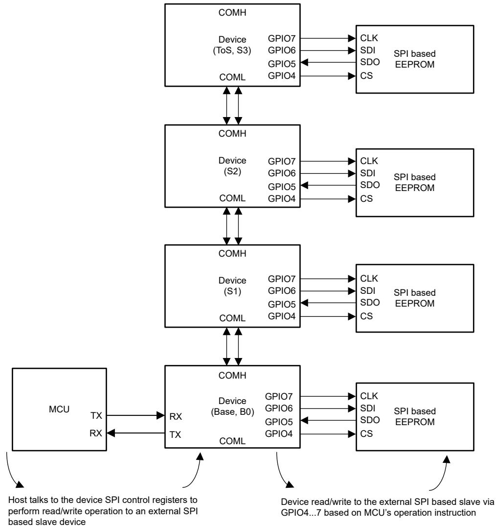
8-39. SPI Controller Stack Configuration
