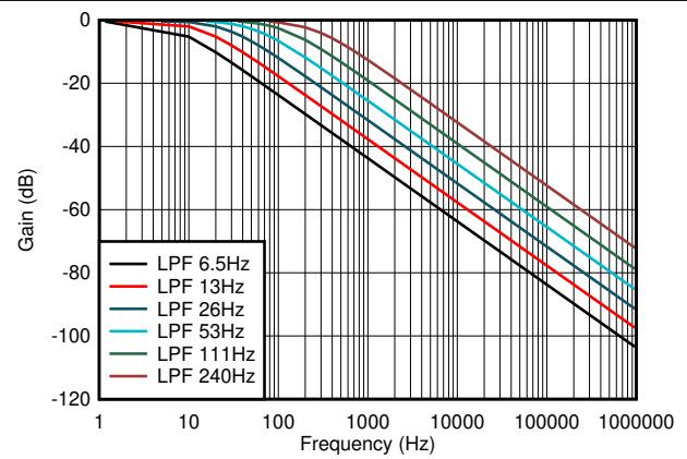
7-4. Digital Low Pass Filter
