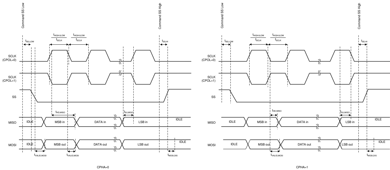
8-41. SPI Controller Timing Diagram
