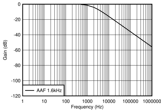
7-5. MAIN ADC Filter
