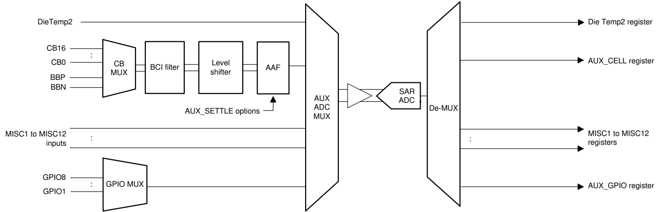
8-8. AUX ADC Measurement Path
