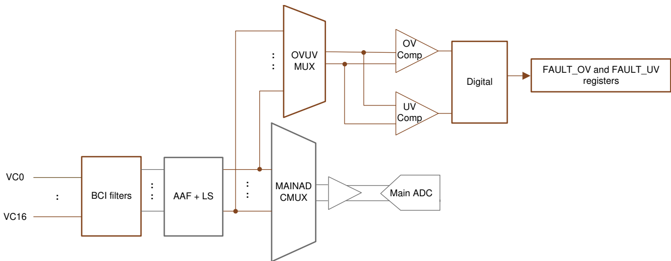
8-19. OV and UV Protectors
