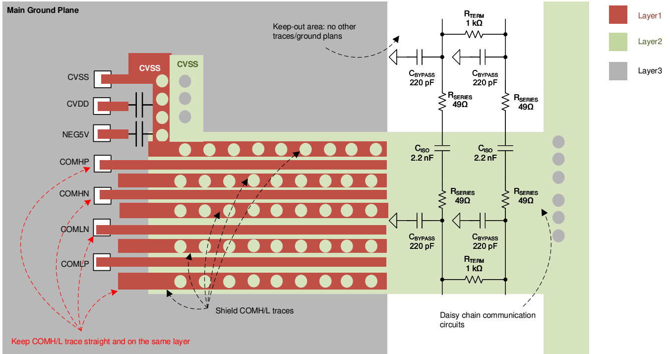
11-3. Daisy Chain Layout Consideration
