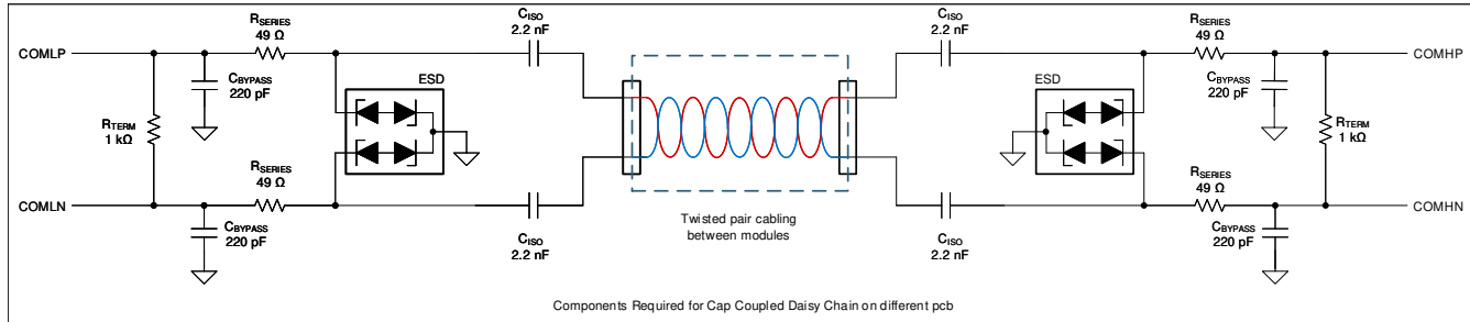
図 9-7. Capacitor Isolation on Different PCB
