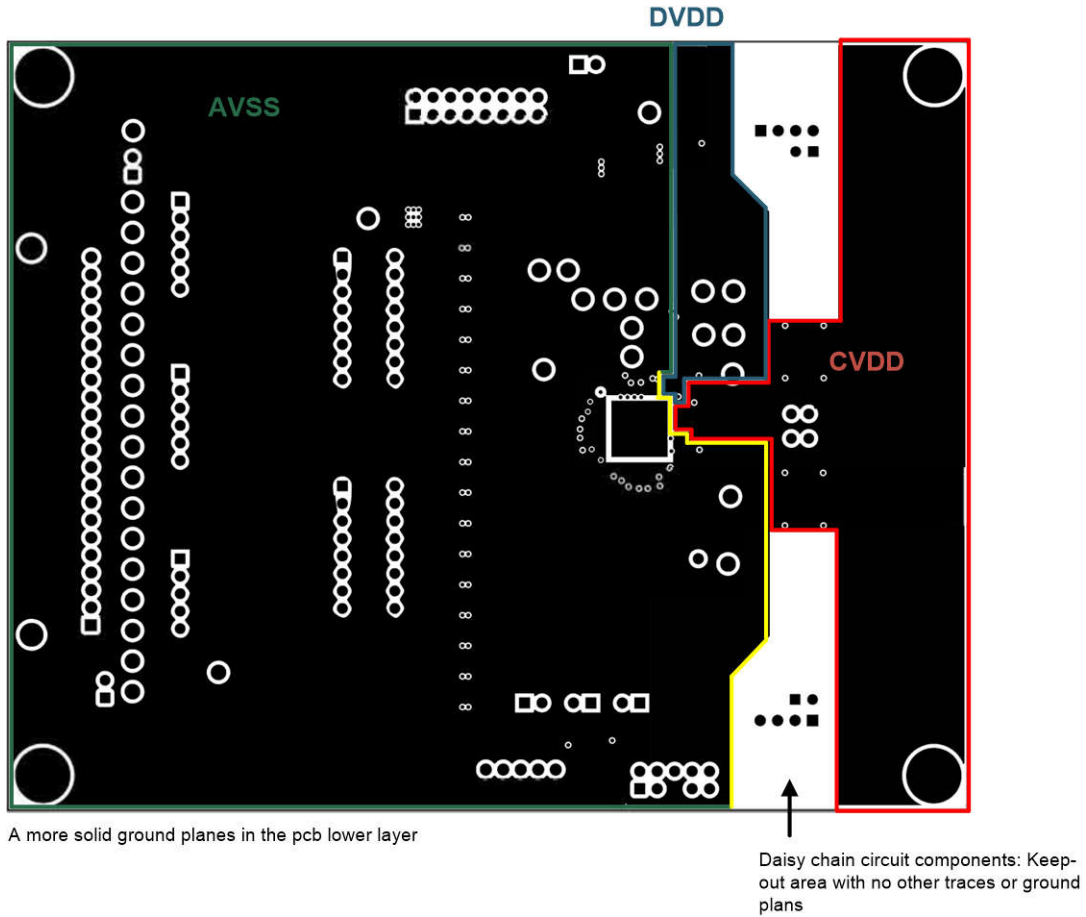
11-5. Second Layer with Solid, Separate Ground Planes
