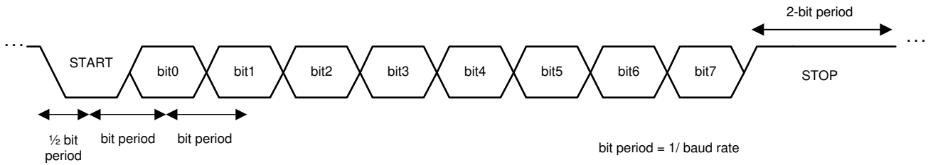
8-24. UART Response Frame with Two STOP Bits
