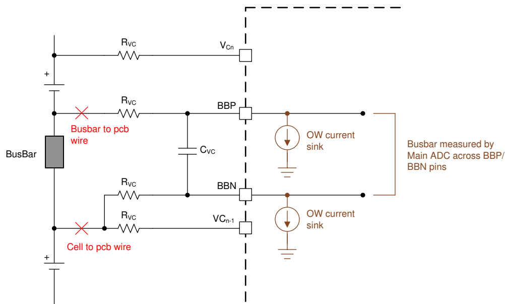
FIG 8-55. Current Sink for BBP/N Open Wire Detection
