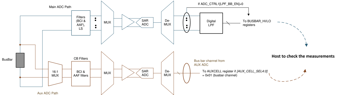
8-54. Bus Bar Through BBP/N Measurement Check
