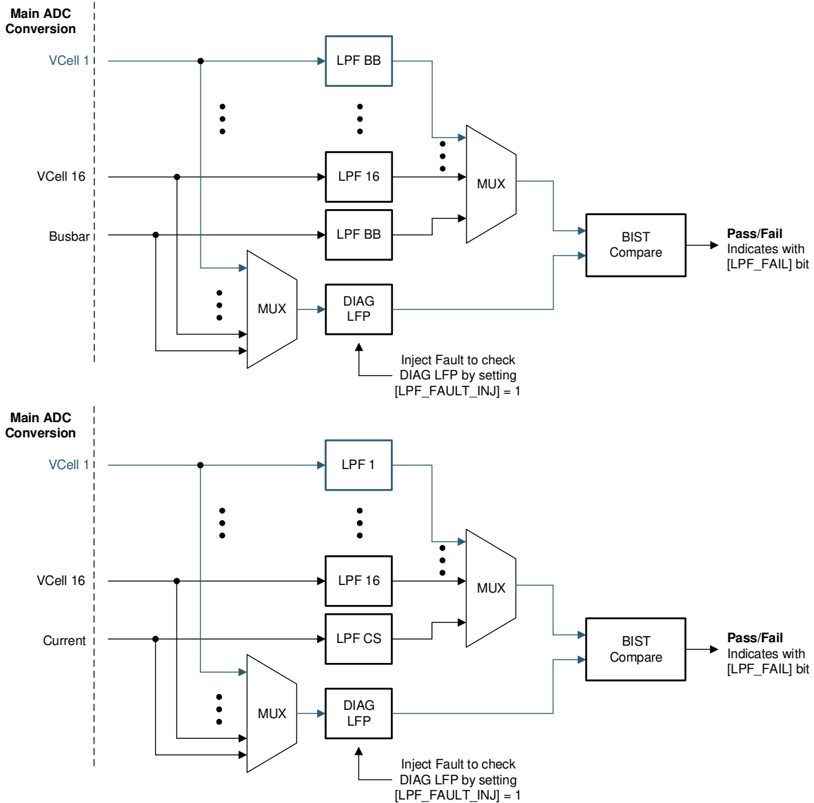
8-48. Post-ADC LPF Diagnostic (Blue Path as Example of Checking LPF1)
