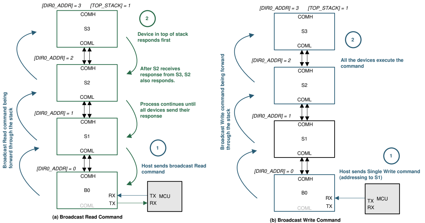
8-30. Broadcast Read/Write
