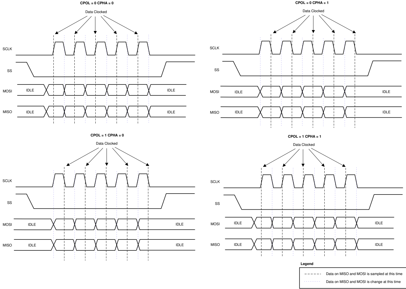
8-40. SPI Controller CPOL and CPHA
