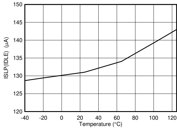
7-1. ISLP (IDLE) vs Temperature
