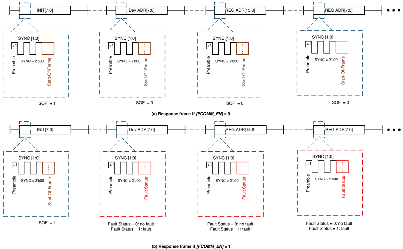
8-42. Embed Fault Status in Communication Response Frame
