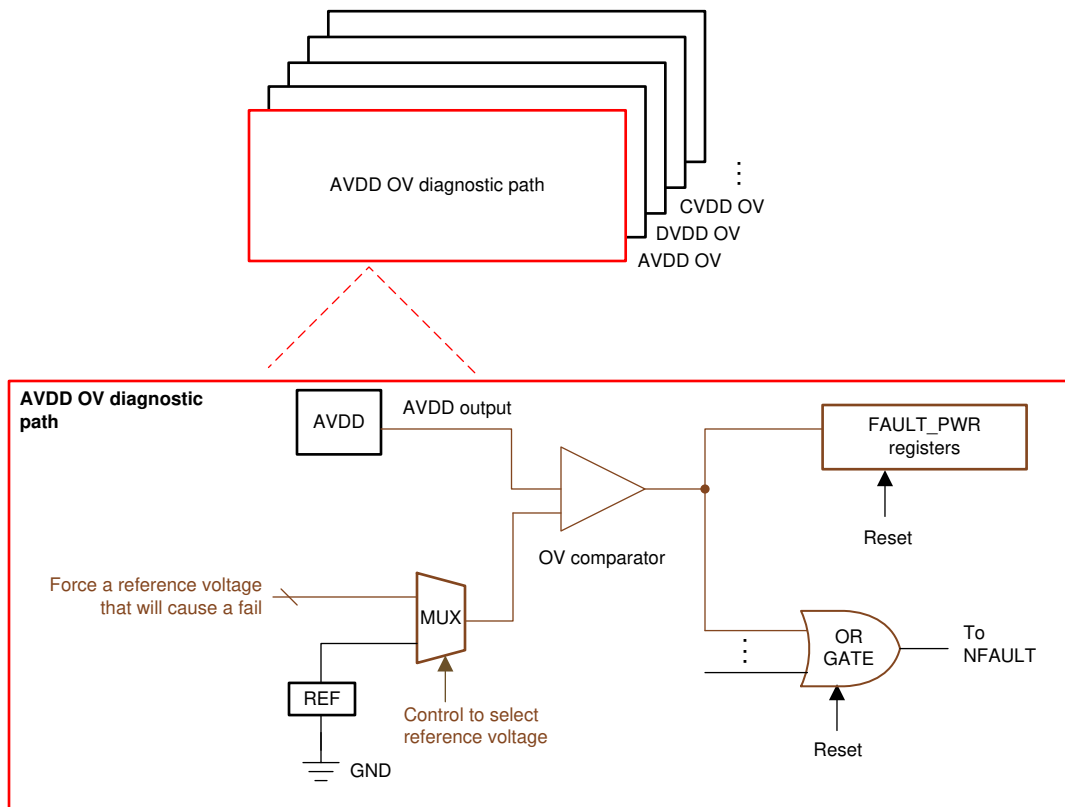
图 8-46. Power Supply BIST
