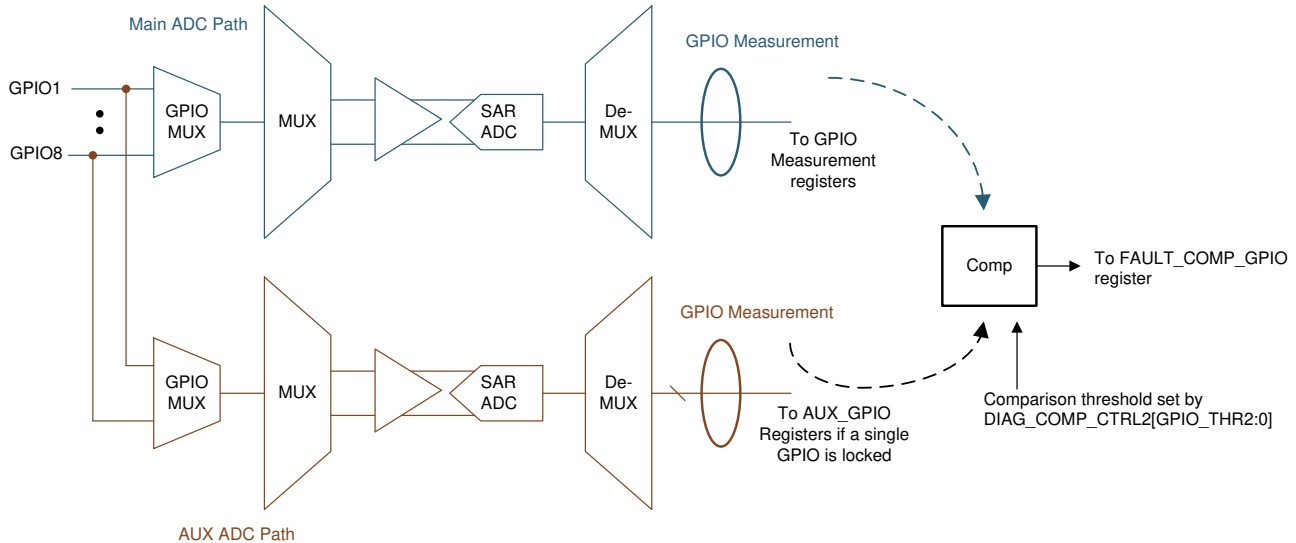
8-49. Thermistor Temperature (GPIO) Measurement Diagnostic
