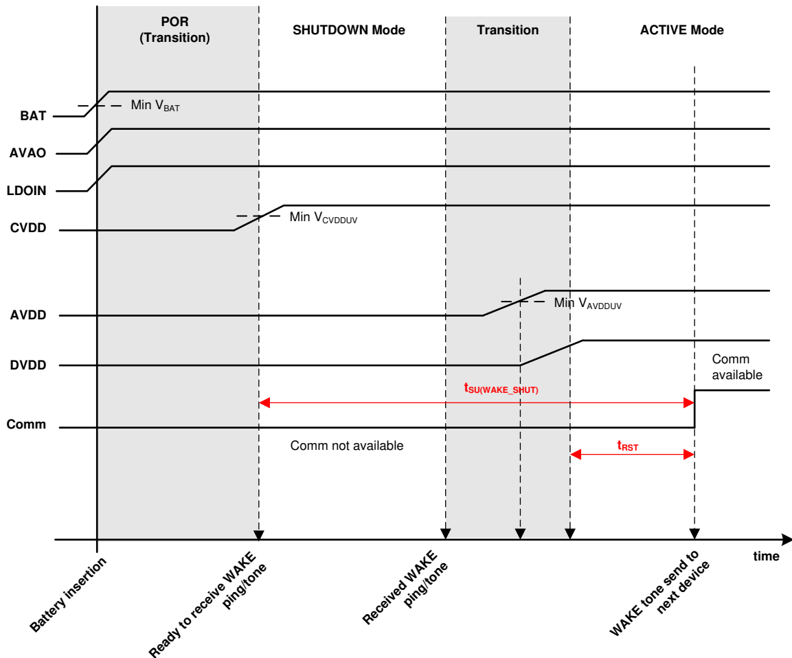
图 8-60. SHUTDOWN to ACTIVE Mode Transition
