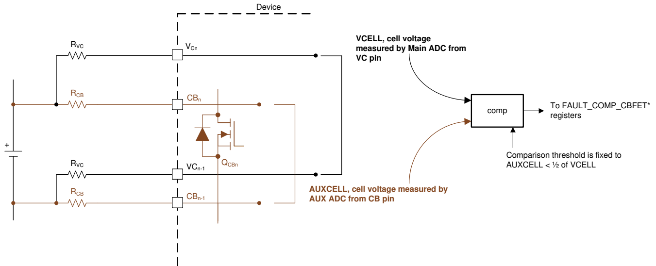
图 8-50. Cell Balancing FET Diagnostic
