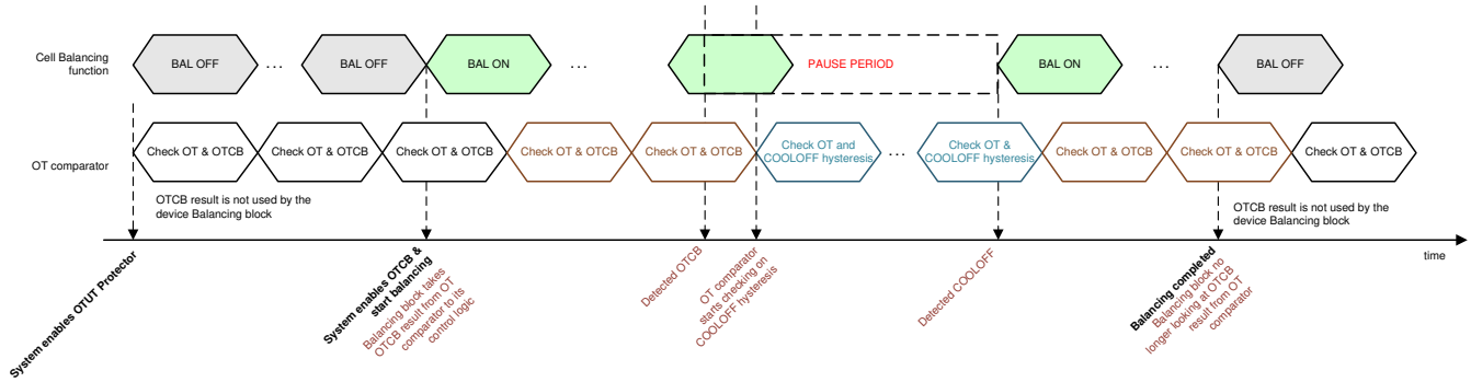
8-17. Cell Balancing Pause and Resume by OTCB Detection
