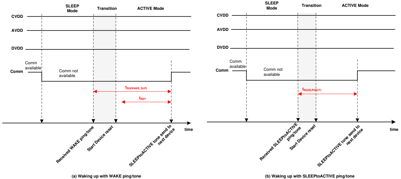
8-61. SLEEP to ACTIVE Mode Transition
