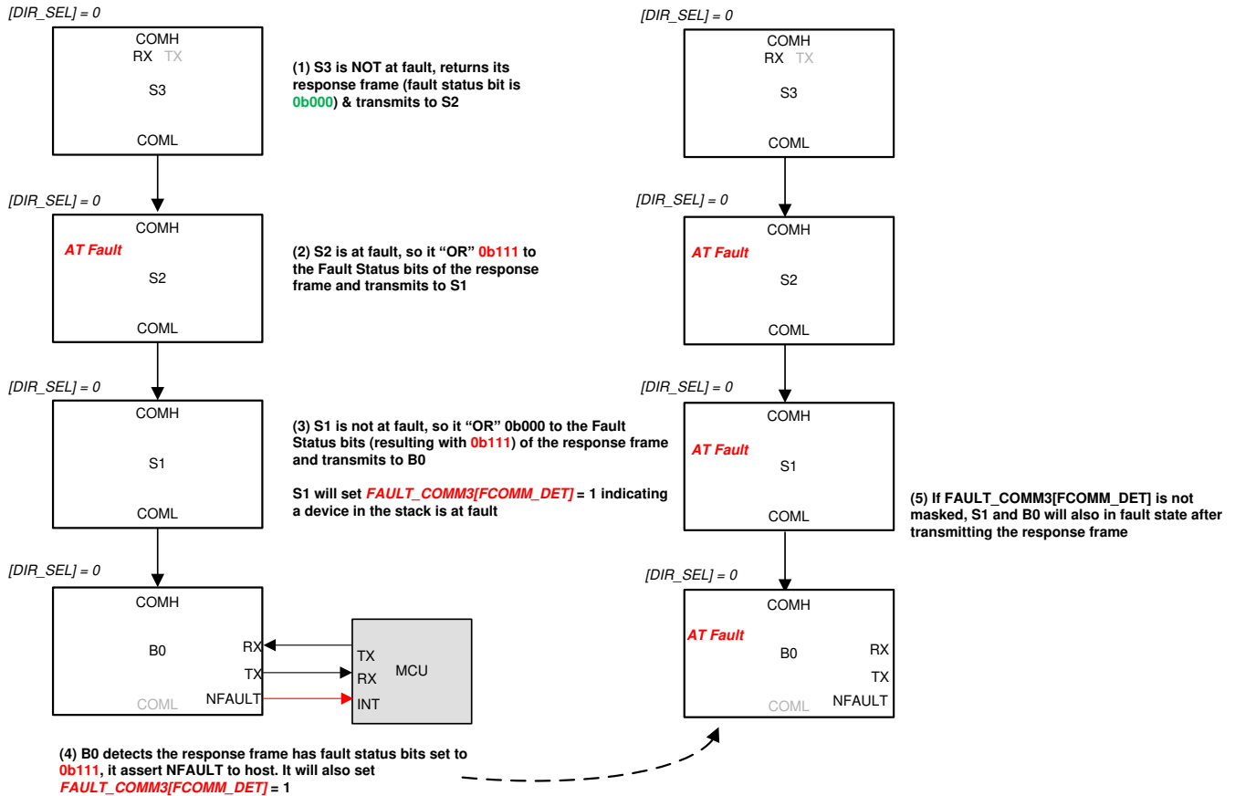
8-43. Transfer Fault Status in ACTIVE Mode (Respond to a Single Device Read)
