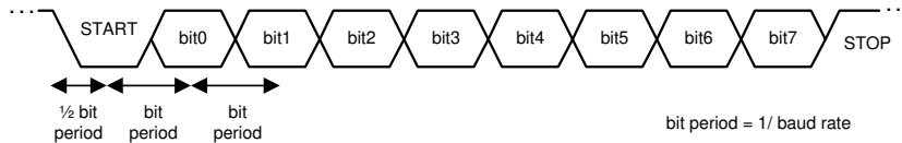
8-23. UART Communication to Host
