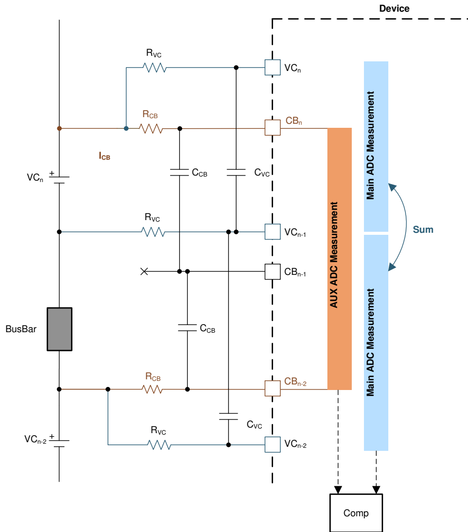
8-58. Cell Measurement Check with Bus Bar Connected to Individual VC Channel
