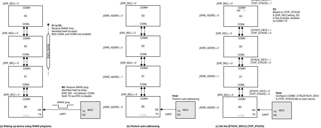
8-35. Configure Device for Communication
