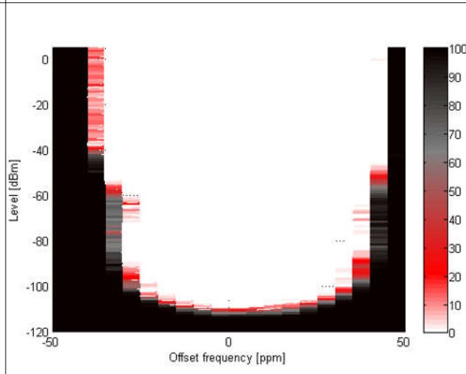
8-17. 802.15.4, 50 kbps, \pm 25 kHz deviation, 2-GFSK, 100 kHz RX Bandwidth
