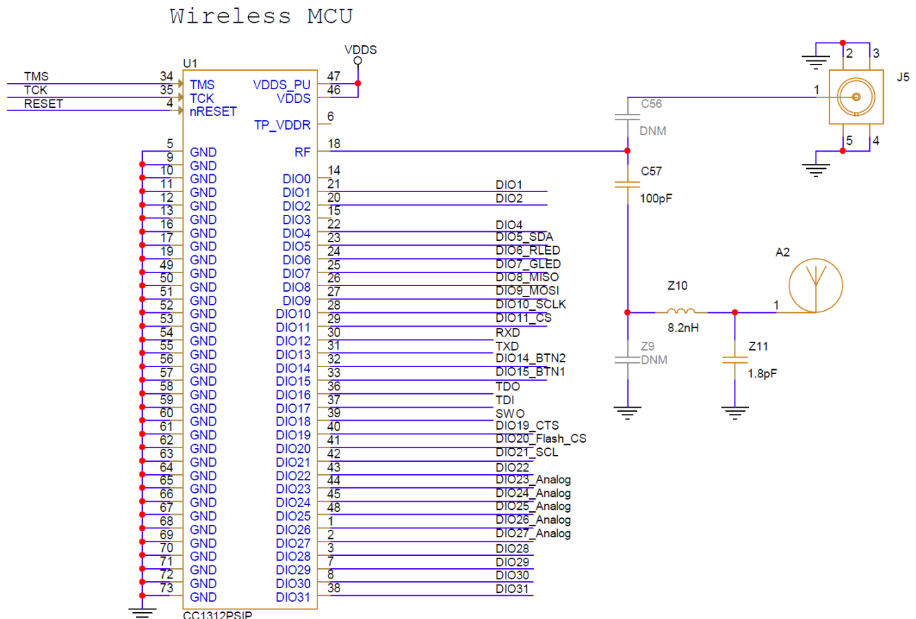
☒ 10-1. CC1312PSIP Typical Application Schematic with integrated antenna on LP-EM-CC1312PSIP
