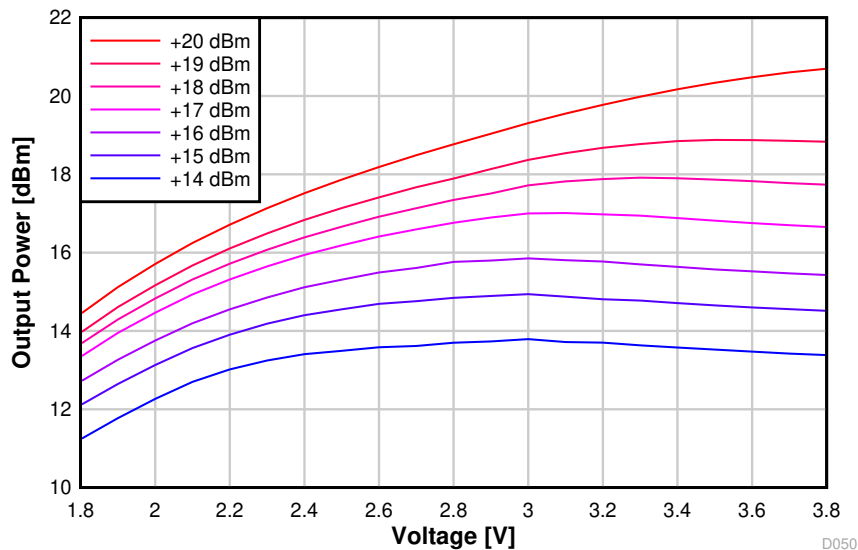
8-49. Output Power vs. Supply Voltage (VDD5) (BLE 1 Mbps, 2.44 GHz, +20 dBm PA)
