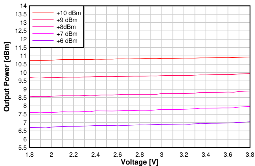
8-50. Output Power vs. Supply Voltage (VDD5) (2.44 GHz, +10 dBm PA)
