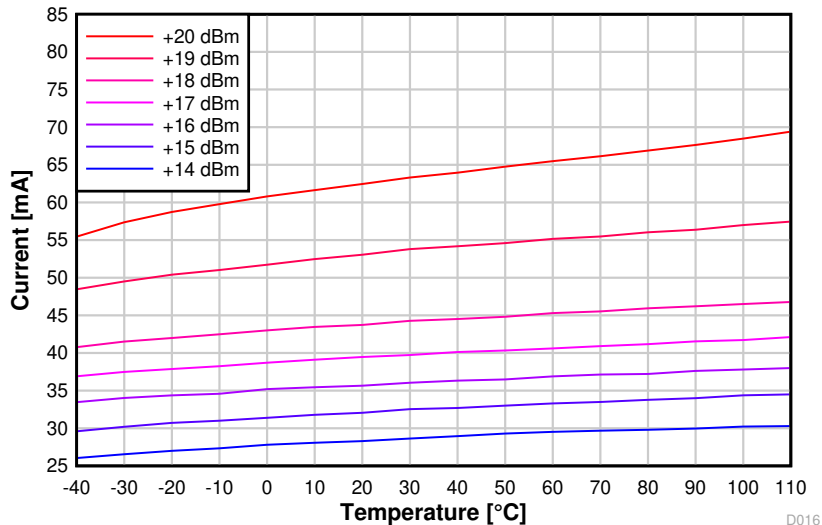
8-14. TX Current vs. Temperature (50 kbps, 915 MHz, VDD5 = 3.3 V)
