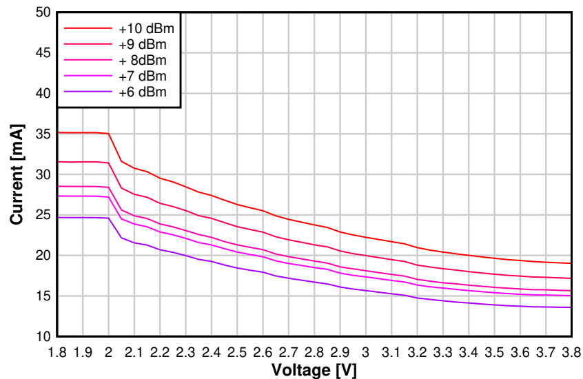
8-22. TX Current vs. Supply Voltage (VDD5) (250 kbps, 2.44 GHz, +10 dBm PA)
