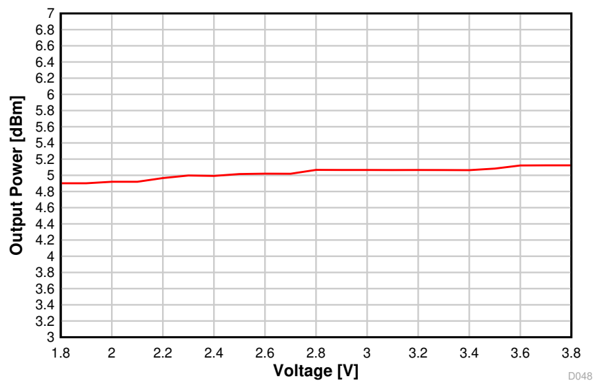
8-38. Output Power vs. Supply Voltage (VDD5) (BLE 1 Mbps, 2.44 GHz, +5 dBm)
