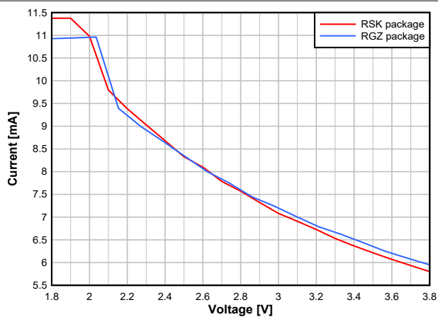
8-13. TX Current vs. Supply Voltage (VDD5) (BLE 1 Mbps, 2.44 GHz, 0 dBm)
