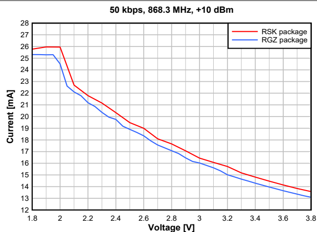
8-12. TX Current vs. Supply Voltage (VDD5) (50 kbps, 868.3 MHz)
