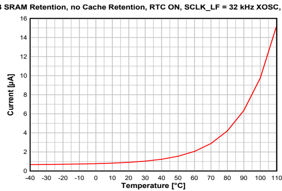
8-5. Standby Mode (MCU) Current vs. Temperature (VDD5 = 3.6 V)
