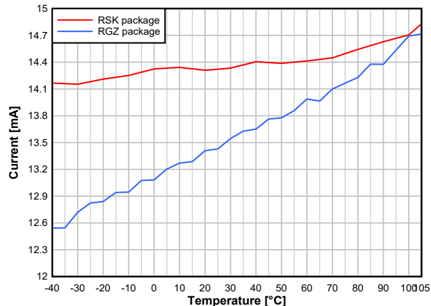
8-10. TX Current vs. Temperature (50 kbps, 868.3 MHz, +10 dBm, VDD5 = 3.6 V)
