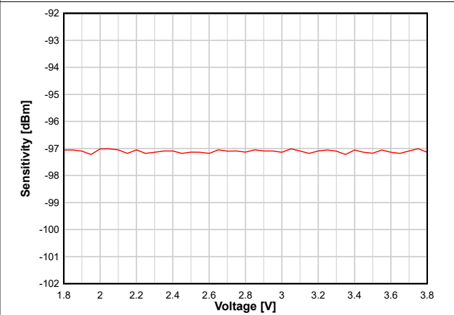
8-14. Sensitivity vs. Supply Voltage (VDD5) (BLE 1 Mbps, 2.44 GHz, DCDC Off)
