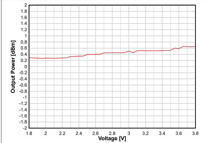
8-18. Output Power vs. Supply Voltage (VDD5) (BLE 1 Mbps, 2.44 GHz, 0dBm)
