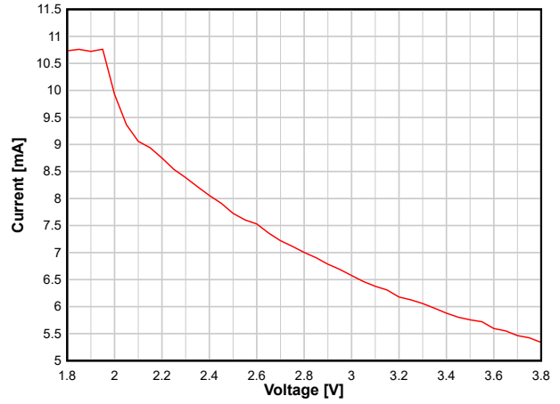
8-8. RX Current versus Supply Voltage (VDDS) (BLE 1 Mbps, 2.44 GHz)
