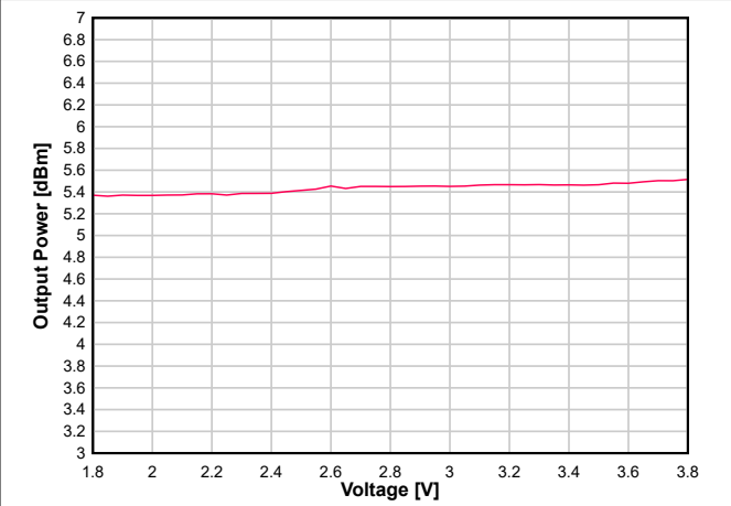
8-19. Output Power vs. Supply Voltage (VDD5) (BLE 1 Mbps, 2.44 GHz, +5dBm)
