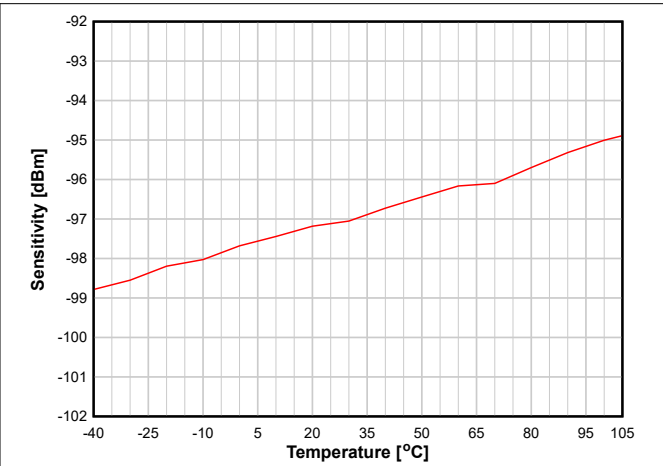
8-12. Sensitivity vs. Temperature (BLE 1 Mbps, 2.44 GHz)
