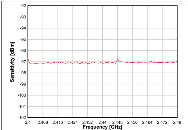
8-11. Sensitivity versus Frequency (BLE 1 Mbps, 2.44 GHz)
