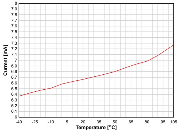
8-7. RX Current versus Temperature (BLE 1 Mbps, 2.44 GHz)
