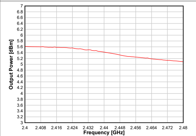
8-21. Output Power vs. Frequency (BLE 1 Mbps, +5dBm)
