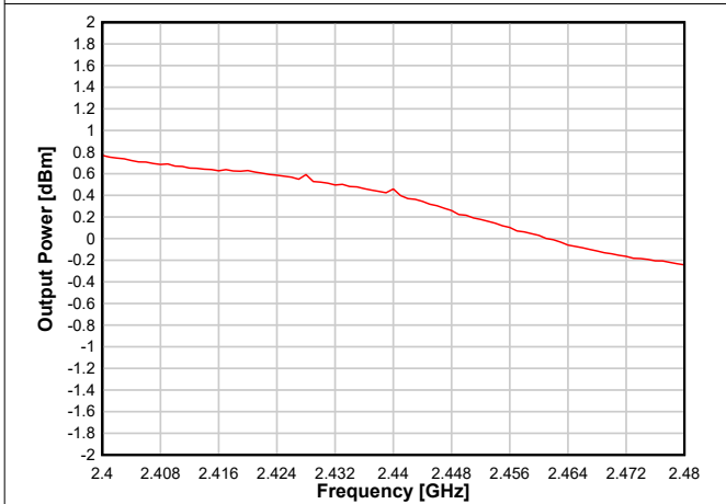
8-20. Output Power vs. Frequency (BLE 1 Mbps, 0dBm)
