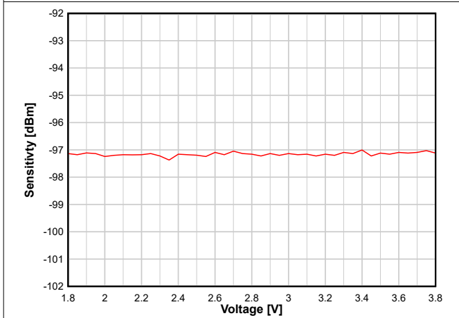
8-13. Sensitivity vs. Supply Voltage (VDD5) (BLE 1 Mbps, 2.44 GHz)
