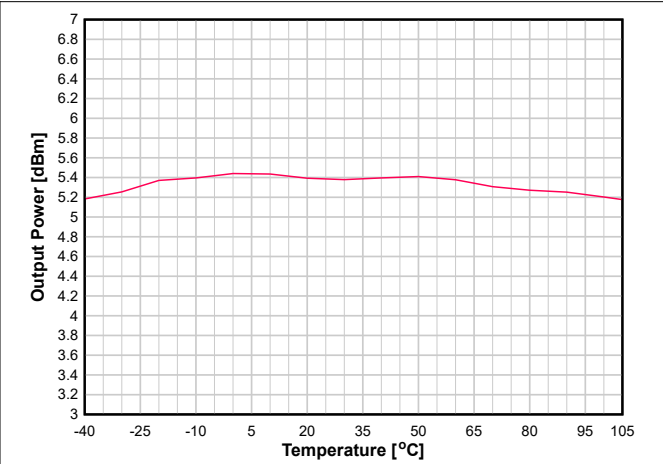
8-17. Output Power vs. Temperature (BLE 1 Mbps, 2.44 GHz, +5dBm)
