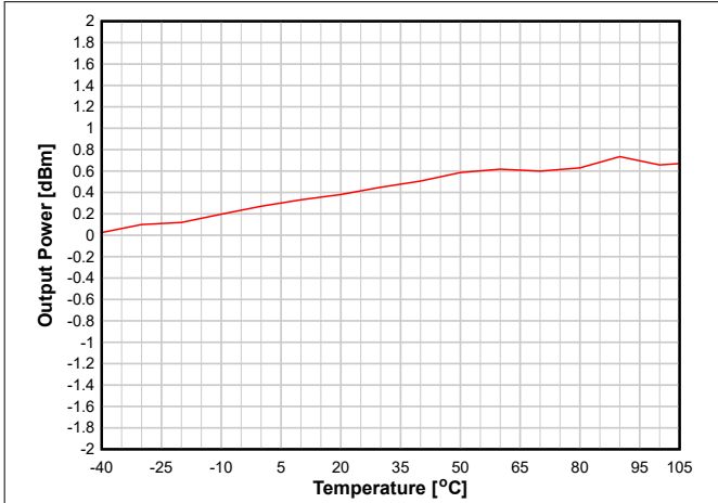
8-16. Output Power vs. Temperature (BLE 1 Mbps, 2.44 GHz, 0dBm)
