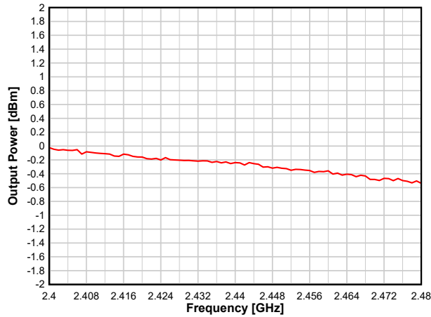
8-27. Output Power vs. Frequency (BLE 1 Mbps, 0 dBm)
