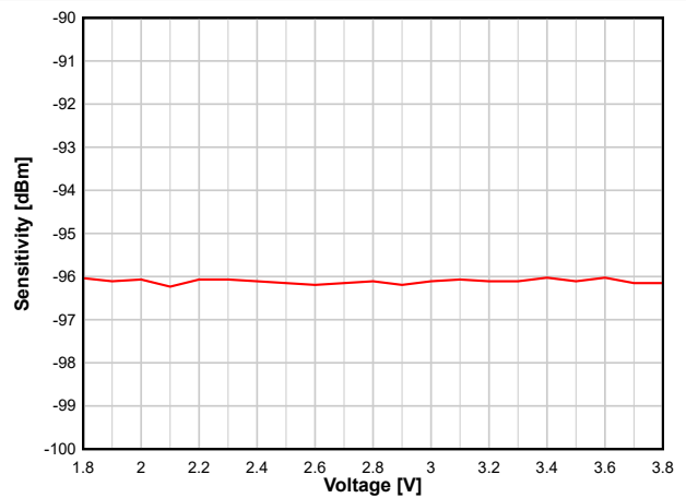
8-19. Sensitivity vs. Supply Voltage (VDD5) (BLE 1 Mbps, 2.44 GHz, DCDC Off)
