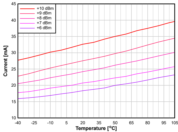
8-10. TX Current vs. Temperature (BLE 1 Mbps, 2.44 GHz, +10 dBm)
