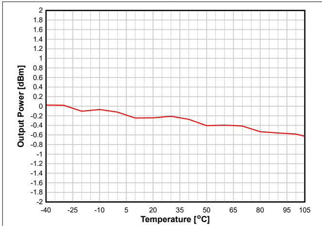
8-21. Output Power vs. Temperature (BLE 1 Mbps, 2.44 GHz, 0 dBm)
