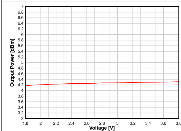
8-25. Output Power vs. Supply Voltage (VDD5) (BLE 1 Mbps, 2.44 GHz, +5 dBm)
