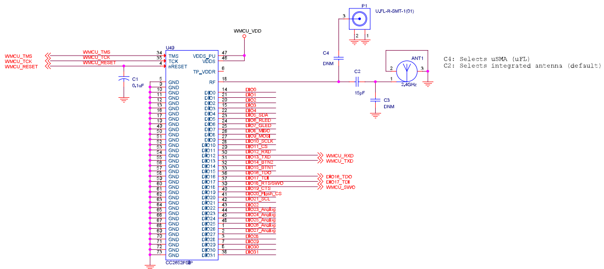
☒ 10-1. CC2652PSIP Typical Application Schematic
