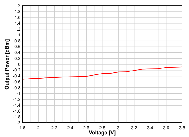
8-24. Output Power vs. Supply Voltage (VDD5) (BLE 1 Mbps, 2.44 GHz, 0 dBm)
