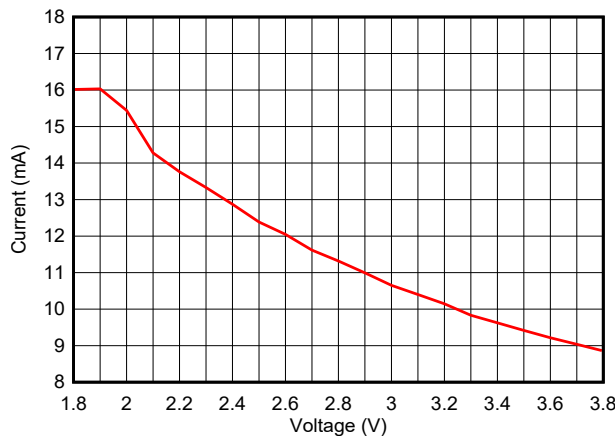
8-12. TX Current vs. Supply Voltage (VDD5) (BLE 1 Mbps, 2.44 GHz, +5 dBm)
