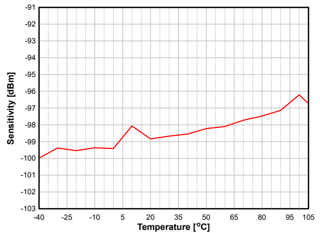
8-17. Sensitivity vs. Temperature (250 kbps, 2.44 GHz)
