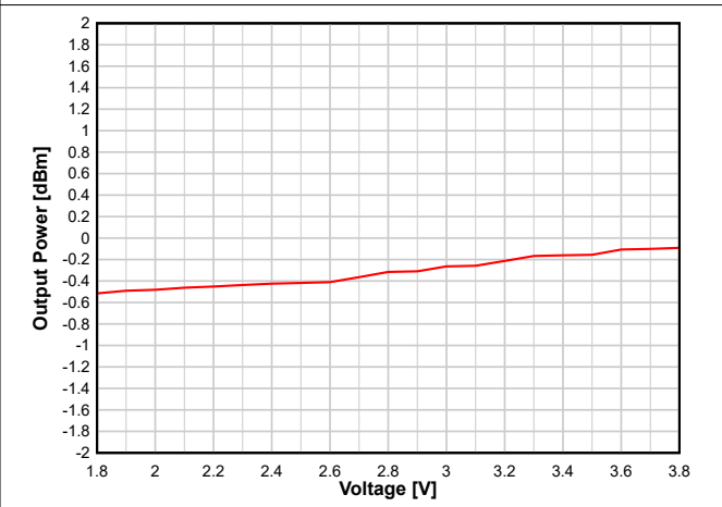
8-24. Output Power vs. Supply Voltage (VDD5) (BLE 1 Mbps, 2.44 GHz, 0 dBm)
