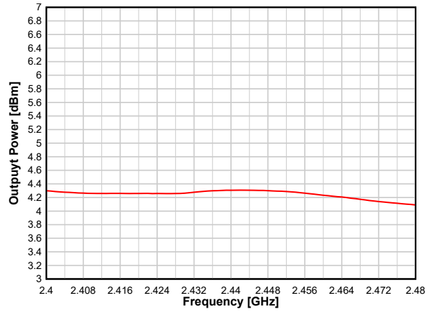
8-28. Output Power vs. Frequency (BLE 1 Mbps, +5 dBm)
