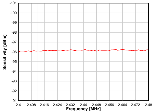
8-14. Sensitivity vs. Frequency (BLE 1 Mbps)
