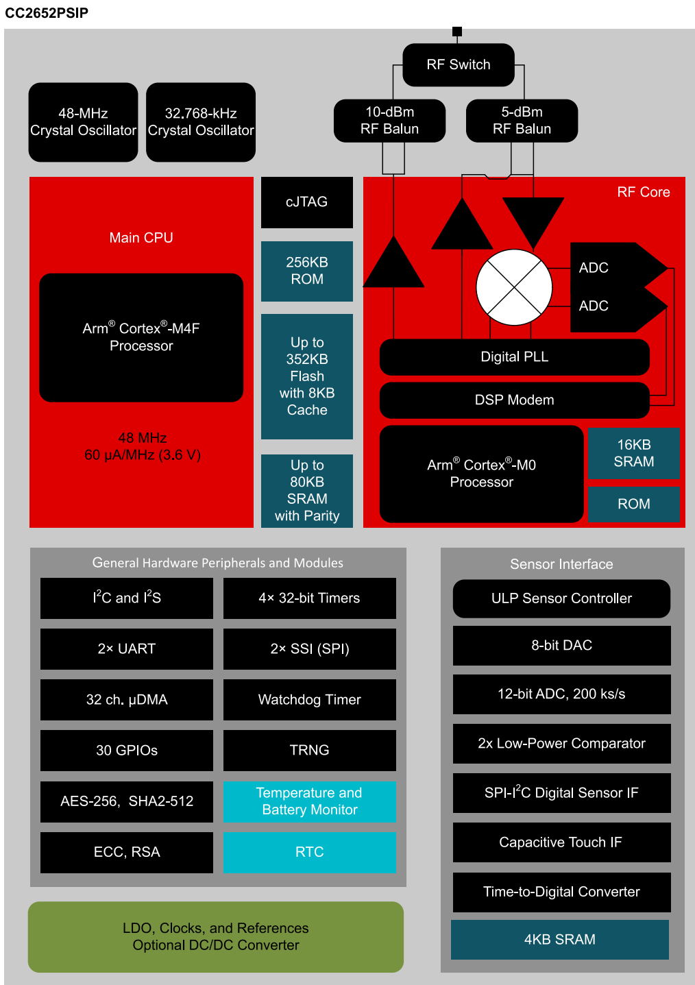
4-2. CC2652PSIP Hardware Overview
