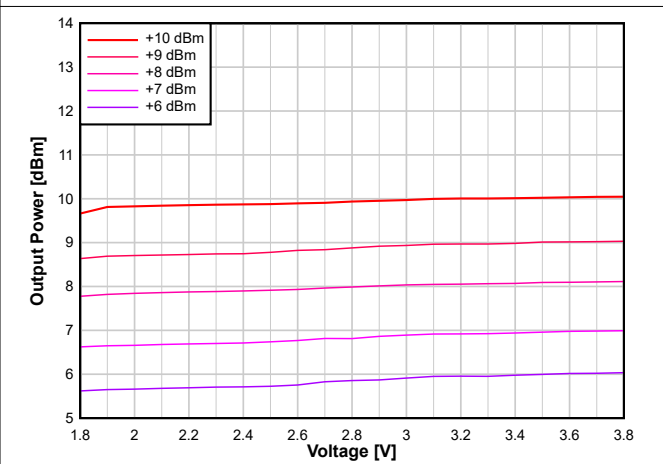
8-26. Output Power vs. Supply Voltage (VDD5) (2.44 GHz, +10 dBm PA)
