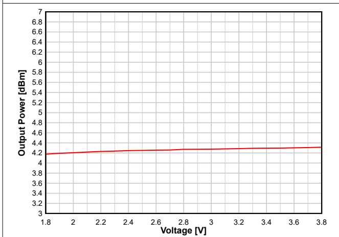
8-25. Output Power vs. Supply Voltage (VDD5) (BLE 1 Mbps, 2.44 GHz, +5 dBm)
