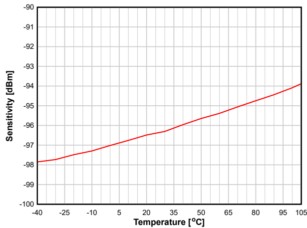
8-16. Sensitivity vs. Temperature (BLE 1 Mbps, 2.44 GHz)
