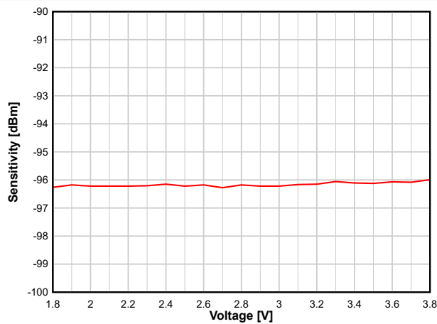
8-18. Sensitivity vs. Supply Voltage (VDD5) (BLE 1 Mbps, 2.44 GHz)
