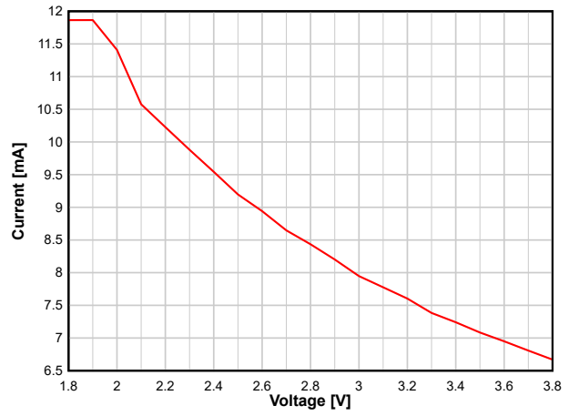
8-11. TX Current vs. Supply Voltage (VDD5) (BLE 1 Mbps, 2.44 GHz, 0 dBm)
