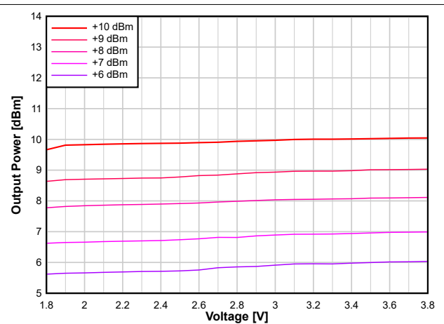
8-26. Output Power vs. Supply Voltage (VDD5) (2.44 GHz, +10 dBm PA)
