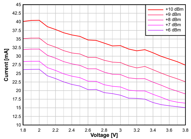
8-13. TX Current vs. Supply Voltage (VDD5) (BLE 1 Mbps, 2.44 GHz, +10 dBm PA)
