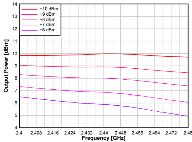
8-29. Output Power vs. Frequency (BLE 1 Mbps, +10 dBm PA)
