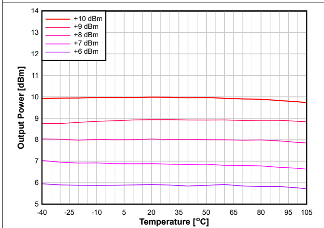
8-23. Output Power vs. Temperature (BLE 1 Mbps, 2.44 GHz, +10 dBm)
