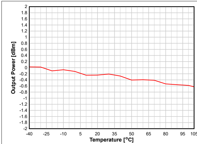
8-21. Output Power vs. Temperature (BLE 1 Mbps, 2.44 GHz, 0 dBm)
