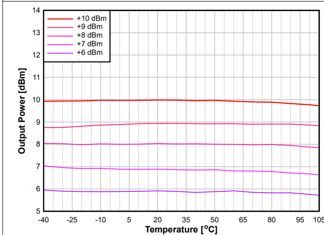
8-23. Output Power vs. Temperature (BLE 1 Mbps, 2.44 GHz, +10 dBm)
