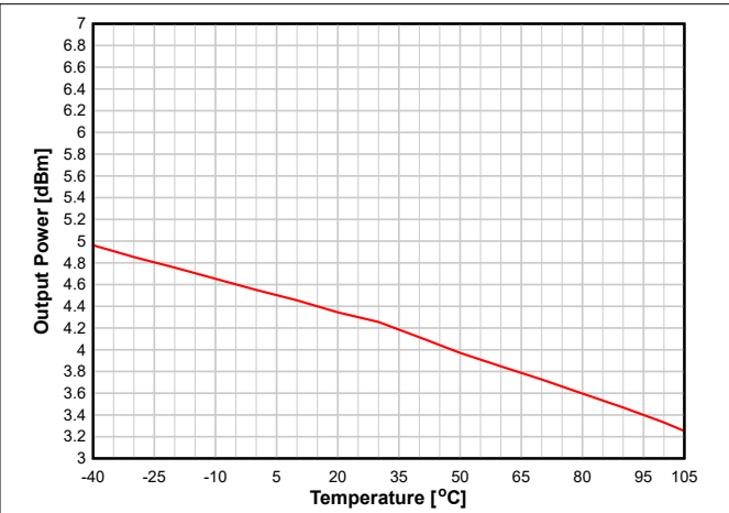
8-22. Output Power vs. Temperature (BLE 1 Mbps, 2.44 GHz, +5 dBm)
