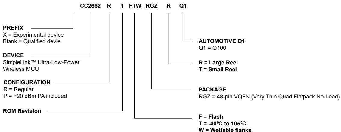
❏ 11-1. Device Nomenclature
