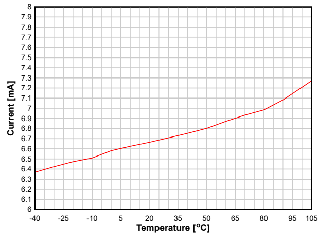
8-7. RX Current versus Temperature (WBMS, 2.44 GHz)
