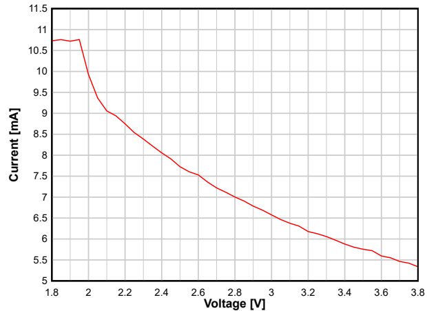
8-8. RX Current versus Supply Voltage (VDD5) (WBMS, 2.44 GHz)
