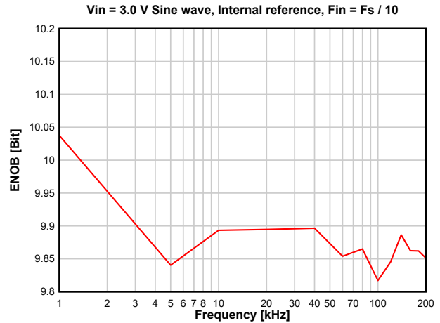
8-22. ENOB versus Sampling Frequency
