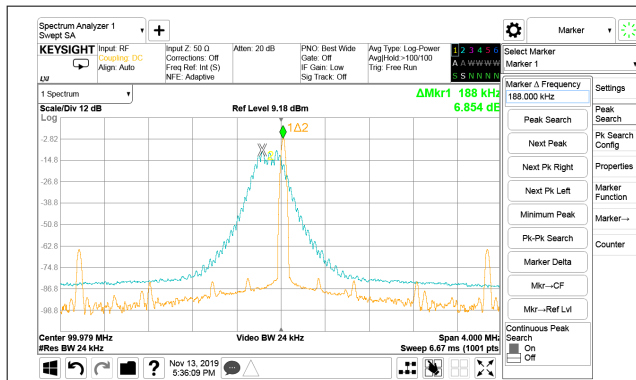
9-4. 100 MHz With - 0.25% Down Spread With and Without Trace
