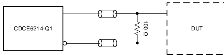
8-12. LVDS Output - DC-Coupled. Place 100Ω close to the DUT
