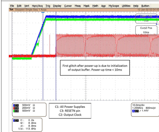
7-7. All Power Supply = 1.8 V, VDD Ramp Time = 10 ms
