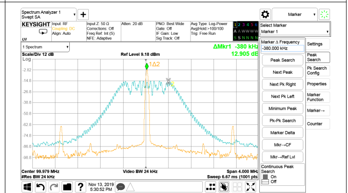
9-7. 100 MHz With +/- 0.5% Center Spread With and Without Trace
