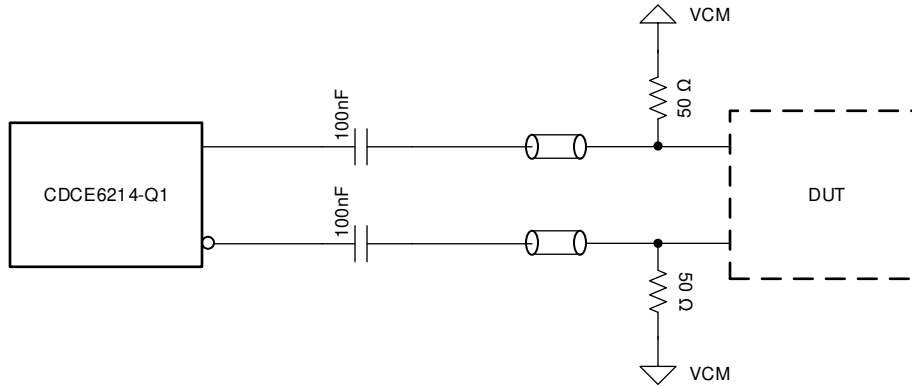
8-13. LVDS Output - AC-Coupled
