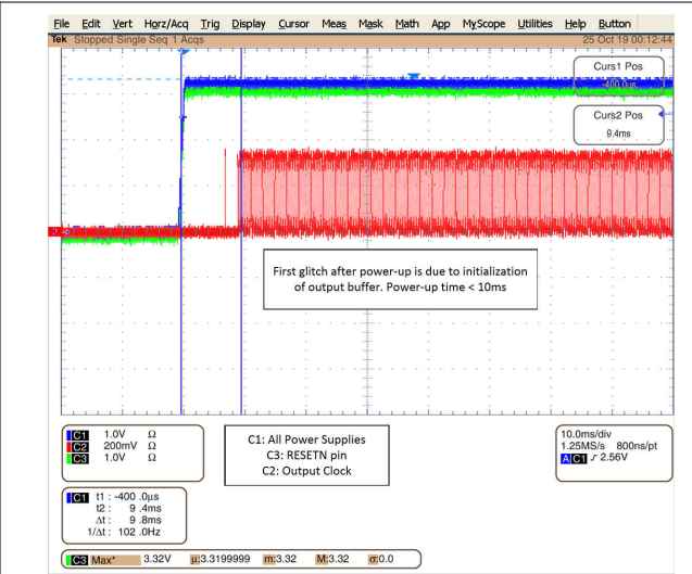
7-6. All Power Supply = 3.3 V, VDD Ramp Time = 1 ms
