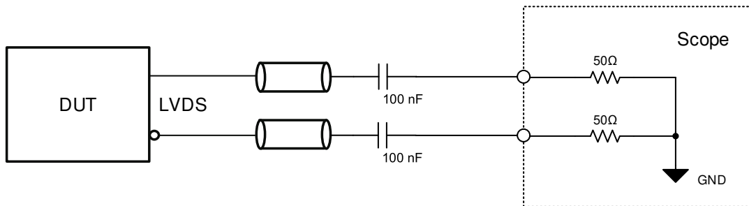
8-3. LVDS Output Test Configuration, AC-Coupled
