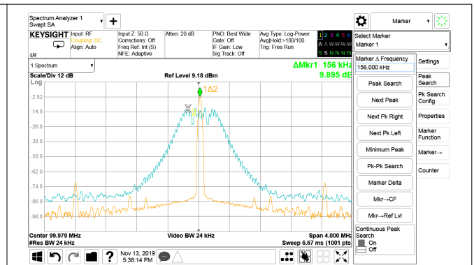
9-5. 100 MHz With +/- 0.25% Center Spread With and Without Trace
