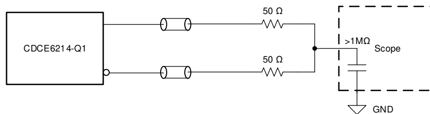
8-5. LVDS Common Mode Voltage, DC-Coupled
