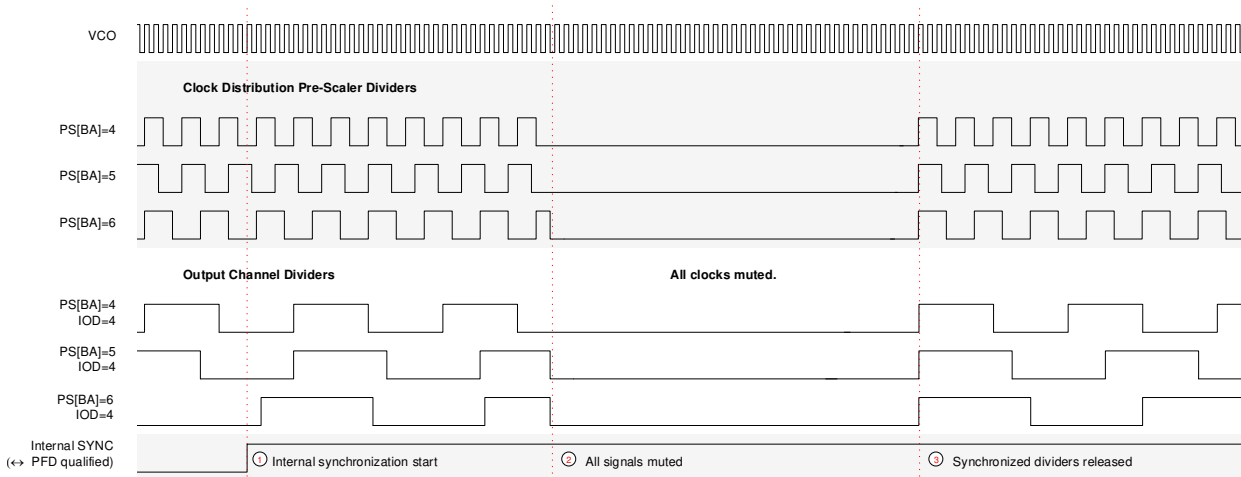
9-9. Output Divider Synchronization
