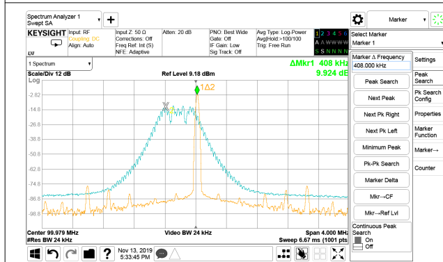
9-6. 100 MHz With - 0.5% Down Spread With and Without Trace
