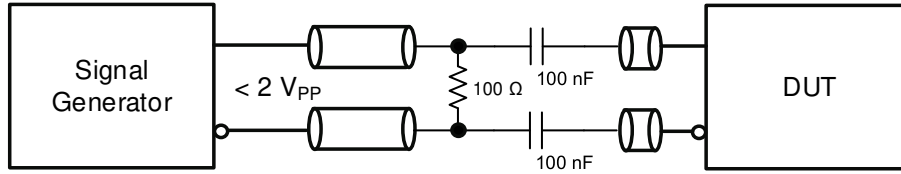
8-10. Differential Input to Reference
