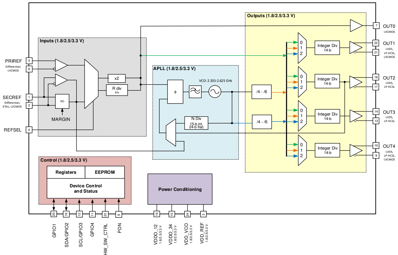
9-1. CDCE6214-Q1 Clock Generator With 2 Inputs, 1 Fractional-N PLL, and 4 Outputs
