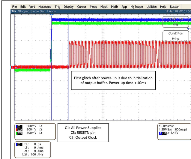
7-5. All Power Supply = 1.8 V, VDD Ramp Time = 1 ms
