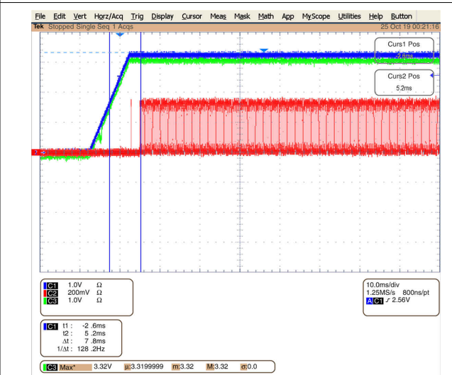
7-8. All Power Supply = 3.3 V, VDD Ramp Time = 10 ms
