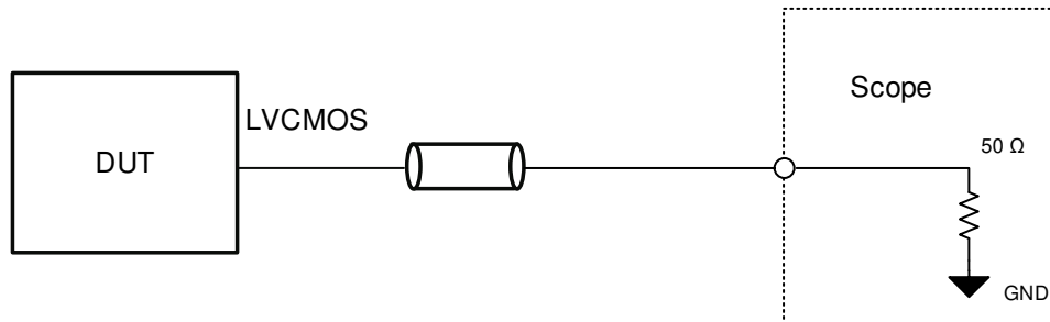
8-2. LVC MOS Output Test Configuration
