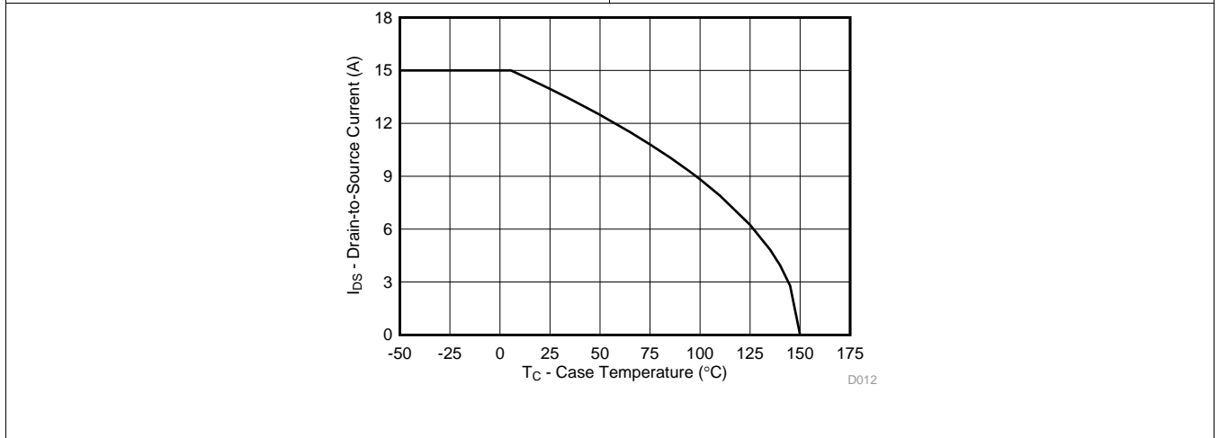
Figure 12. Maximum Drain Current vs Temperature
