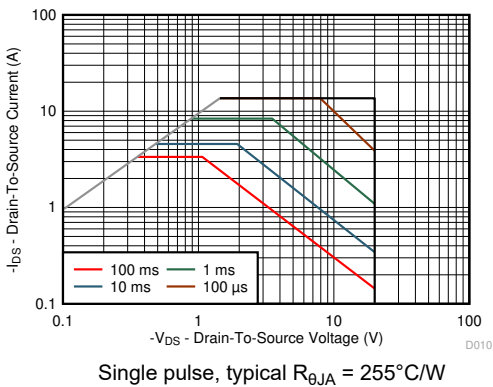
4-10. Maximum Safe Operating Area
