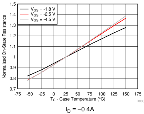
4-8. Normalized On-State Resistance vs Temperature
