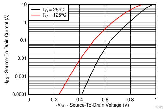
4-9. Typical Diode Forward Voltage
