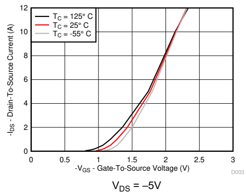
4-3. Transfer Characteristics
