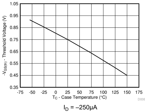
4-6. Threshold Voltage vs Temperature
