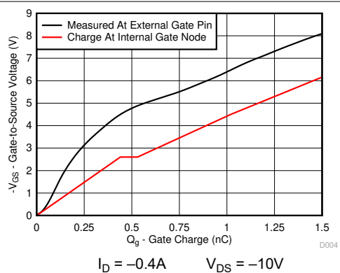
4-4. Gate Charge
