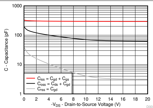
4-5. Capacitance
