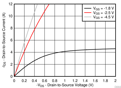
4-2. Saturation Characteristics
