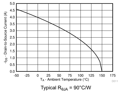
4-11. Maximum Drain Current vs Temperature
