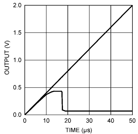
Power-On Reset
