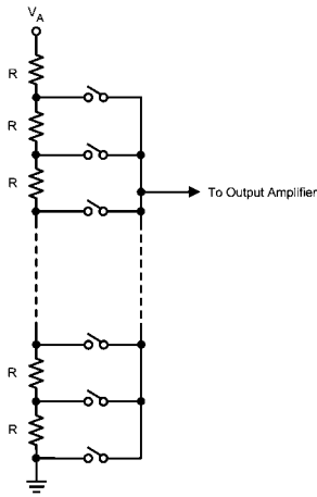
FIGURE 3. DAC Resistor String
