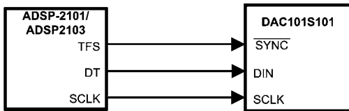
FIGURE 5. ADSP-2101/2103 Interface
