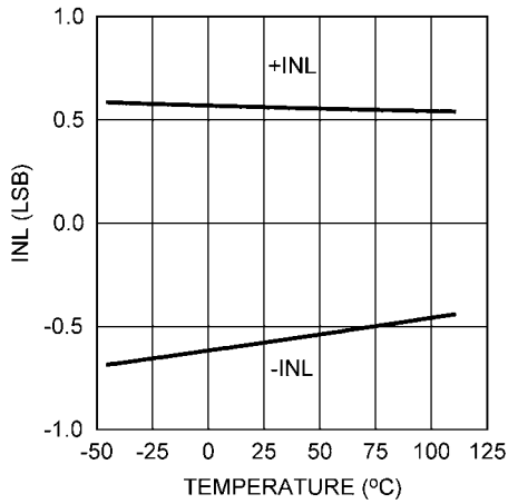
3V INL vs. Temperature
