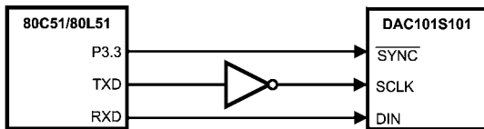
FIGURE 6. 80C51/80L51 Interface
