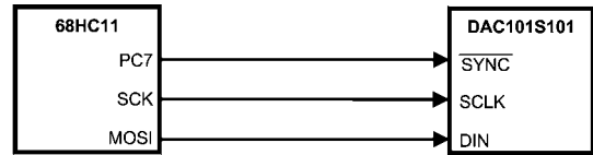
FIGURE 7. 68HC11 Interface
