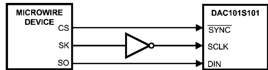
FIGURE 8. Microwire Interface
