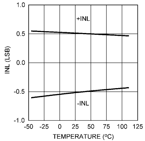
5V INL vs. Temperature
