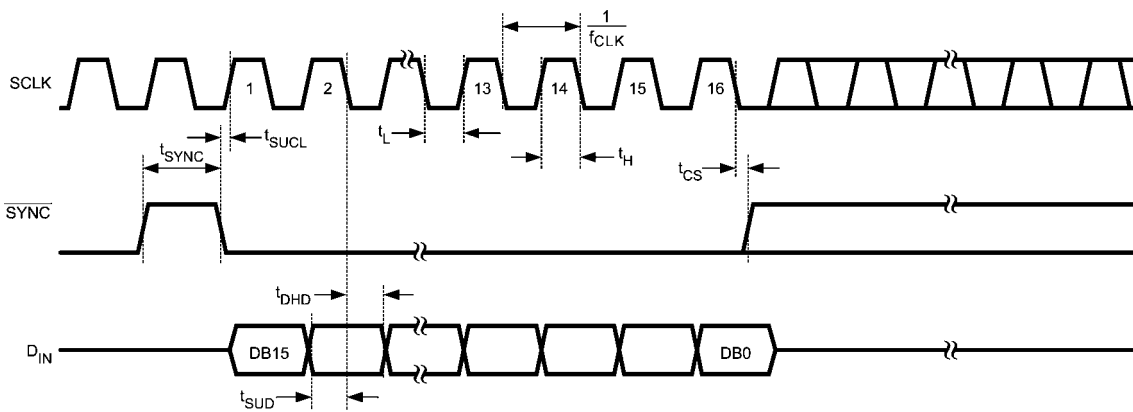
FIGURE 2. DAC101S101 Timing
