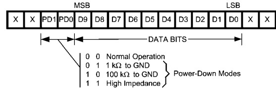
FIGURE 4. Input Register Contents
