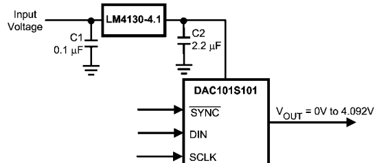
FIGURE 9. The LM4130 as a power supply
