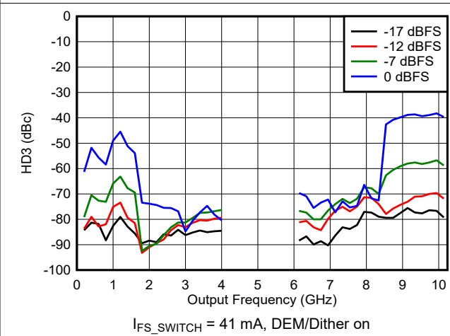
6-168. HD3 vs Frequency and Digital Amplitude in DES2X Modes
