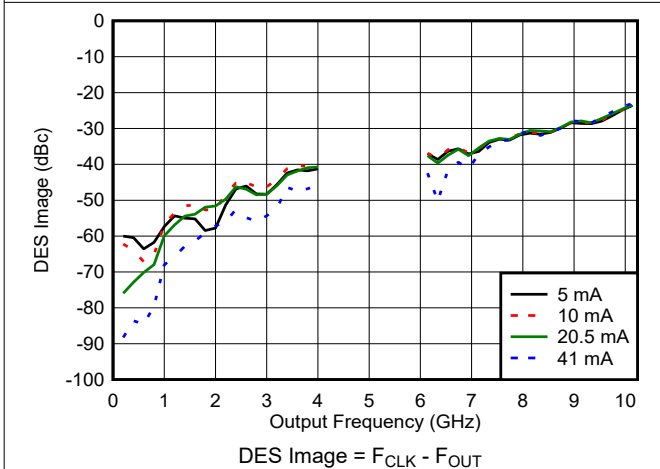
6-193. DES Image vs Frequency and Output Current in DES2X Modes
