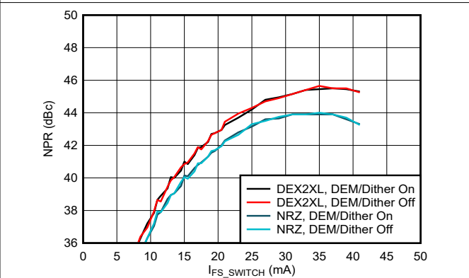
6-200. Noise Power Ratio vs Output Current: 2nd Nyquist Zone
