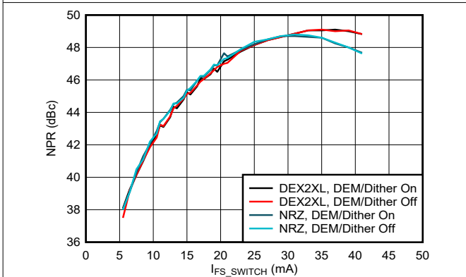
6-199. Noise Power Ratio vs Output Current: 1st Nyquist Zone
