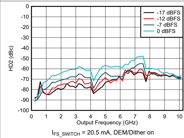
6-146. HD2 vs Frequency and Digital Amplitude in NRZ/RF Modes
