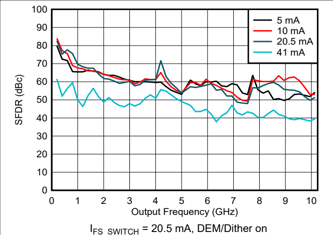
Figure 6-98. SFDR vs Frequency and Output Current in NRZ/RF Modes
