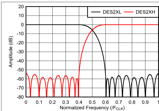
図 7-48. DES Interpolator Frequency Response
