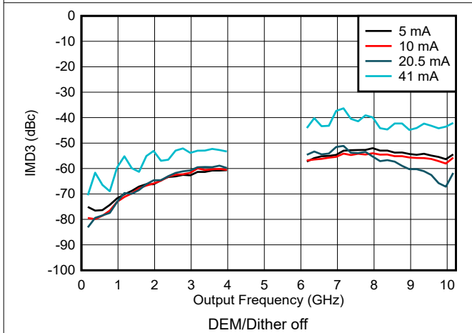
6-115. IMD3 vs Frequency and Output Current in DES2X Modes
