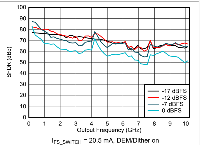
6-102. SFDR vs Frequency and Digital Amplitude in NRZ/RF Modes
