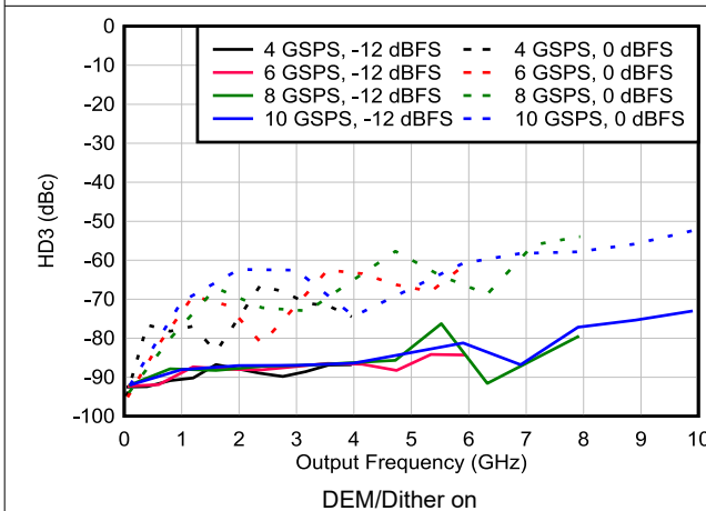
6-169. HD3 vs Frequency and Sample Rate in NRZ/RF Modes
