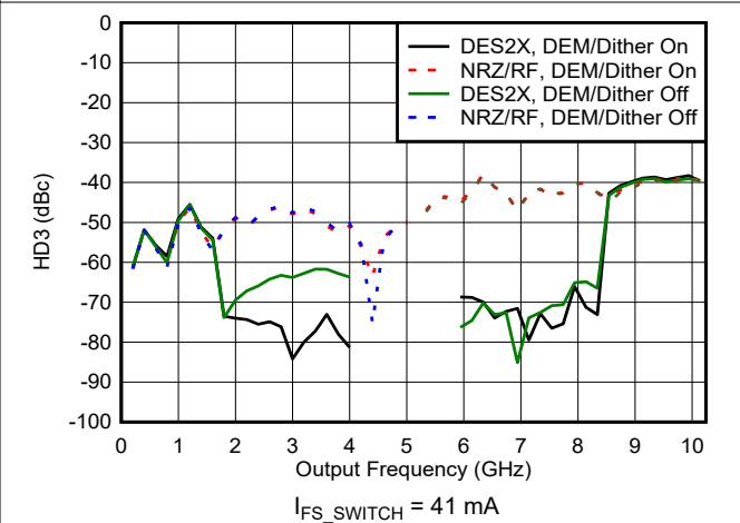
Figure 6-96. HD3 vs Frequency and Mode
