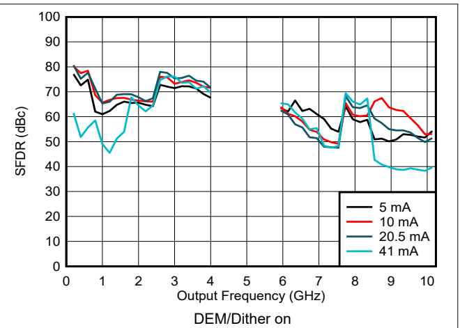
6-100. SFDR vs Frequency and Output Current in DES2X Modes
