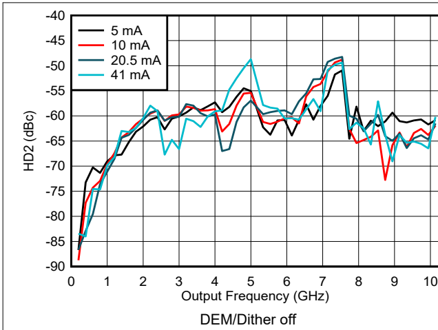
6-141. HD2 vs Frequency and Output Current in NRZ/RF Modes
