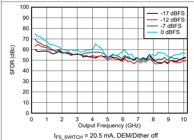
6-101. SFDR vs Frequency and Digital Amplitude in NRZ/RF Modes
