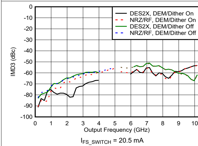
Figure 6-91. IMD3 vs Frequency and Mode
