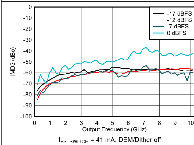
6-119. IMD3 vs Frequency and Digital Amplitude in NRZ/RF Modes
