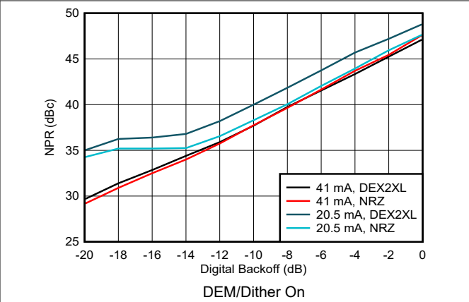
6-196. Noise Power Ratio vs Digital Backoff: 1st Nyquist Zone
