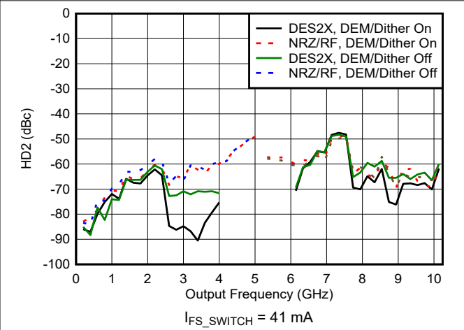
Figure 6-94. HD2 vs Frequency and Mode
