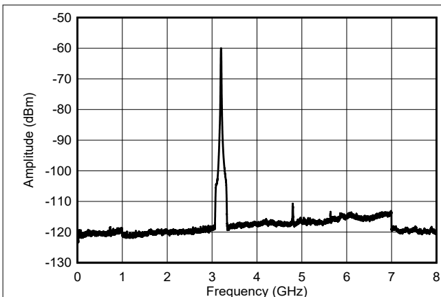
8-18. NLFM Chirp Output Spectra across 0 - 8 GHz
