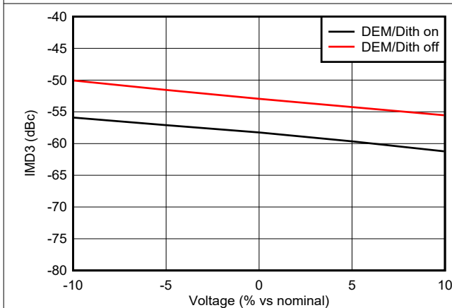
6-139. IMD3 vs Voltage in RF Mode at 7247 MHz
