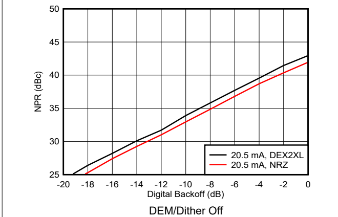
6-197. Noise Power Ratio vs Digital Backoff: 2nd Nyquist Zone
