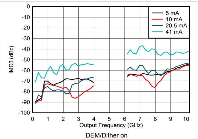
6-116. IMD3 vs Frequency and Output Current in DES2X Modes
