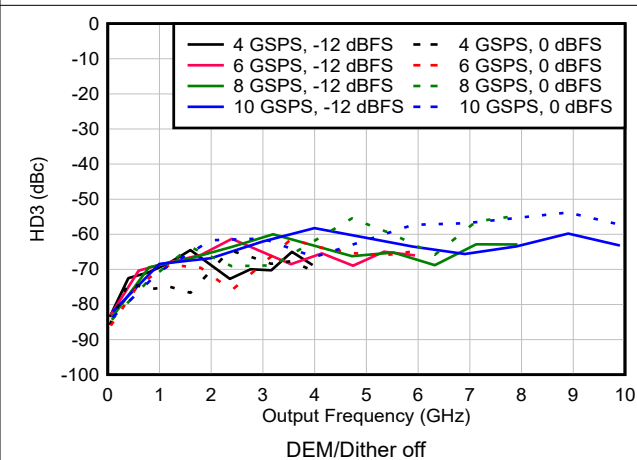
6-170. HD3 vs Frequency and Sample Rate in NRZ/RF Modes
