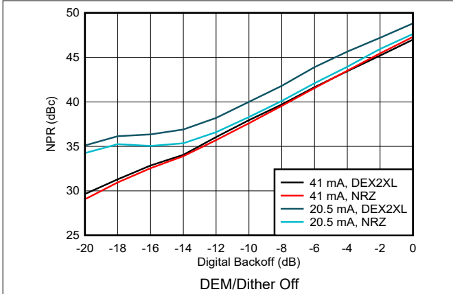
6-195. Noise Power Ratio vs Digital Backoff: 1st Nyquist Zone
