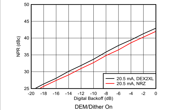
6-198. Noise Power Ratio vs Digital Backoff: 2nd Nyquist Zone
