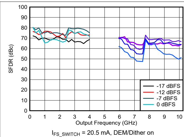
6-106. SFDR vs Frequency and Digital Amplitude in DES2X Modes
