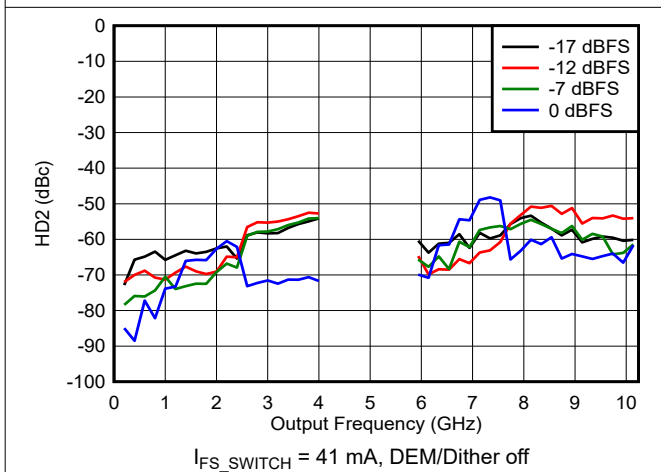
6-151. HD2 vs Frequency and Digital Amplitude in DES2X Modes
