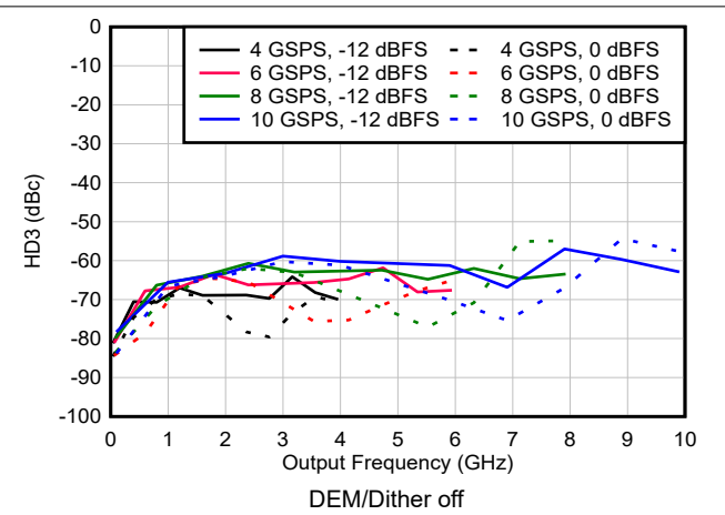
6-172. HD3 vs Frequency and Sample Rate in DES2X Modes
