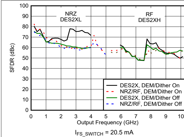
Figure 6-89. SFDR vs Frequency and Mode
