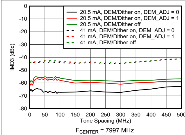
6-127. IMD3 vs Tone Spacing in RF Mode
