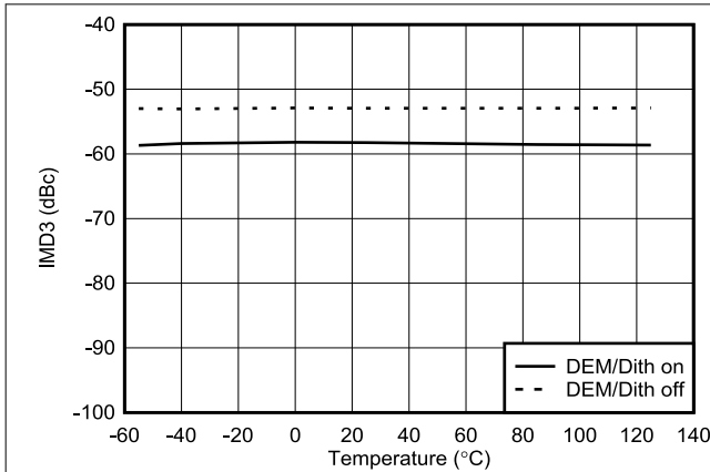
6-135. IMD3 vs Temperature in RF Mode at 7247 MHz
