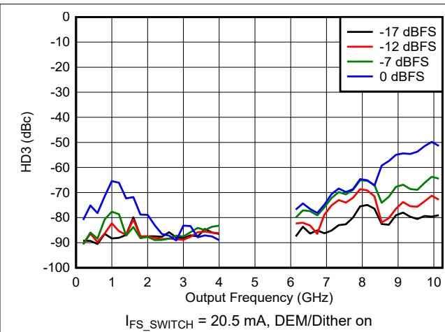
6-166. HD3 vs Frequency and Digital Amplitude in DES2X Modes
