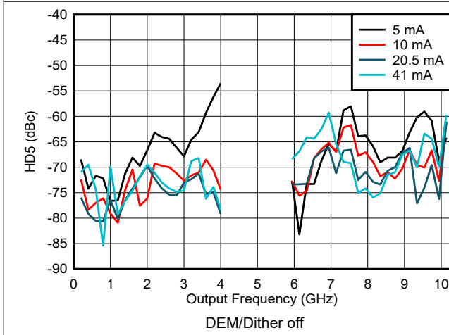
图 6-179. HD5 vs Frequency and Output Current in DES2X Modes
