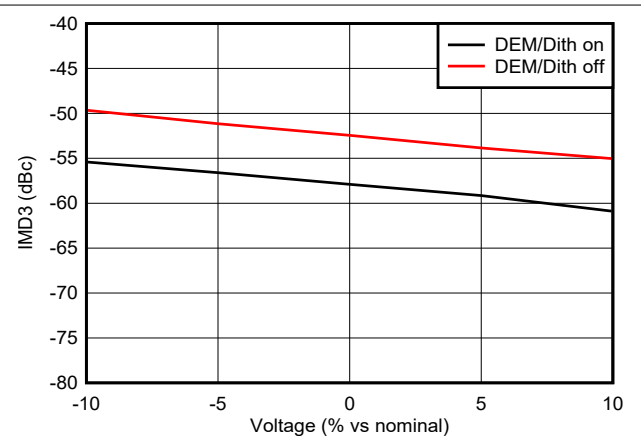
6-140. IMD3 vs Voltage in DES2XH Mode at 7247 MHz
