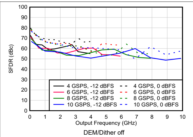
6-112. SFDR vs Frequency and Sample Rate in DES2X Modes
