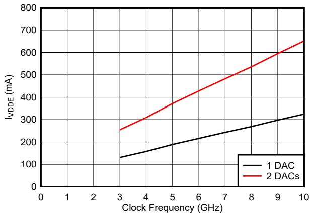
Figure 6-221. VDDE Current vs Clock Frequency
