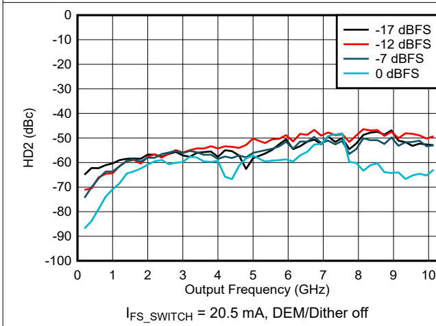
6-145. HD2 vs Frequency and Digital Amplitude in NRZ/RF Modes
