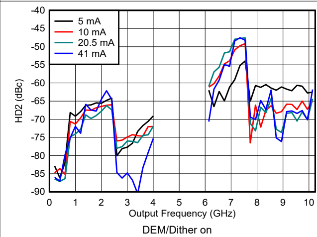
6-144. HD2 vs Frequency and Output Current in DES2X Modes
