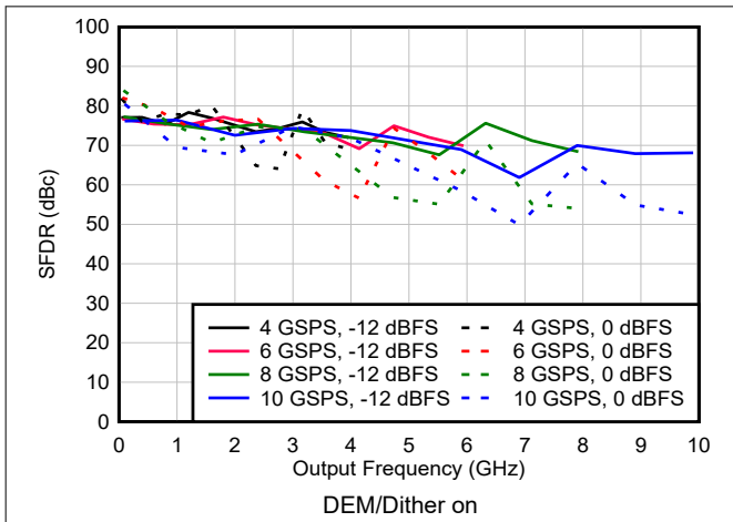
6-111. SFDR vs Frequency and Sample Rate in DES2X Modes
