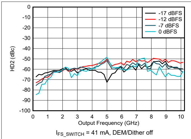
6-147. HD2 vs Frequency and Digital Amplitude in NRZ/RF Modes
