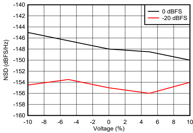
图 6-86. NSD vs Supply Voltage
