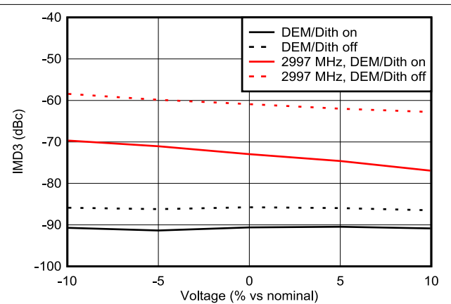
6-138. IMD3 vs Voltage in DES2XL Mode
