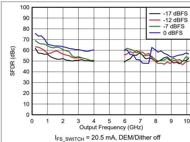
6-105. SFDR vs Frequency and Digital Amplitude in DES2X Modes
