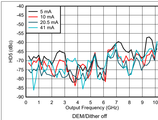
图 6-177. HD5 vs Frequency and Output Current in NRZ/RF Modes
