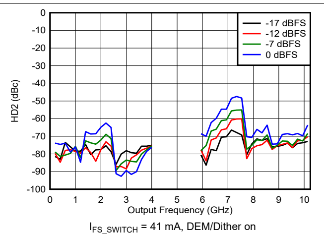
6-152. HD2 vs Frequency and Digital Amplitude in DES2X Modes
