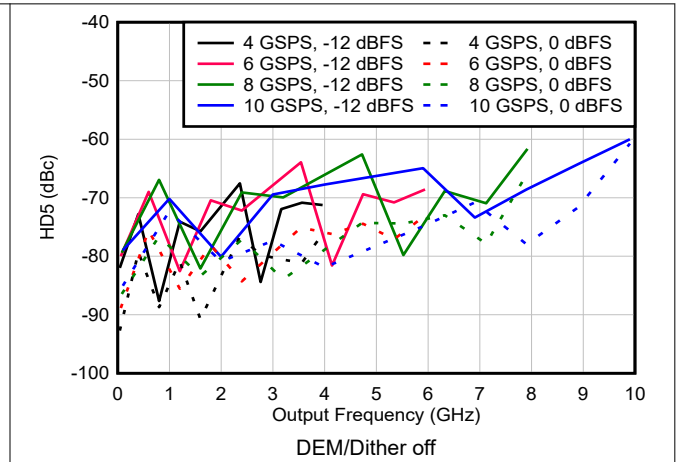
6-190. HD5 vs Frequency and Sample Rate in NRZ/RF Modes
