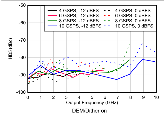
6-191. HD5 vs Frequency and Sample Rate in DES2X Modes
