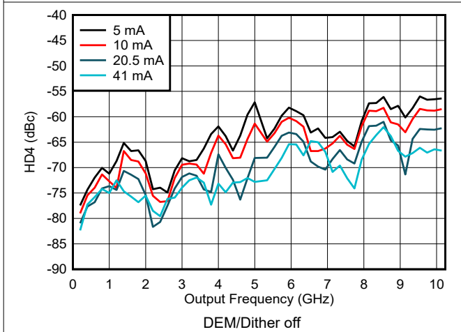
6-173. HD4 vs Frequency and Output Current in NRZ/RF Modes
