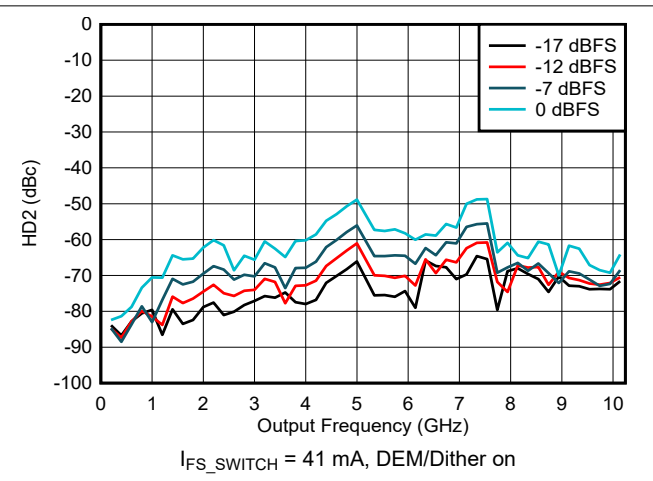
6-148. HD2 vs Frequency and Digital Amplitude in NRZ/RF Modes
