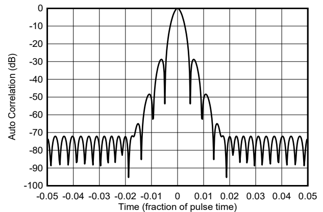
8-17. Auto-correlation of NLFM Chirp
