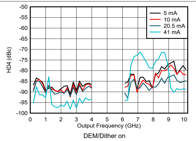
6-176. HD4 vs Frequency and Output Current in DES2X Modes
