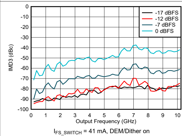
6-120. IMD3 vs Frequency and Digital Amplitude in NRZ/RF Modes
