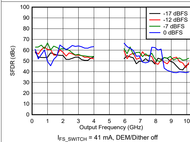
6-107. SFDR vs Frequency and Digital Amplitude in DES2X Modes
