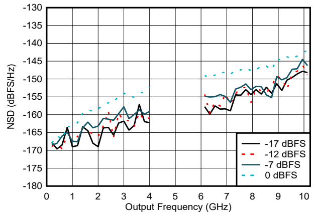
6-69. NSD vs Output Frequency and Digital Amplitude
