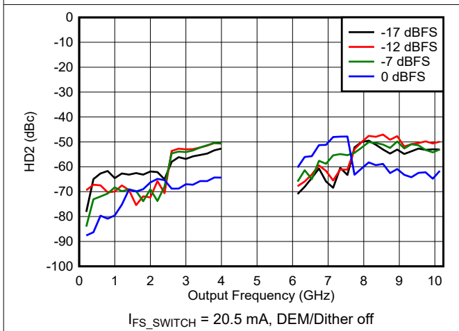
6-149. HD2 vs Frequency and Digital Amplitude in DES2X Modes
