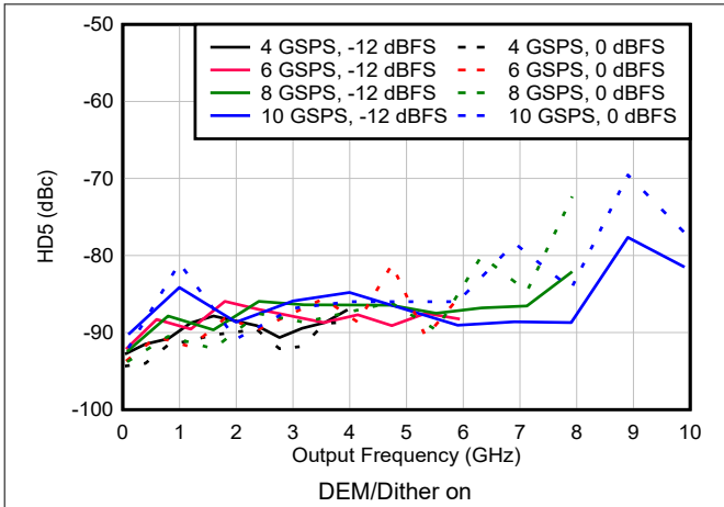
6-189. HD5 vs Frequency and Sample Rate in NRZ/RF Modes
