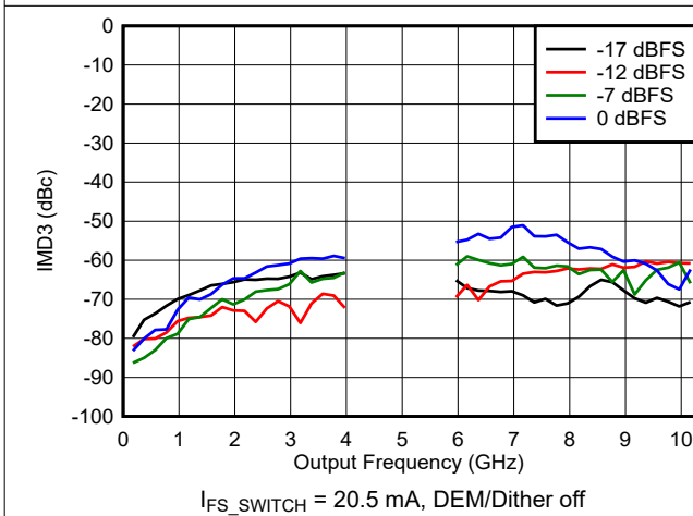
6-121. IMD3 vs Frequency and Digital Amplitude in DES2X Modes
