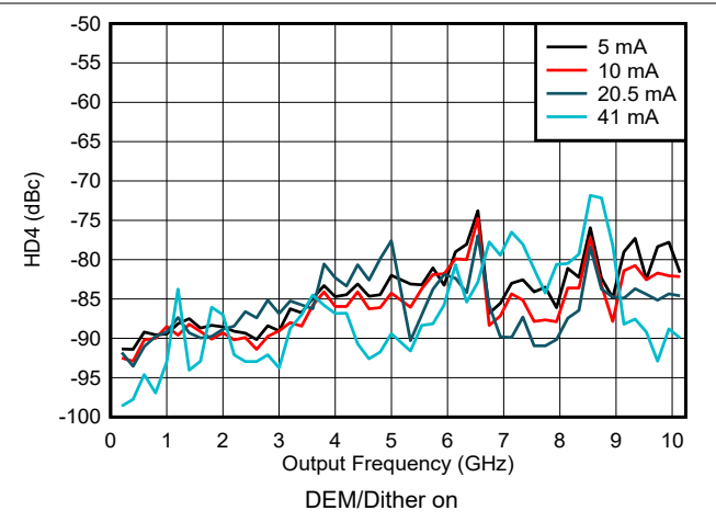
6-174. HD4 vs Frequency and Output Current in NRZ/RF Modes
