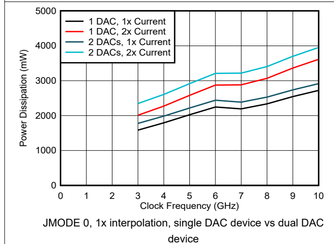
6-215. Power Dissipation vs Clock Frequency and DAC Mode
