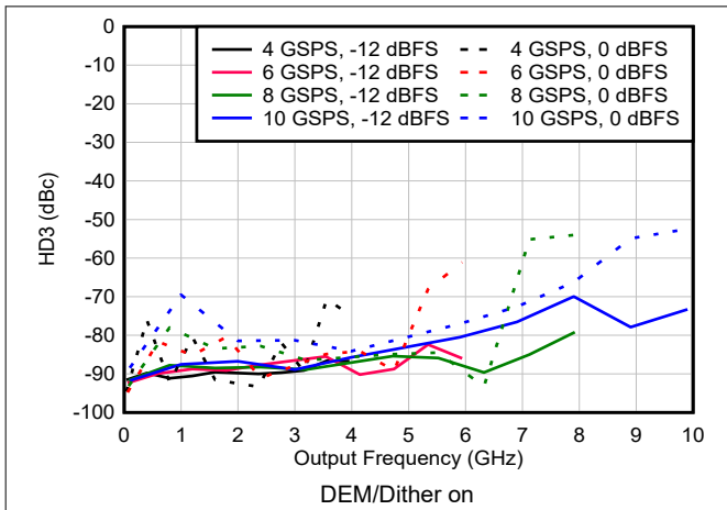
6-171. HD3 vs Frequency and Sample Rate in DES2X Modes
