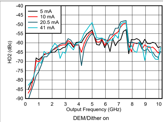
6-142. HD2 vs Frequency and Output Current in NRZ/RF Modes
