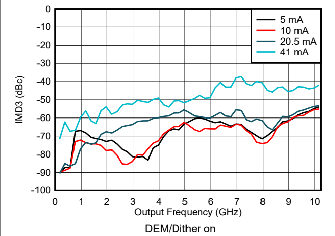
6-114. IMD3 vs Frequency and Output Current in NRZ/RF Modes
