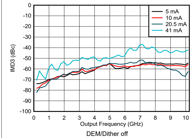
6-113. IMD3 vs Frequency and Output Current in NRZ/RF Modes
