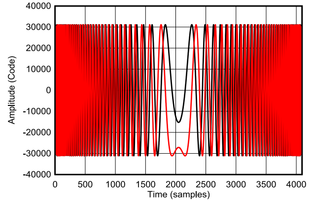
8-15. Complex Time Domain of NLFM Chirp (Red = real, Black = imag)
