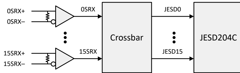
7-53. Crossbar Block Diagram
