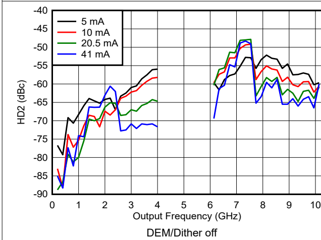
6-143. HD2 vs Frequency and Output Current in DES2X Modes
