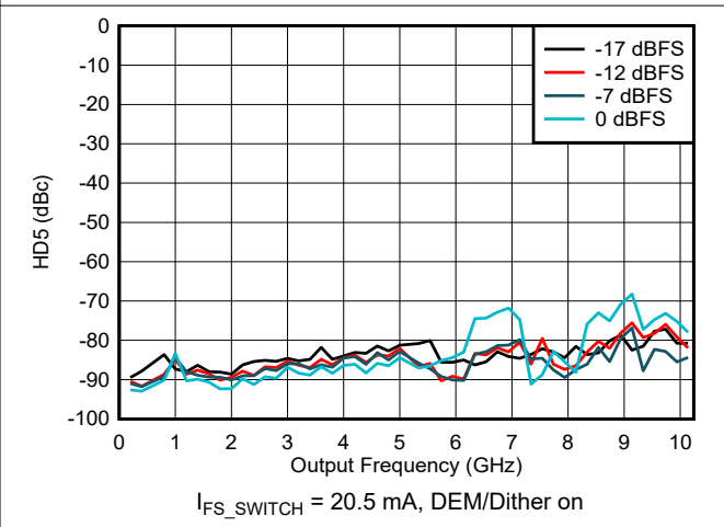
图 6-182. HD5 vs Frequency and Digital Amplitude in NRZ/RF Modes
