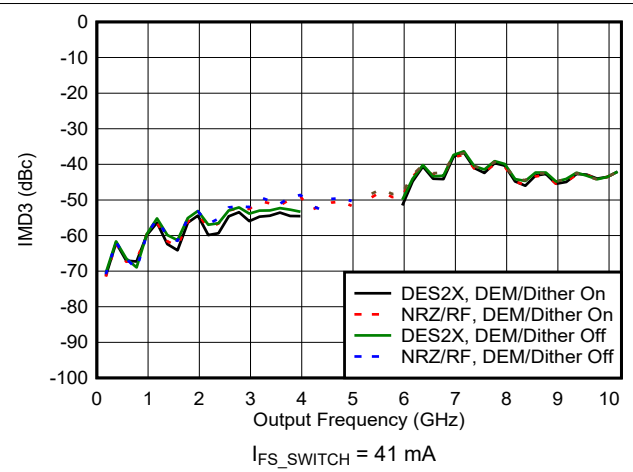
Figure 6-92. IMD3 vs Frequency and Mode
