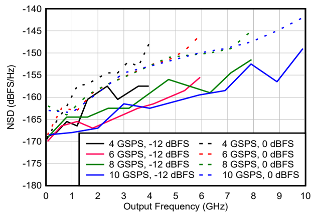
6-77. NSD vs Output Frequency and Sample Rate
