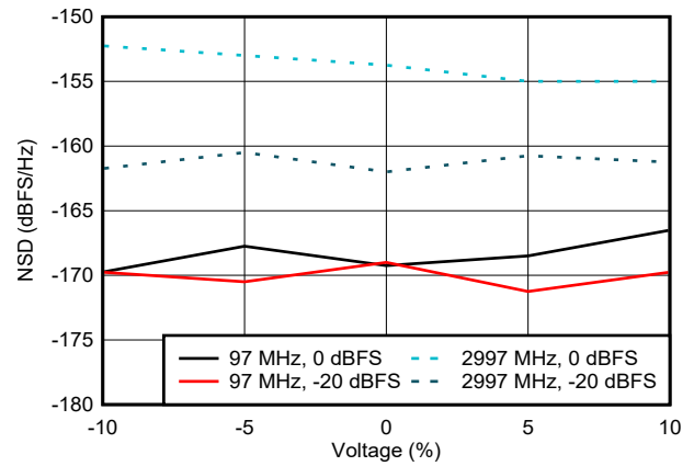
图 6-87. NSD vs Supply Voltage
