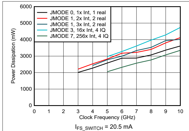
6-211. Power Dissipation vs Clock Frequency and Digital Mode
