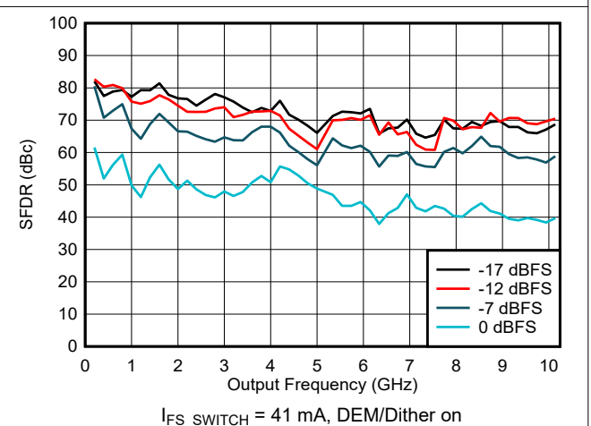
6-104. SFDR vs Frequency and Digital Amplitude in NRZ/RF Modes
