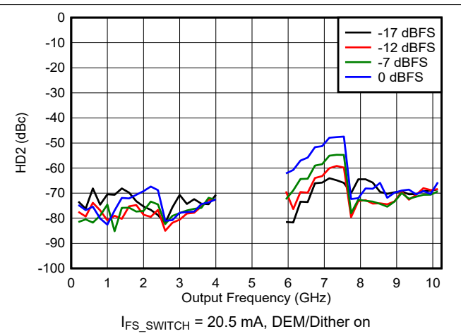
6-150. HD2 vs Frequency and Digital Amplitude in DES2X Modes
