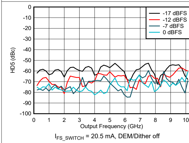
图 6-181. HD5 vs Frequency and Digital Amplitude in NRZ/RF Modes
