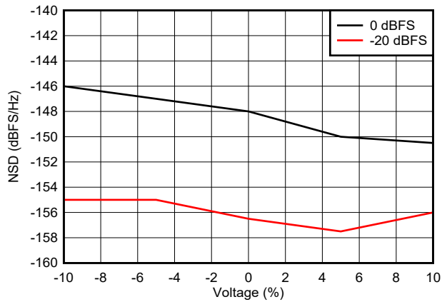
图 6-86. NSD vs Supply Voltage
