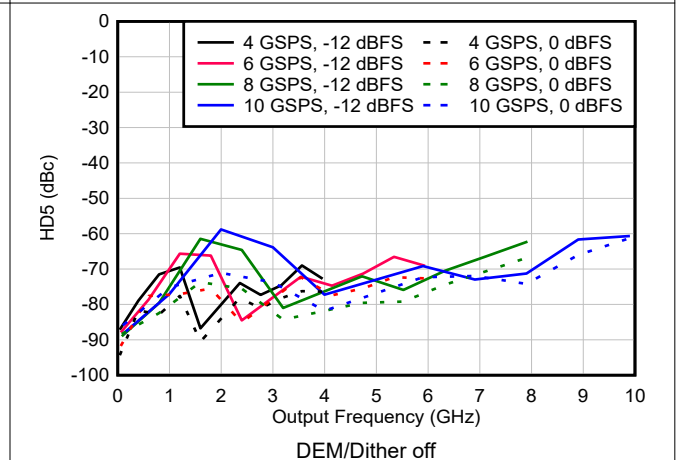
6-192. HD5 vs Frequency and Sample Rate in DES2X Modes
