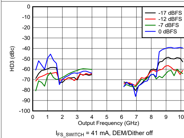
6-167. HD3 vs Frequency and Digital Amplitude in DES2X Modes
