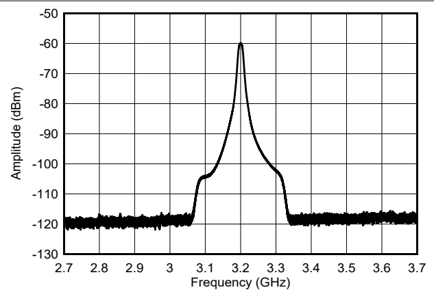
8-19. NLFM Chirp Output Spectra across 1 GHz
