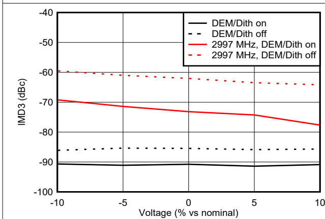
6-137. IMD3 vs Voltage in NRZ Mode
