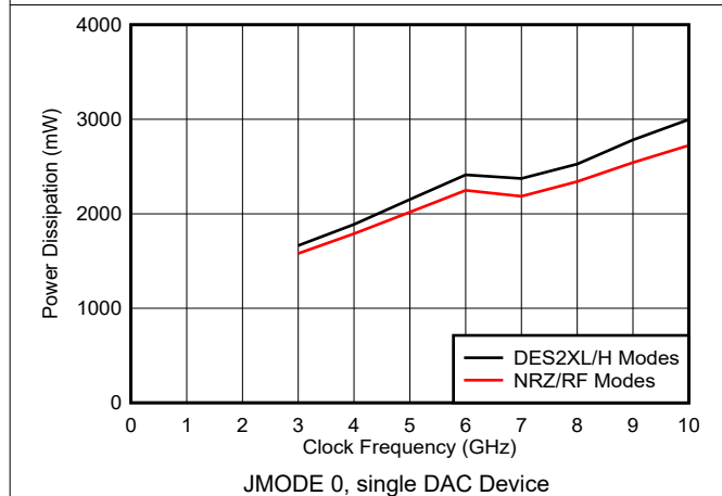
6-213. Power Dissipation vs Clock Frequency and DAC Mode
