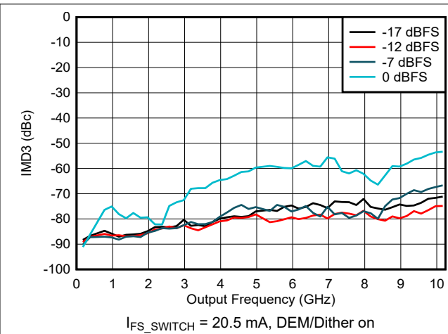
6-118. IMD3 vs Frequency and Digital Amplitude in NRZ/RF Modes
