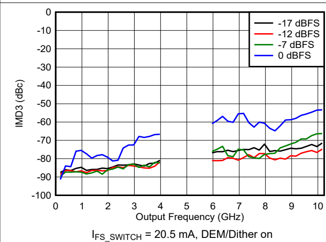
6-122. IMD3 vs Frequency and Digital Amplitude in DES2X Modes
