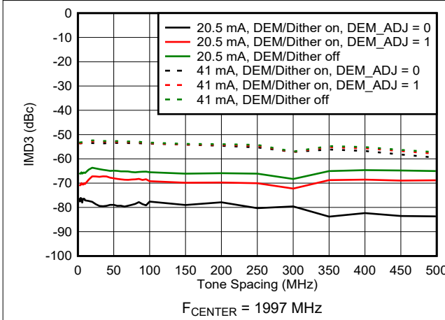
6-125. IMD3 vs Tone Spacing in NRZ Mode
