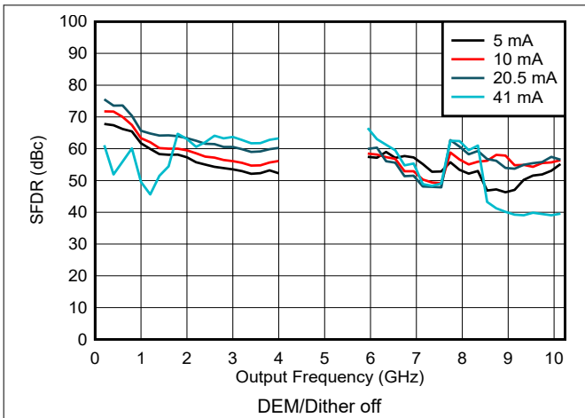
6-99. SFDR vs Frequency and Output Current in DES2X Modes
