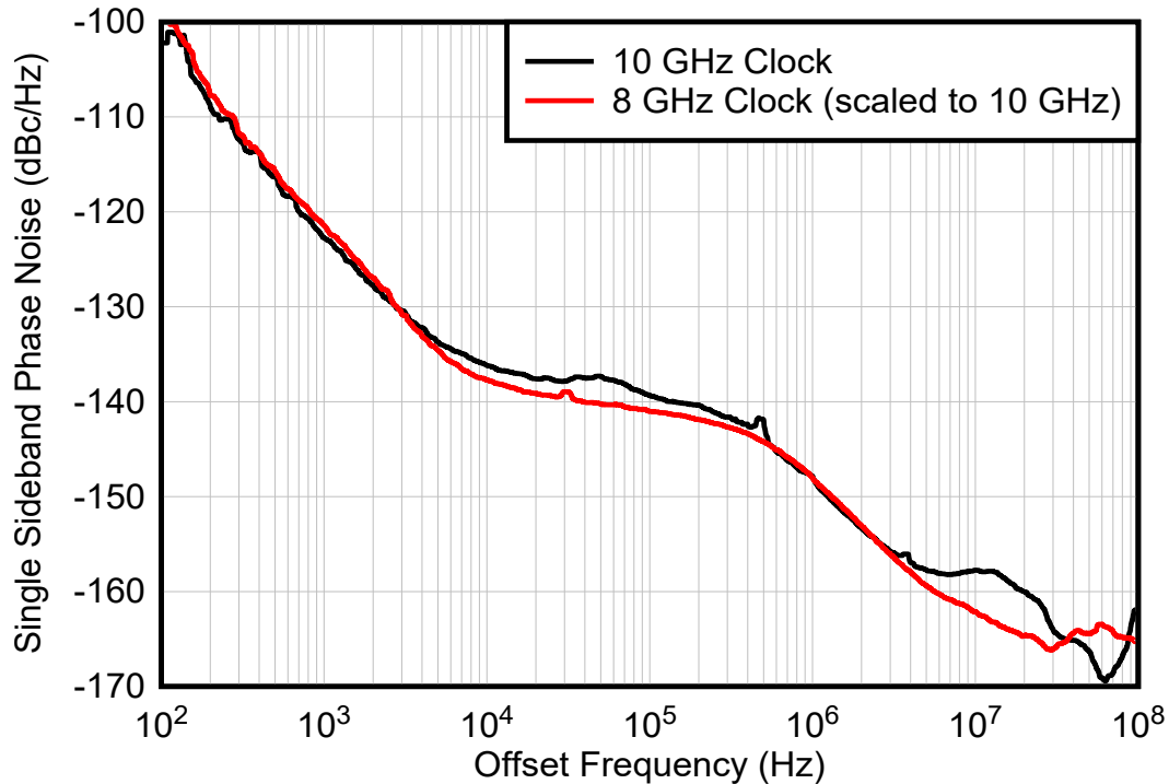
☒ 8-13. 8 GHz and 10 GHz Clock Phase Noise
