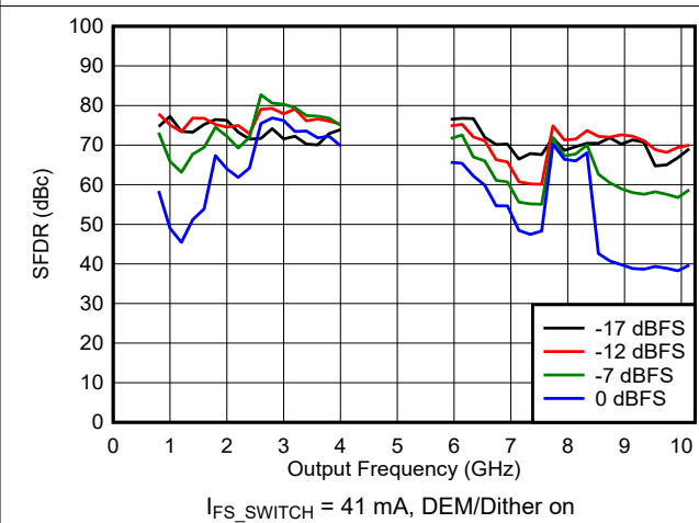
6-108. SFDR vs Frequency and Digital Amplitude in DES2X Modes
