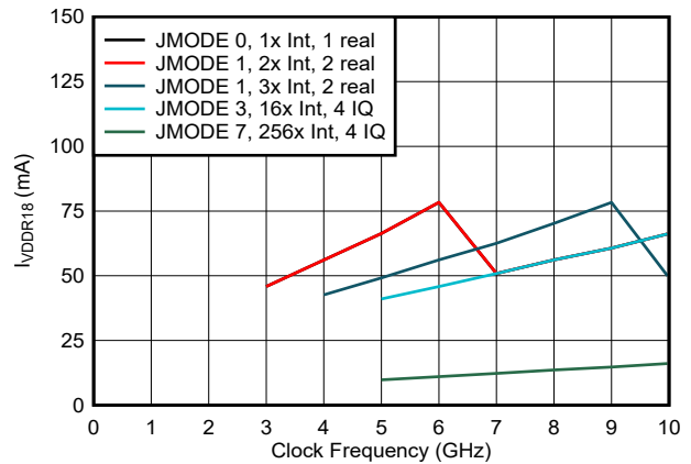
Figure 6-222. VDDR18 Current vs Clock Frequency and Mode
