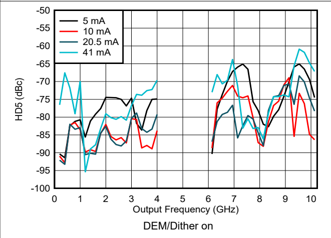
图 6-180. HD5 vs Frequency and Output Current in DES2X Modes
