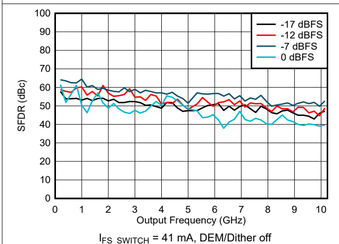
6-103. SFDR vs Frequency and Digital Amplitude in NRZ/RF Modes
