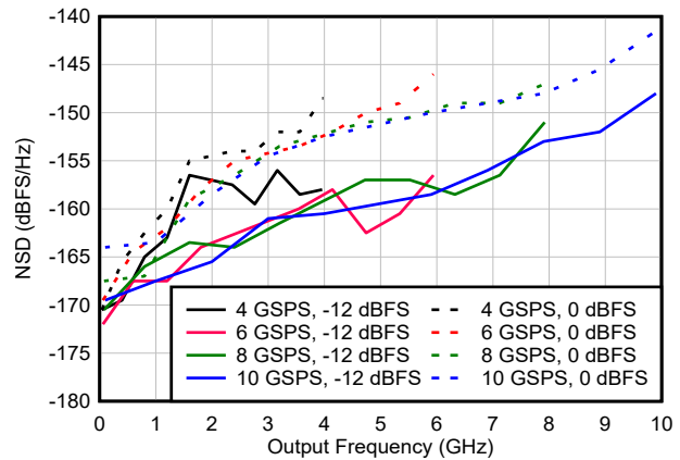
6-75. NSD vs Output Frequency and Digital Amplitude
