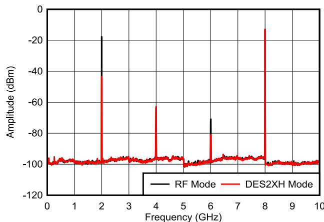
☒ 8-4. Output Spectra Comparing DES2XH and RF Modes
