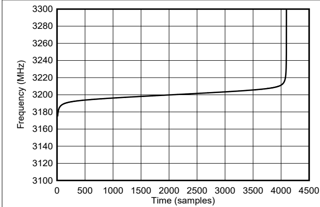
8-14. NLFM Frequency Ramp
