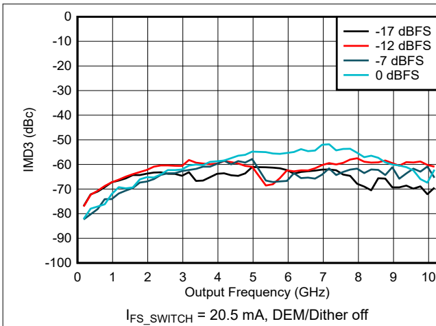
6-117. IMD3 vs Frequency and Digital Amplitude in NRZ/RF Modes
