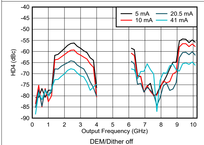
6-175. HD4 vs Frequency and Output Current in DES2X Modes
