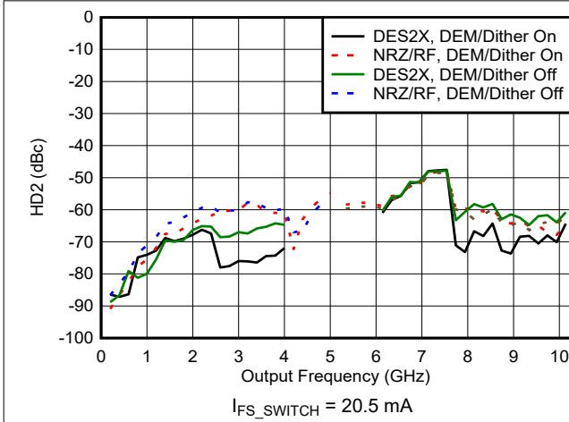
Figure 6-93. HD2 vs Frequency and Mode
