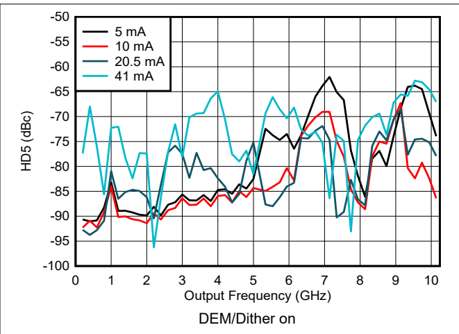
图 6-178. HD5 vs Frequency and Output Current in NRZ/RF Modes
