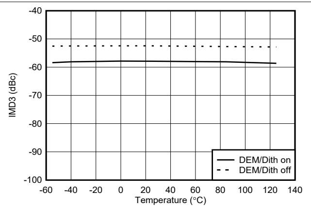
6-136. IMD3 vs Temperature in DES2XH Mode at 7247 MHz
