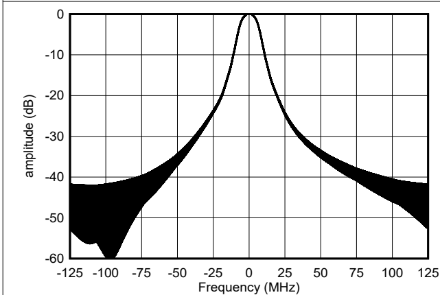
8-16. Digital Spectrum for NLFM Chirp
