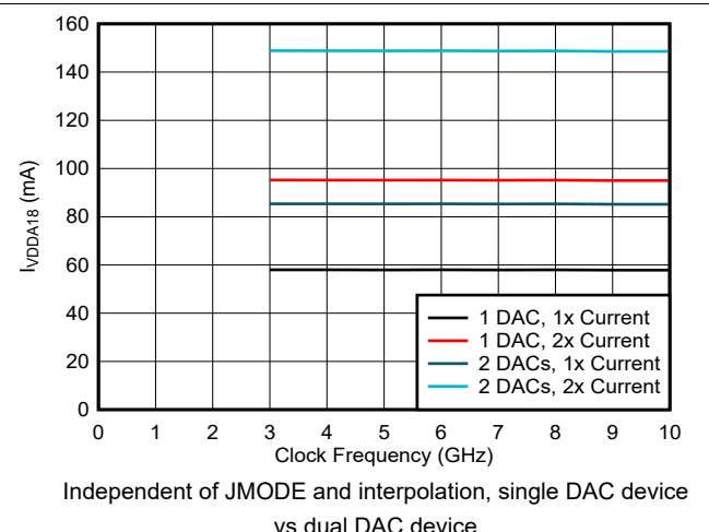
6-216. VDDA18 Current vs Clock Frequency and DAC Mode
