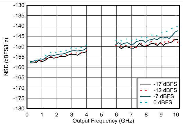
6-71. NSD vs Output Frequency and Digital Amplitude
