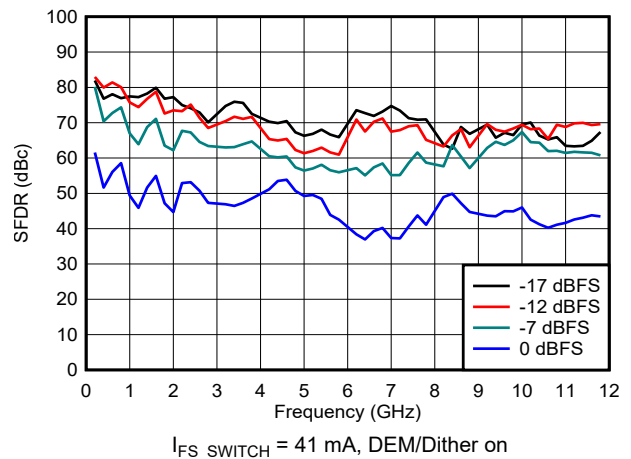
6-97. SFDR vs Frequency and Digital Amplitude in NRZ/RF Modes
