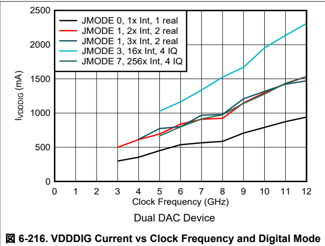
图 6-216. VDDDIG Current vs Clock Frequency and Digital Mode
