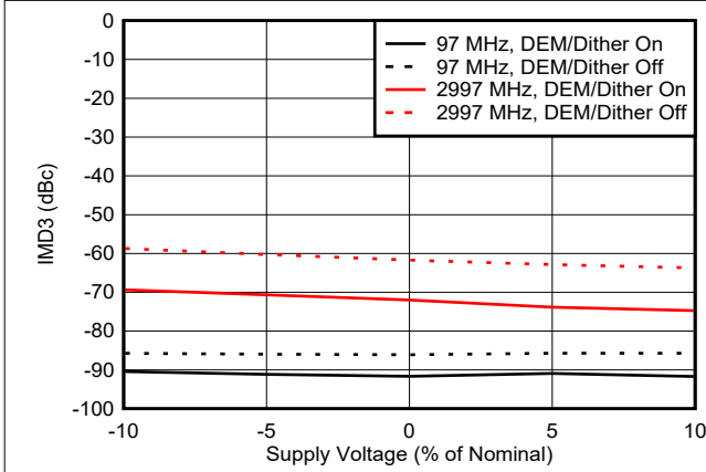
6-130. IMD3 vs Voltage in NRZ Mode
