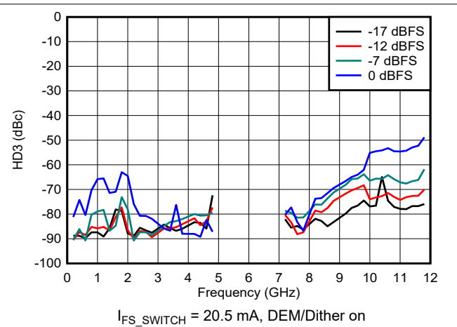
Figure 6-159. HD3 vs Frequency and Digital Amplitude in DES2X Modes
