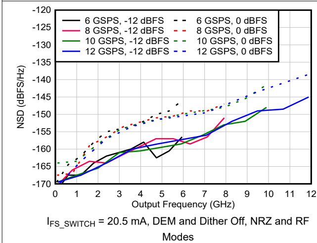
6-72. NSD vs Output Frequency and Sample Rate
