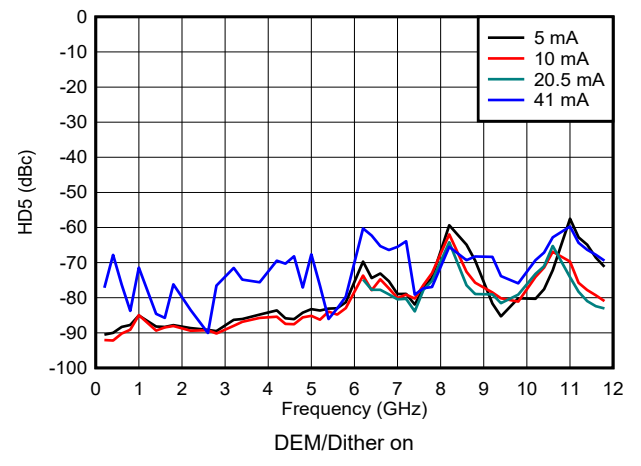
6-175. HD5 vs Frequency and Output Current in NRZ/RF Modes
