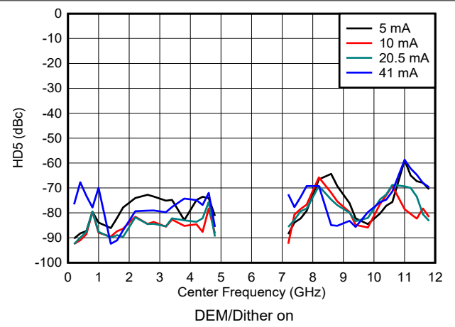
6-177. HD5 vs Frequency and Output Current in DES2X Modes
