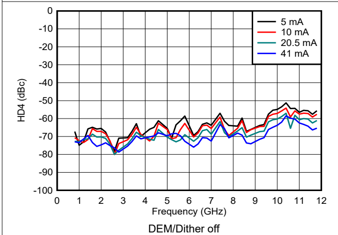
Figure 6-166. HD4 vs Frequency and Output Current in NRZ/RF Modes
