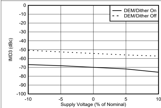
6-132. IMD3 vs Voltage in RF Mode at 9002 MHz
