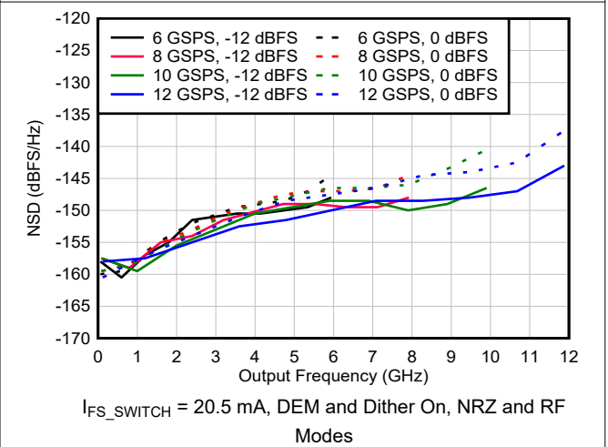
6-73. NSD vs Output Frequency and Sample Rate
