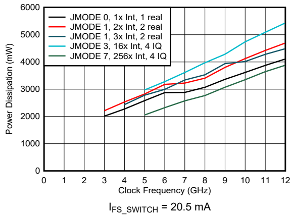
6-203. Power Dissipation vs Clock Frequency and Digital Mode
