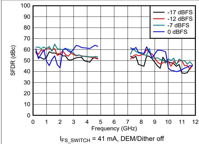
Figure 6-100. SFDR vs Frequency and Digital Amplitude in DES2X Modes
