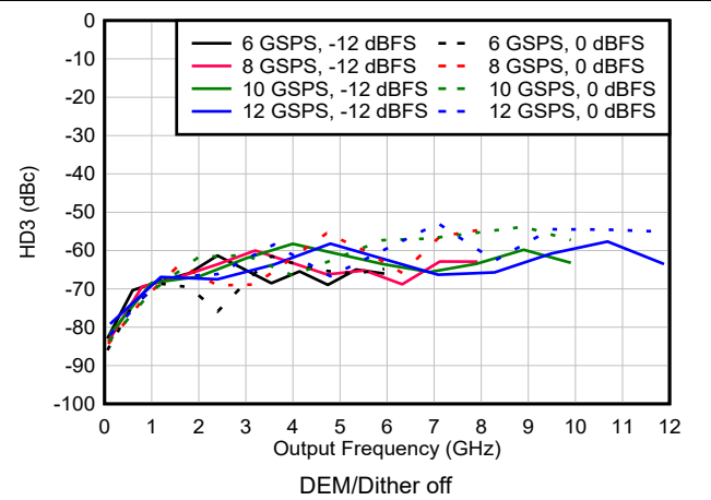
Figure 6-163. HD3 vs Frequency and Sample Rate in NRZ/RF Modes
