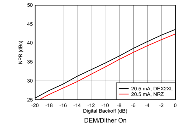
6-190. Noise Power Ratio vs Digital Backoff: 2 nd Nyquist Zone
