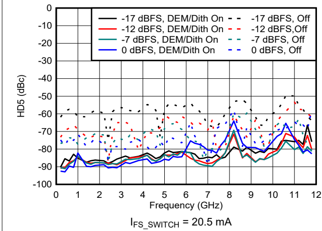
6-178. HD5 vs Frequency and Digital Amplitude in NRZ/RF Modes
