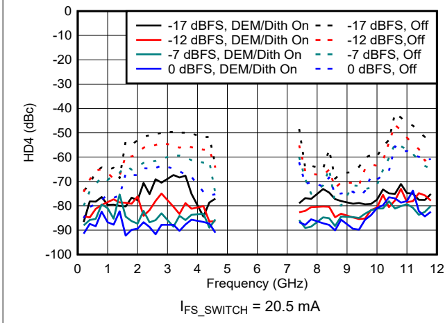
6-172. HD4 vs Frequency and Digital Amplitude in NRZ/RF Modes
