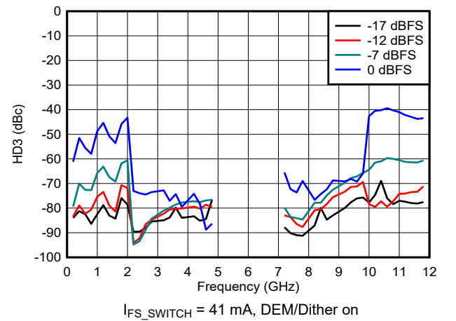
Figure 6-161. HD3 vs Frequency and Digital Amplitude in DES2X Modes
