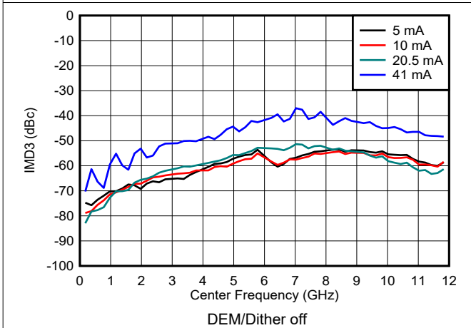
Figure 6-106. IMD3 vs Frequency and Output Current in NRZ/RF Modes
