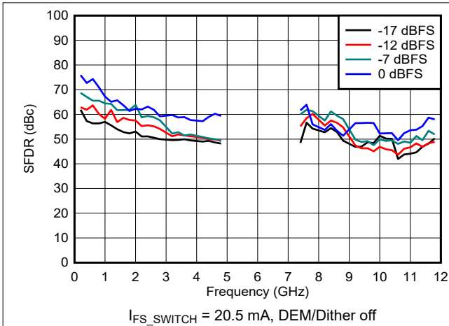
Figure 6-98. SFDR vs Frequency and Digital Amplitude in DES2X Modes
