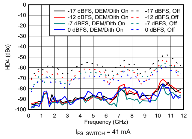
6-173. HD4 vs Frequency and Digital Amplitude in NRZ/RF Modes
