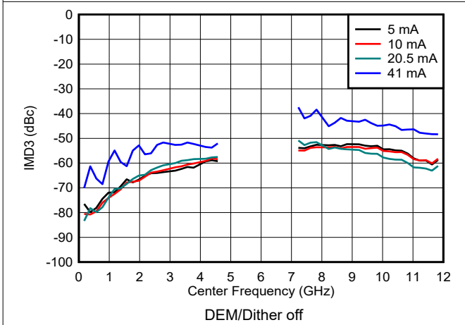
Figure 6-108. IMD3 vs Frequency and Output Current in DES2X Modes
