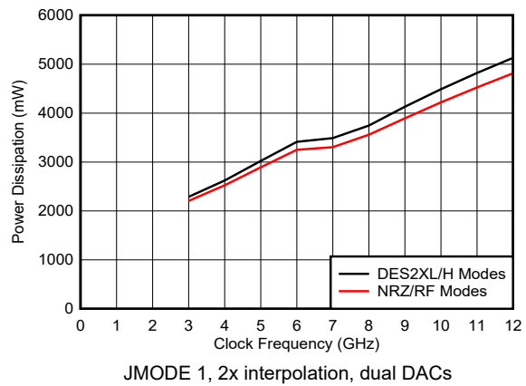
6-206. Power Dissipation vs Clock Frequency and DAC Mode
