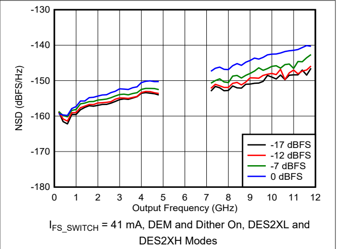
6-71. NSD vs Output Frequency and Digital Amplitude
