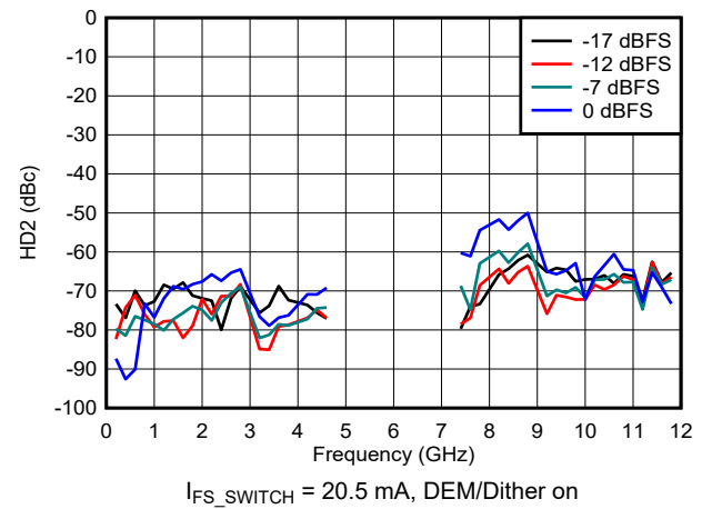
Figure 6-143. HD2 vs Frequency and Digital Amplitude in DES2X Modes
