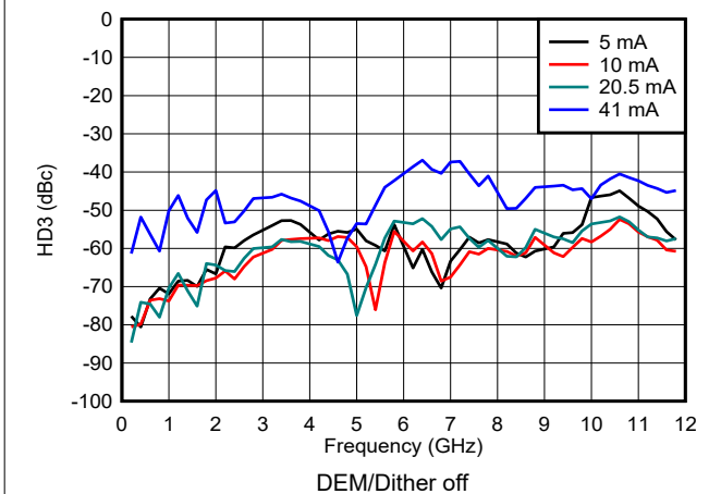
6-150. HD3 vs Frequency and Output Current in NRZ/RF Modes
