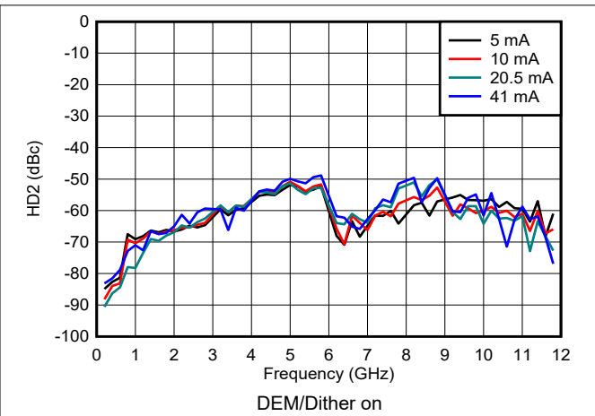
6-135. HD2 vs Frequency and Output Current in NRZ/RF Modes
