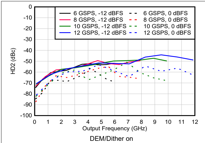
6-146. HD2 vs Frequency and Sample Rate in NRZ/RF Modes
