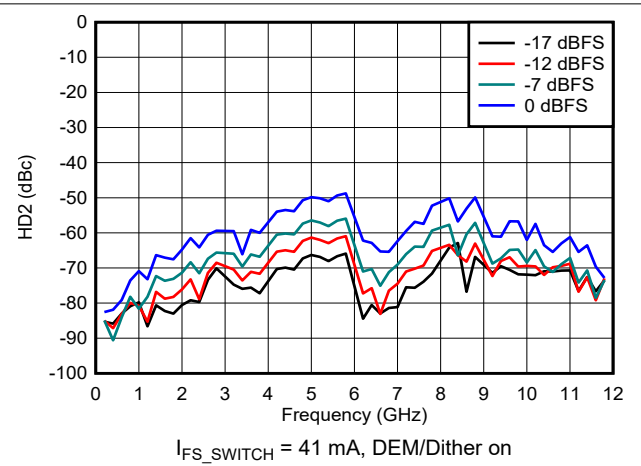
Figure 6-141. HD2 vs Frequency and Digital Amplitude in NRZ/RF Modes
