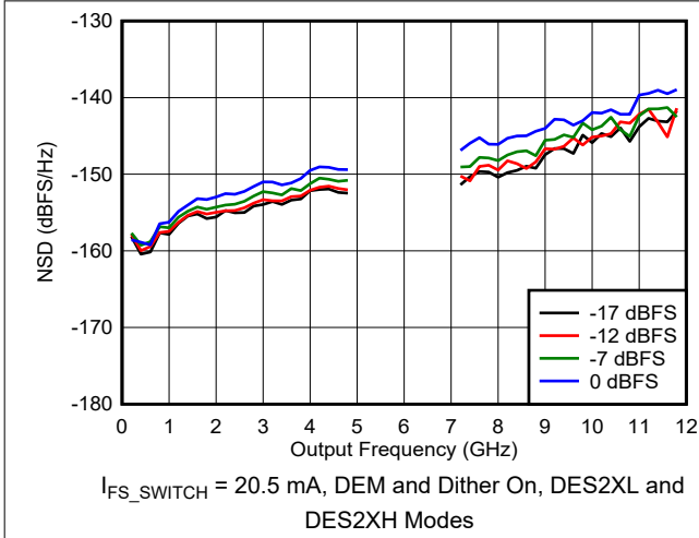
6-70. NSD vs Output Frequency and Digital Amplitude
