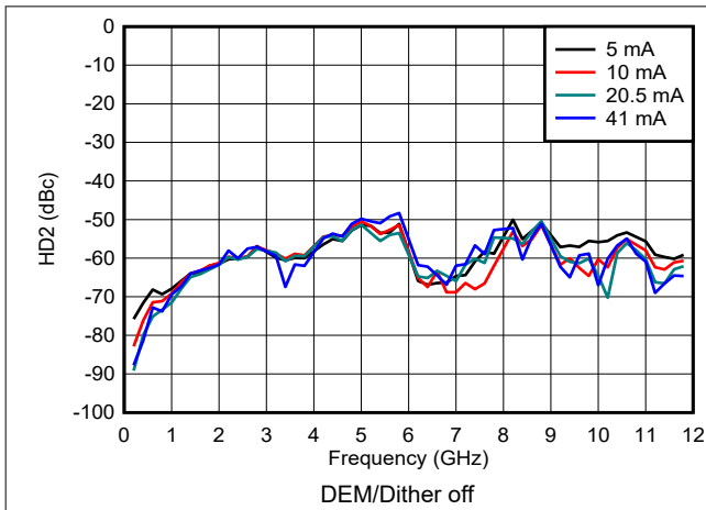
6-134. HD2 vs Frequency and Output Current in NRZ/RF Modes
