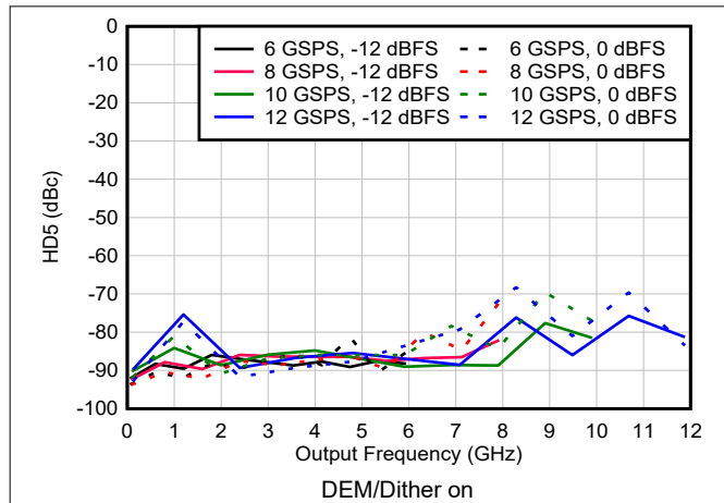
Figure 6-182. HD5 vs Frequency and Sample Rate in NRZ/RF Modes
