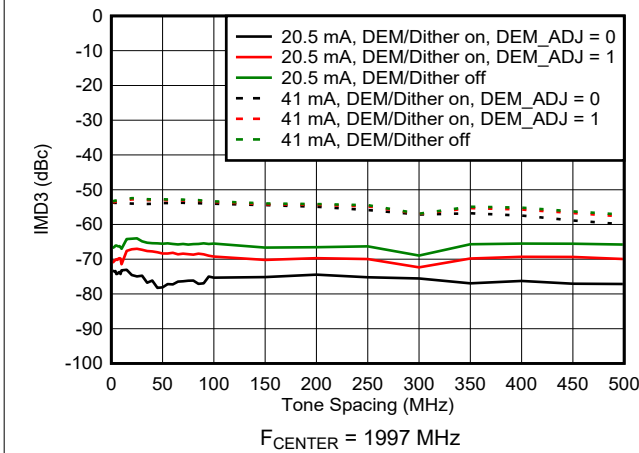
Figure 6-118. IMD3 vs Tone Spacing in NRZ Mode
