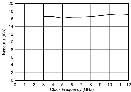
6-209. VDDCLK18 Current vs Clock Frequency
