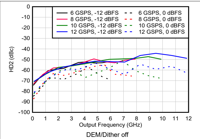
6-147. HD2 vs Frequency and Sample Rate in NRZ/RF Modes
