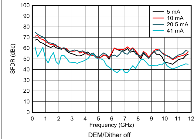
Figure 6-90. SFDR vs Frequency and Output Current in NRZ/RF Modes
