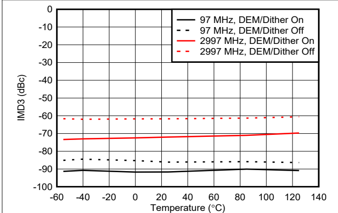
6-126. IMD3 vs Temperature in NRZ Mode
