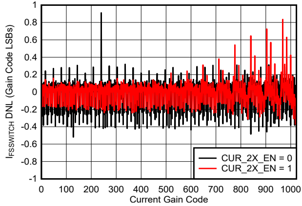
6-18. I_{\text{FS\_SWITCH}} Error Differential Non-Linearity vs Gain Code
