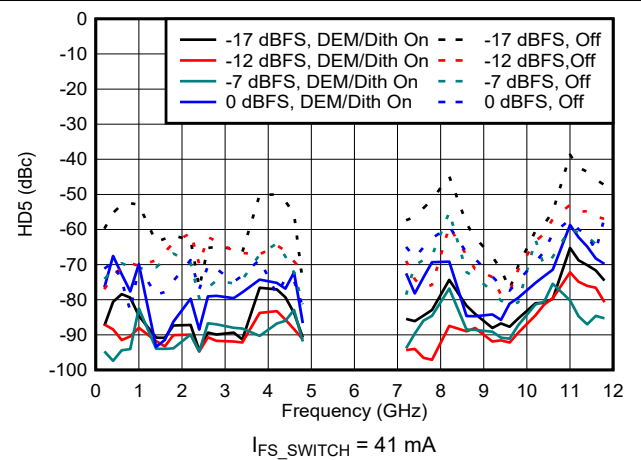
6-181. HD5 vs Frequency and Digital Amplitude in DES2X Modes
