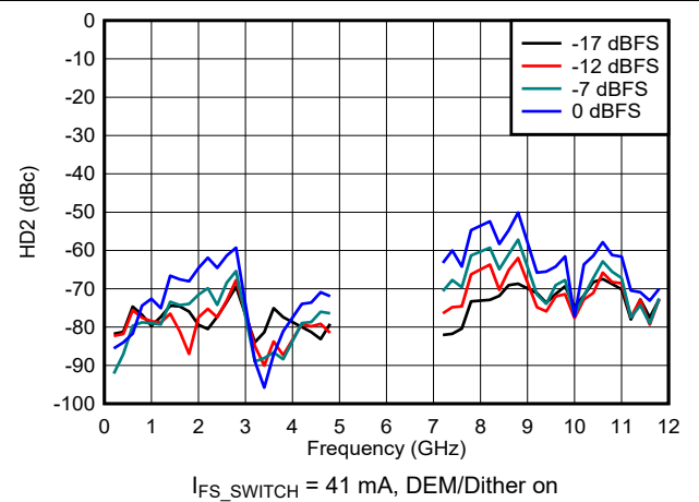
Figure 6-145. HD2 vs Frequency and Digital Amplitude in DES2X Modes
