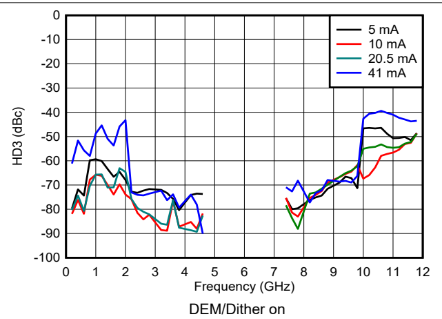
6-153. HD3 vs Frequency and Output Current in DES2X Modes
