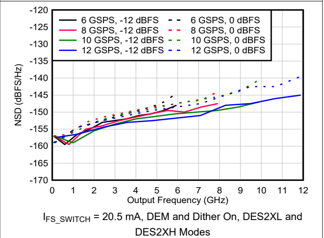
6-75. NSD vs Output Frequency and Sample Rate
