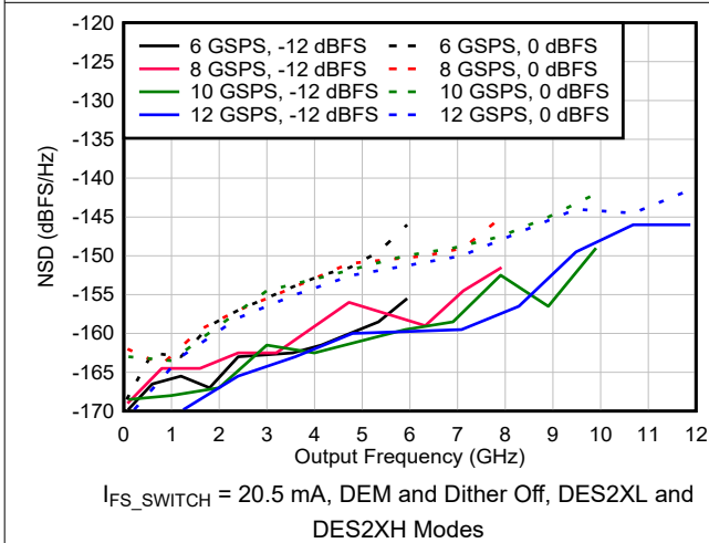
6-74. NSD vs Output Frequency and Sample Rate
