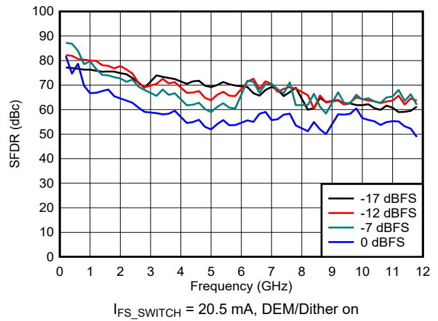
6-95. SFDR vs Frequency and Digital Amplitude in NRZ/RF Modes
