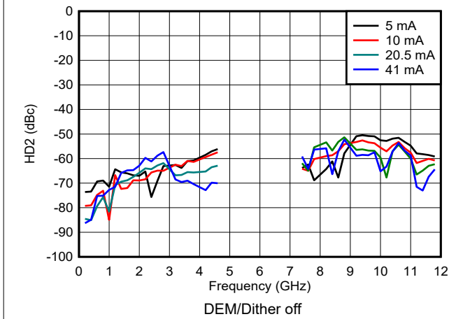
6-136. HD2 vs Frequency and Output Current in DES2X Modes
