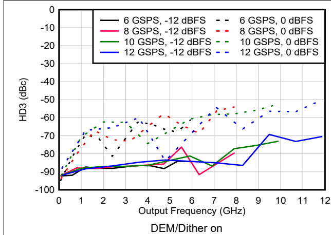
Figure 6-162. HD3 vs Frequency and Sample Rate in NRZ/RF Modes
