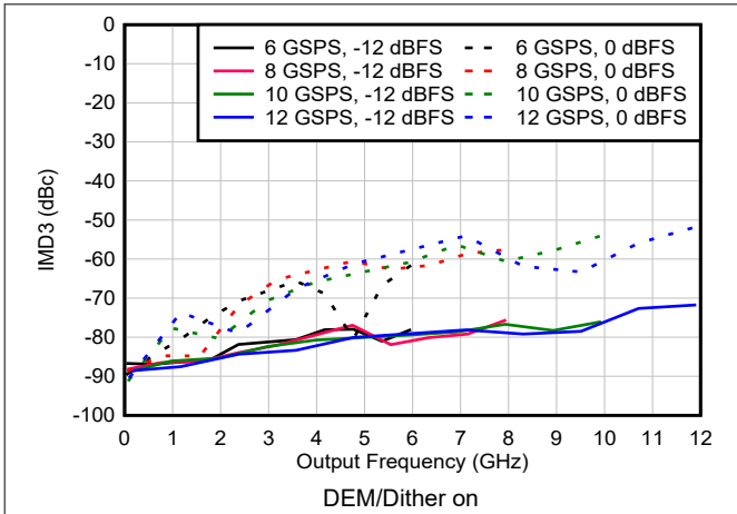
6-122. IMD3 vs Frequency and Sample Rate in NRZ/RF Modes
