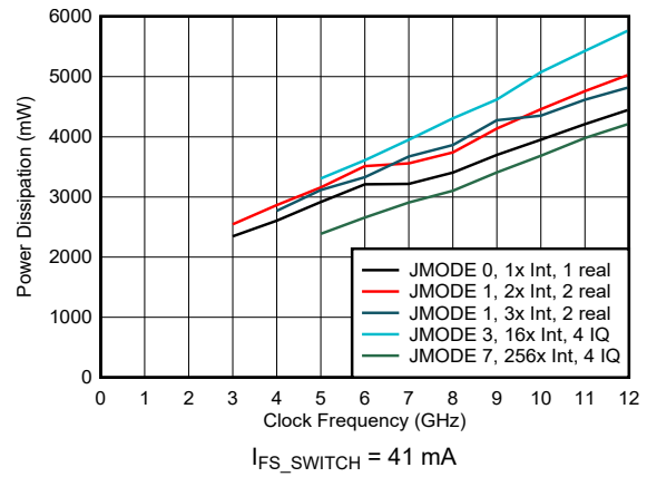
6-204. Power Dissipation vs Clock Frequency and Digital Mode
