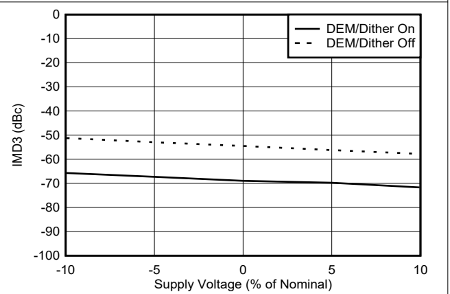
6-133. IMD3 vs Voltage in DES2XH Mode at 9002 MHz
