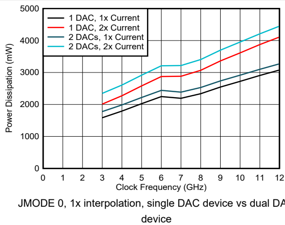
6-207. Power Dissipation vs Clock Frequency and DAC Mode
