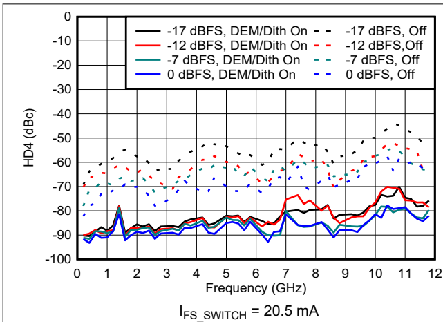
6-170. HD4 vs Frequency and Digital Amplitude in NRZ/RF Modes
