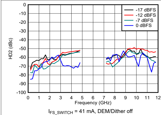
Figure 6-144. HD2 vs Frequency and Digital Amplitude in DES2X Modes
