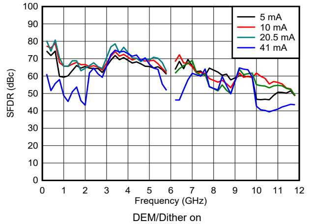
6-93. SFDR vs Frequency and Output Current in DES2X Modes
