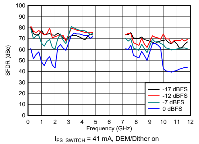
Figure 6-101. SFDR vs Frequency and Digital Amplitude in DES2X Modes
