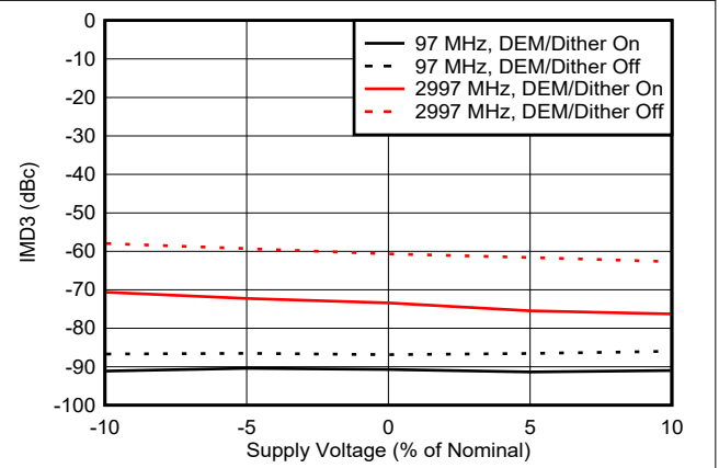
6-131. IMD3 vs Voltage in DES2XL Mode
