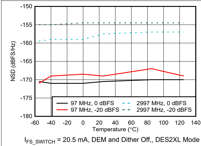
6-78. NSD vs Temperature
