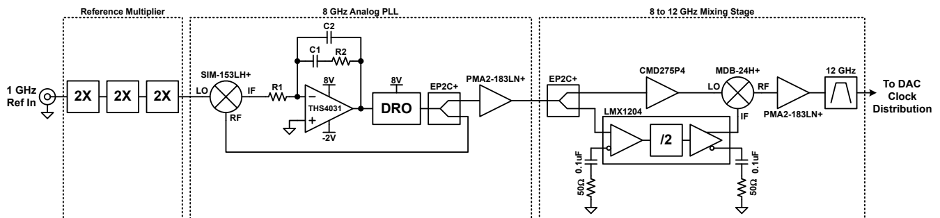
8-11. 12 GHz Clock Synthesizer
