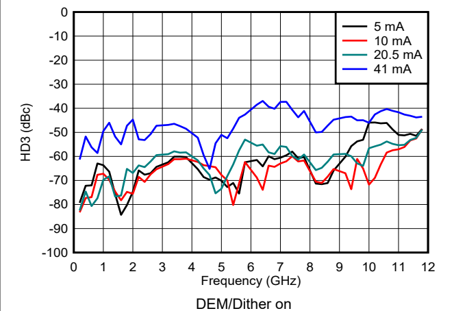
6-151. HD3 vs Frequency and Output Current in NRZ/RF Modes
