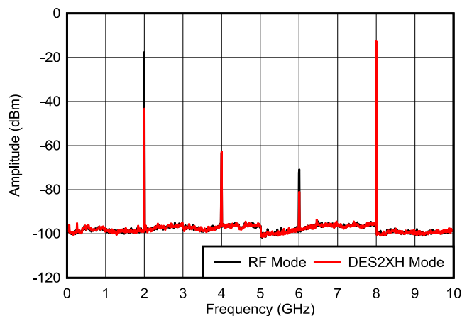
☒ 8-4. Output Spectra Comparing DES2XH and RF Modes
