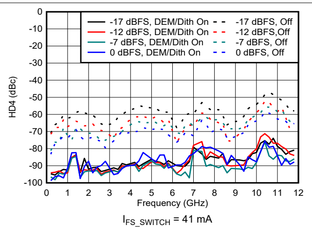
6-171. HD4 vs Frequency and Digital Amplitude in NRZ/RF Modes
