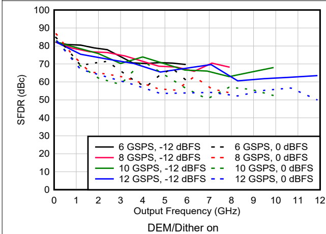
Figure 6-102. SFDR vs Frequency and Sample Rate in NRZ/RF Modes
