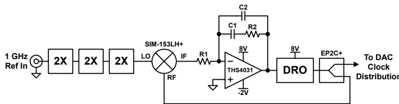
Figure 8-9. Discrete Analog PLL
