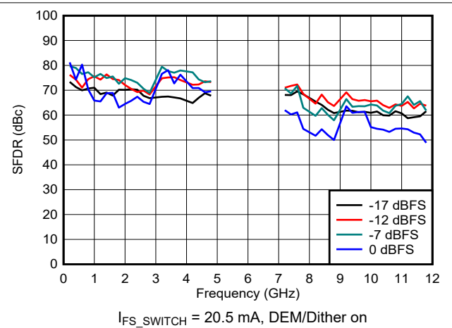
Figure 6-99. SFDR vs Frequency and Digital Amplitude in DES2X Modes
