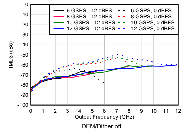
6-125. IMD3 vs Frequency and Sample Rate in DES2X Modes
