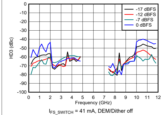
Figure 6-160. HD3 vs Frequency and Digital Amplitude in DES2X Modes
