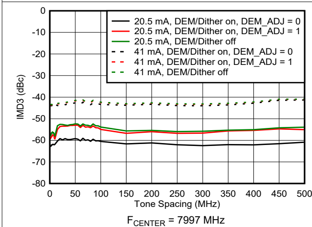
Figure 6-120. IMD3 vs Tone Spacing in RF Mode
