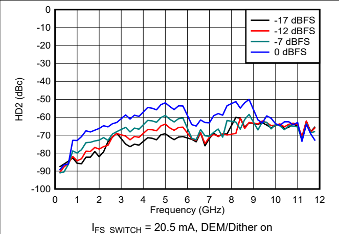
6-139. HD2 vs Frequency and Digital Amplitude in NRZ/RF Modes
