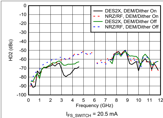
Figure 6-86. HD2 vs Frequency and Mode
