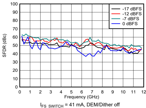
6-96. SFDR vs Frequency and Digital Amplitude in NRZ/RF Modes
