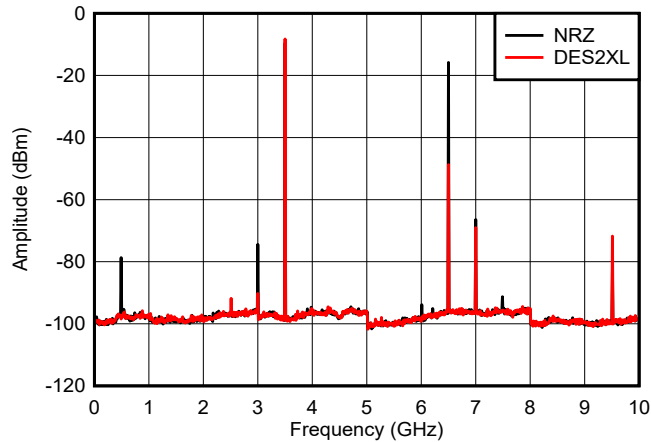
☒ 8-3. Output Spectra Comparing DES2XL and NRZ Modes
