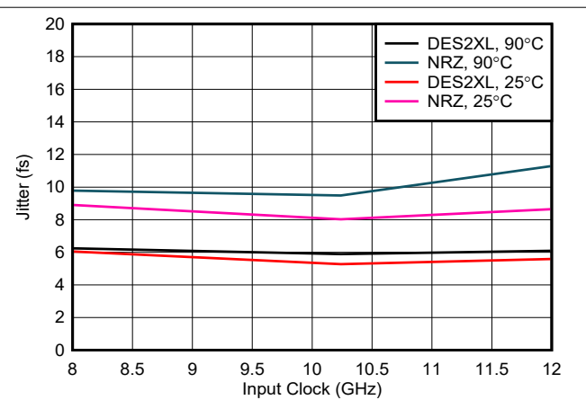
Figure 6-198. Jitter vs Input Clock
