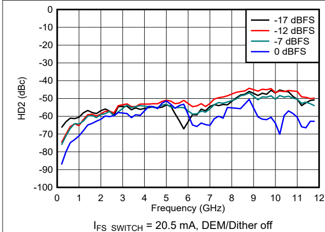
6-138. HD2 vs Frequency and Digital Amplitude in NRZ/RF Modes
