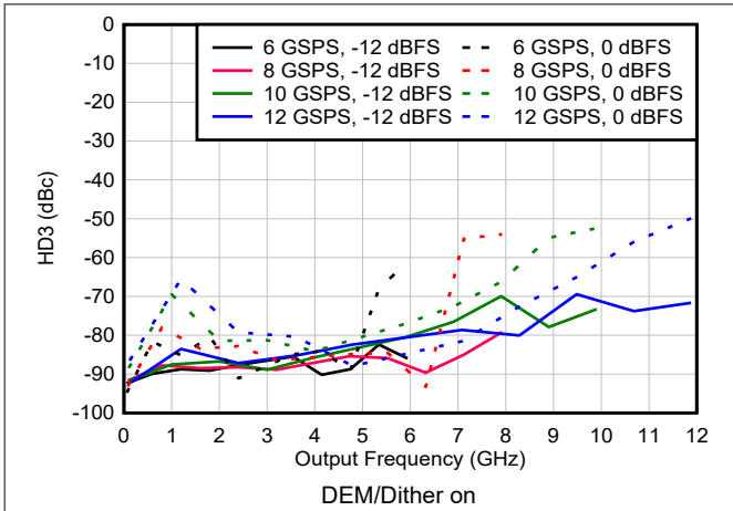
Figure 6-164. HD3 vs Frequency and Sample Rate in DES2X Modes
