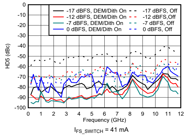
6-179. HD5 vs Frequency and Digital Amplitude in NRZ/RF Modes
