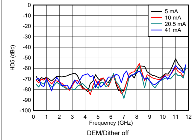
6-174. HD5 vs Frequency and Output Current in NRZ/RF Modes
