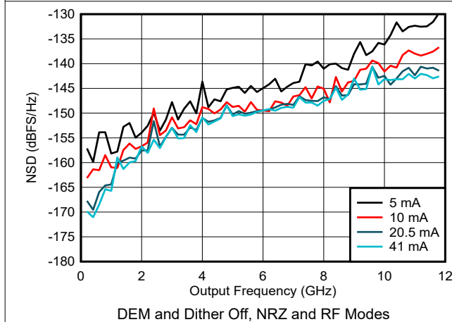
Figure 6-60. NSD vs Output Frequency and Output Current
