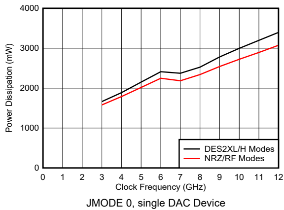
6-205. Power Dissipation vs Clock Frequency and DAC Mode
