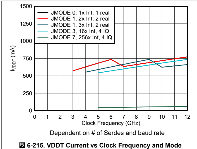
图 6-215. VDDT Current vs Clock Frequency and Mode
