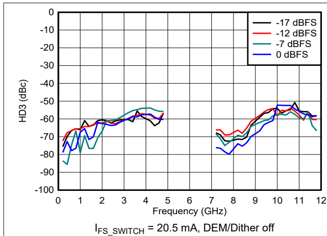
Figure 6-158. HD3 vs Frequency and Digital Amplitude in DES2X Modes
