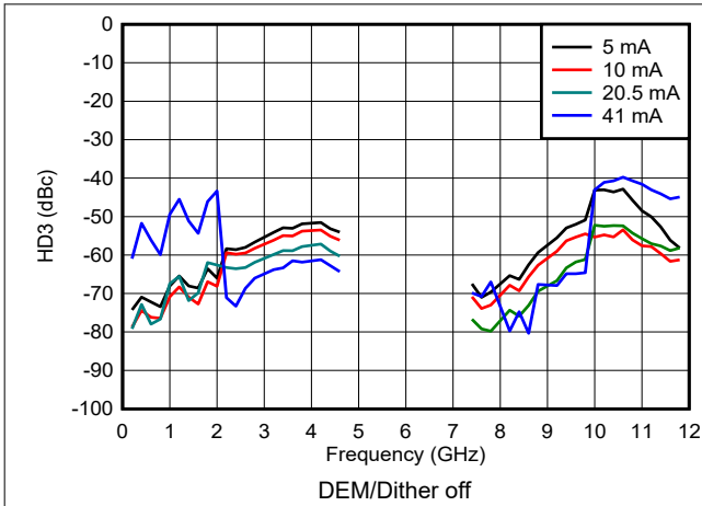
6-152. HD3 vs Frequency and Output Current in DES2X Modes
