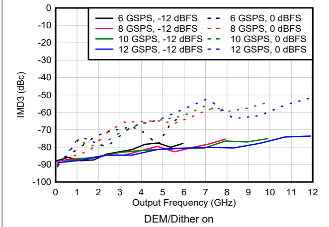
6-124. IMD3 vs Frequency and Sample Rate in DES2X Modes
