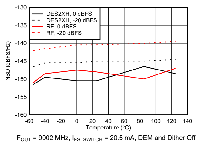
6-77. NSD vs Temperature
