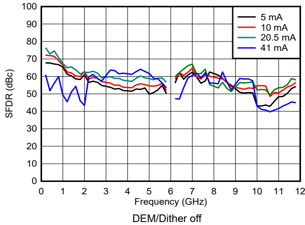
6-92. SFDR vs Frequency and Output Current in DES2X Modes
