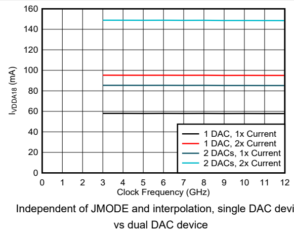
6-208. VDDA18 Current vs Clock Frequency and DAC Mode
