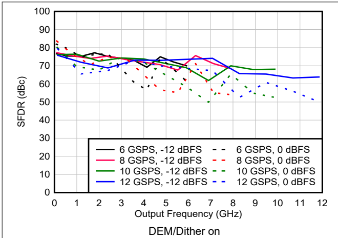
Figure 6-104. SFDR vs Frequency and Sample Rate in DES2X Modes
