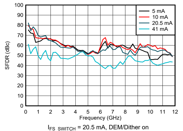
Figure 6-91. SFDR vs Frequency and Output Current in NRZ/RF Modes
