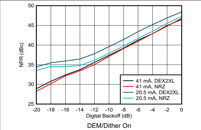
6-188. Noise Power Ratio vs Digital Backoff: 1 st Nyquist Zone
