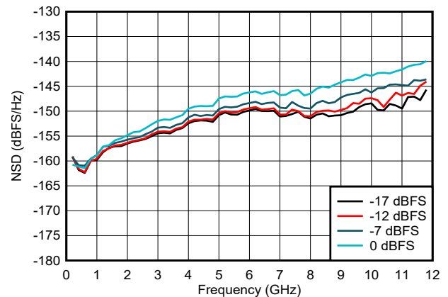
6-65. NSD vs Output Frequency and Digital Amplitude
