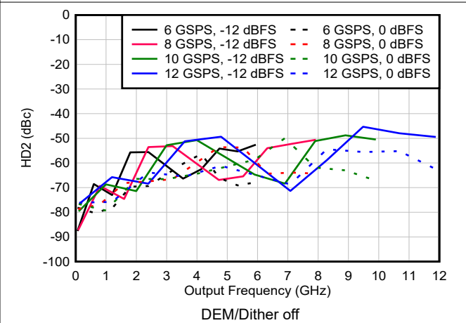
6-149. HD2 vs Frequency and Sample Rate in DES2X Modes
