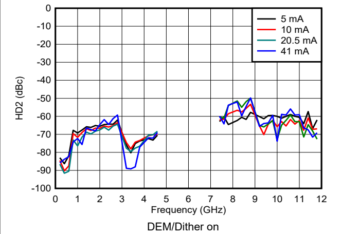
6-137. HD2 vs Frequency and Output Current in DES2X Modes
