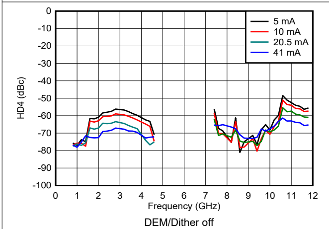
Figure 6-168. HD4 vs Frequency and Output Current in DES2X Modes
