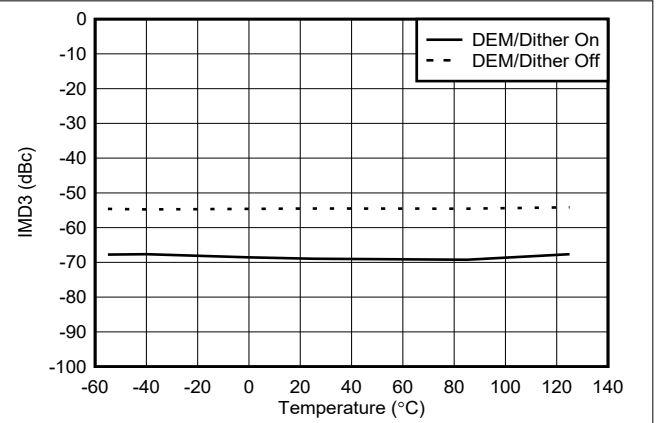
6-129. IMD3 vs Temperature in DES2XH Mode at 9002 MHz
