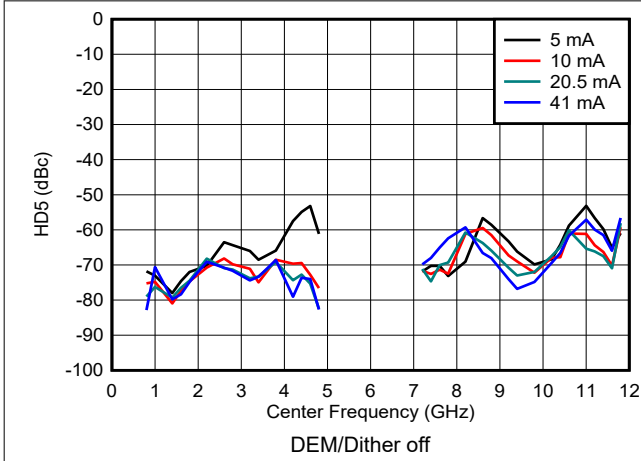
6-176. HD5 vs Frequency and Output Current in DES2X Modes
