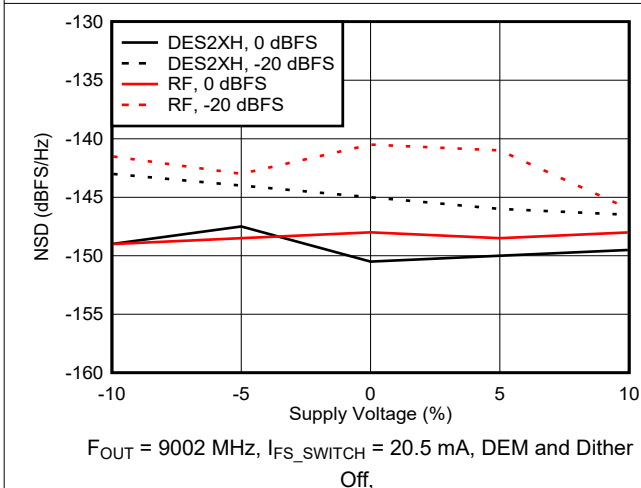
6-80. NSD vs Supply Voltage
