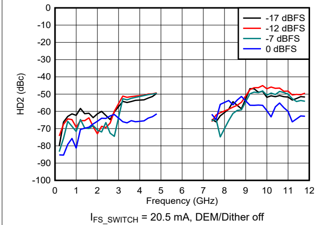
Figure 6-142. HD2 vs Frequency and Digital Amplitude in DES2X Modes
