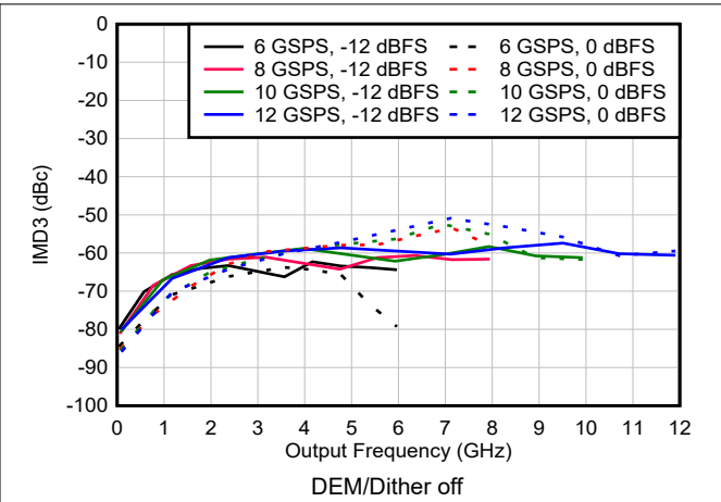
6-123. IMD3 vs Frequency and Sample Rate in NRZ/RF Modes
