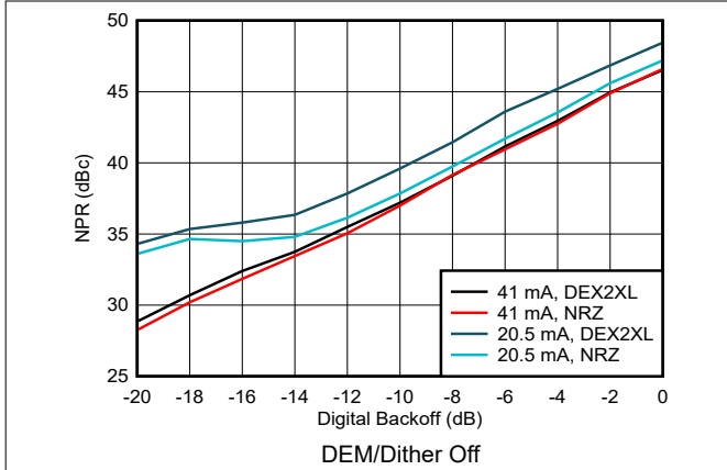
6-187. Noise Power Ratio vs Digital Backoff: 1 st Nyquist Zone
