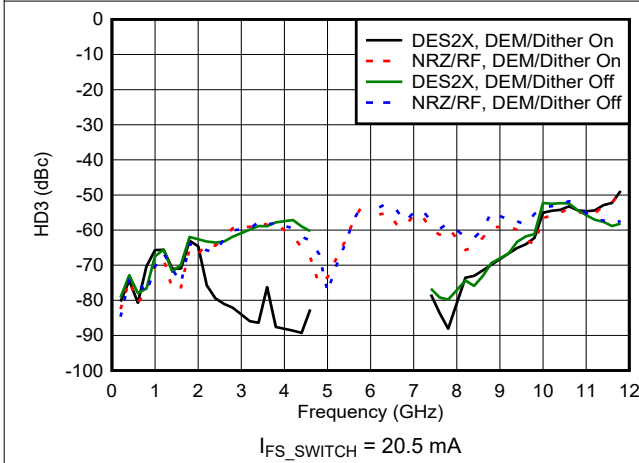
Figure 6-88. HD3 vs Frequency and Mode
