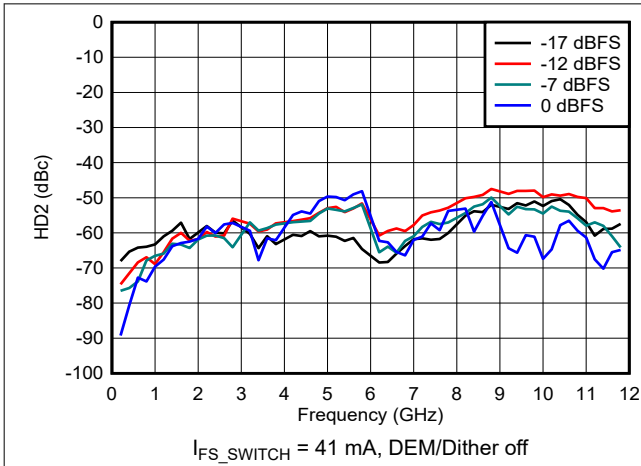
Figure 6-140. HD2 vs Frequency and Digital Amplitude in NRZ/RF Modes
