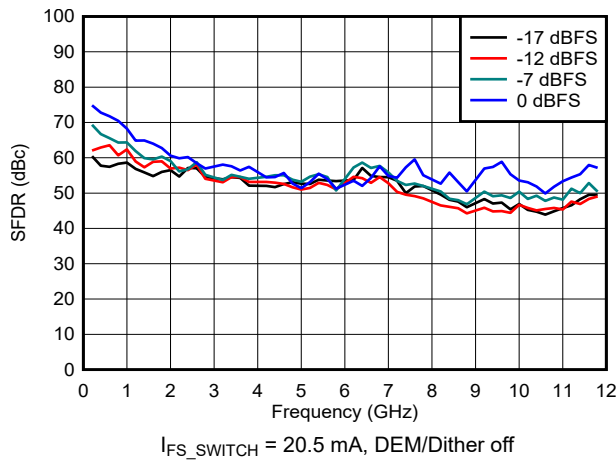
6-94. SFDR vs Frequency and Digital Amplitude in NRZ/RF Modes
