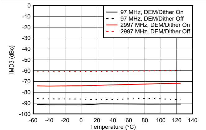
6-127. IMD3 vs Temperature in DES2XL Mode
