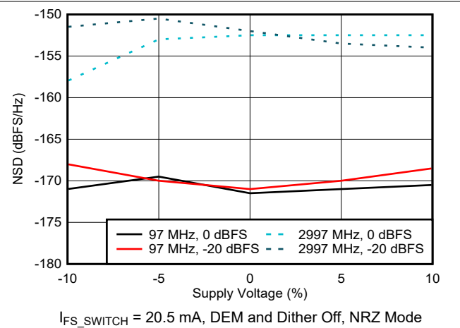
6-79. NSD vs Supply Voltage
