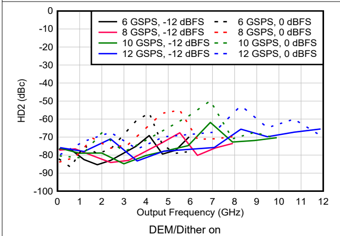
6-148. HD2 vs Frequency and Sample Rate in DES2X Modes
