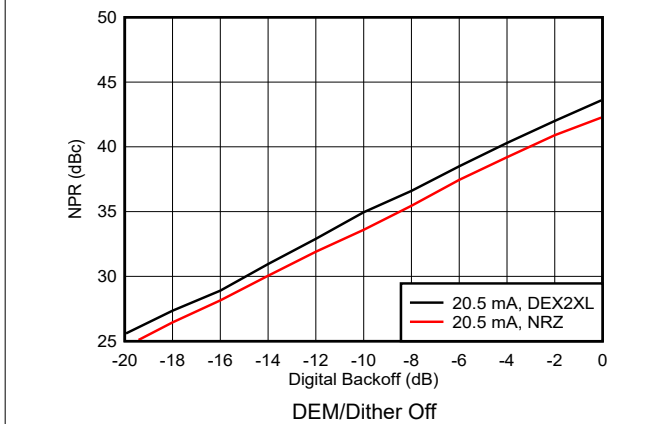
6-189. Noise Power Ratio vs Digital Backoff: 2 nd Nyquist Zone
