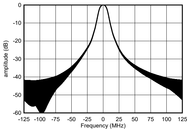
8-15. Digital Spectrum for NLFM Chirp
