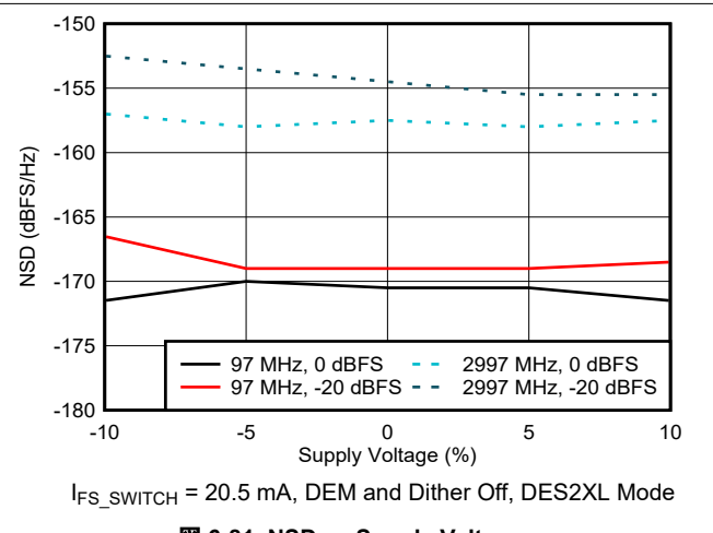
6-81. NSD vs Supply Voltage
