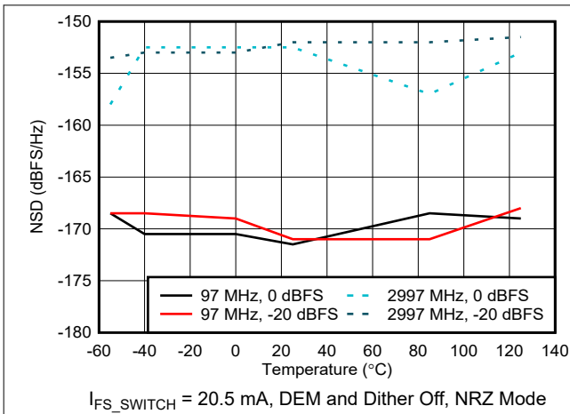
6-76. NSD vs Temperature
