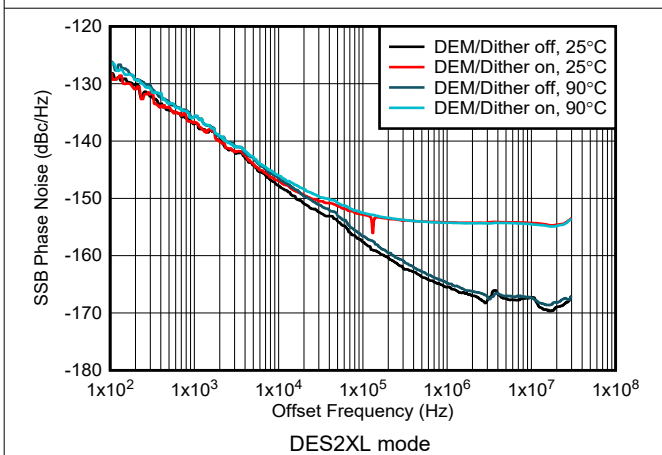
Figure 6-197. Phase Noise vs Offset Frequency at 1 GHz
