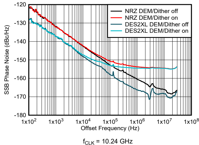
8-5. Phase Noise vs Offset Frequency at 1 GHz
