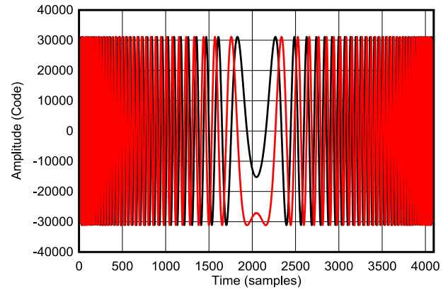
8-14. Complex Time Domain of NLFM Chirp (Red = real, Black = imag)
