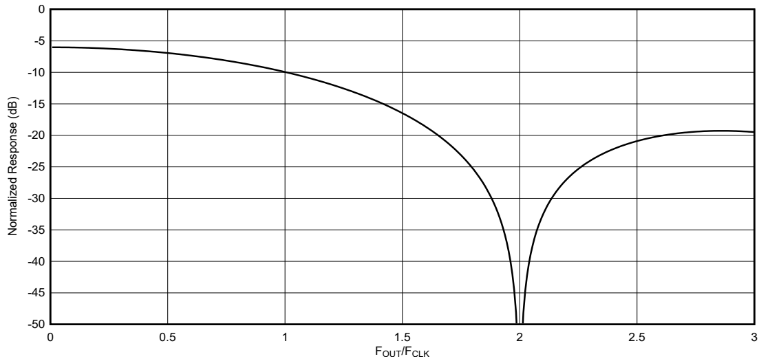
☒ 7-6. RTZ Mode Output Frequency Response
