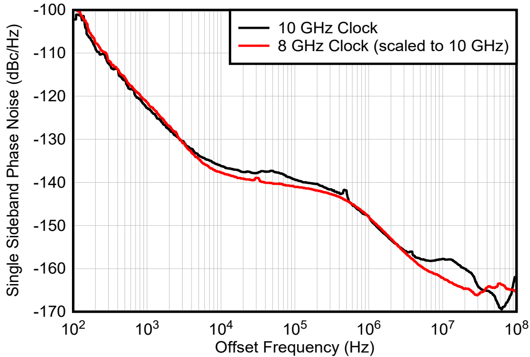
8-12. 8 GHz and 10 GHz Clock Phase Noise
