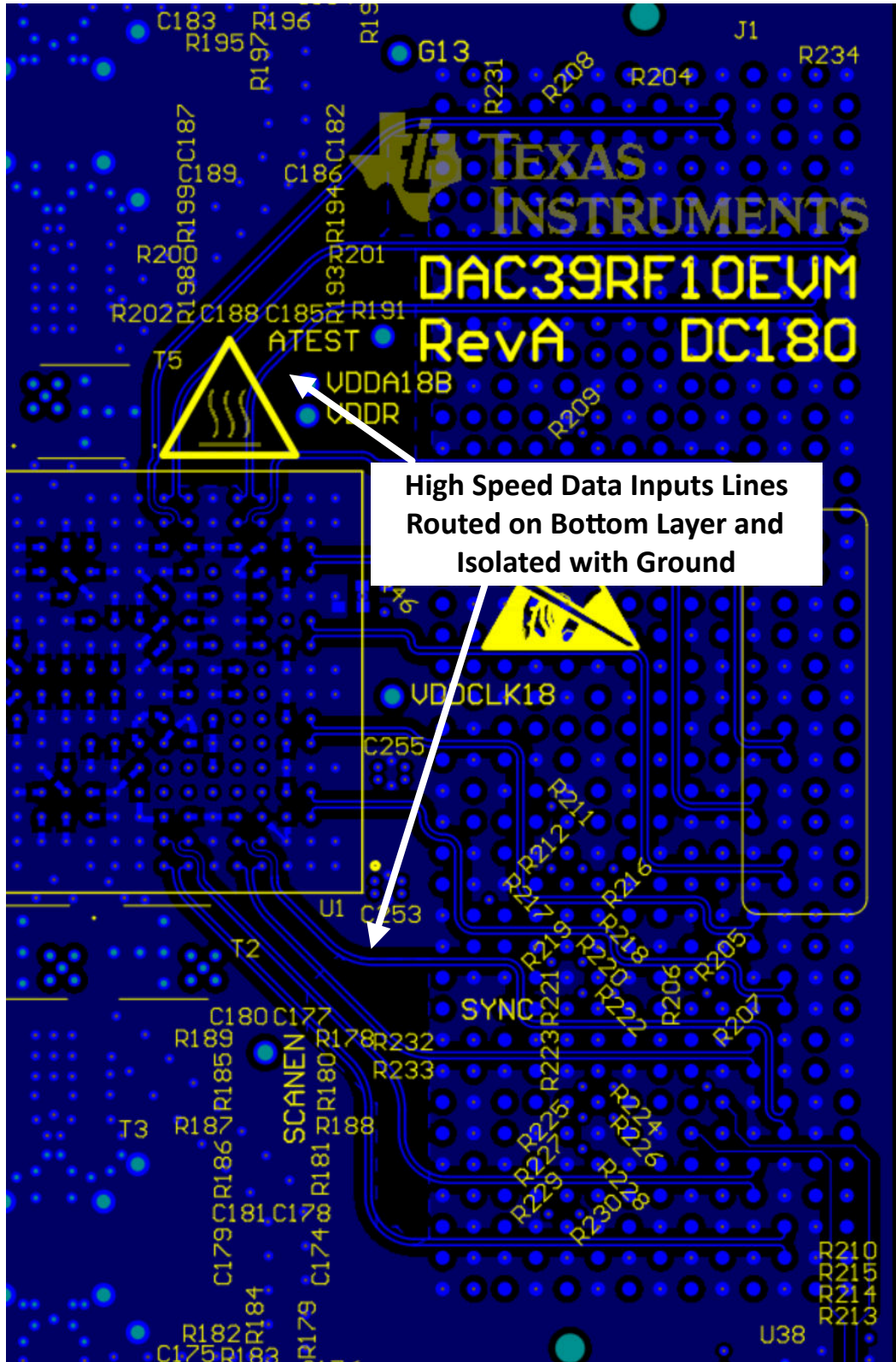
図 8-29. Serdes Bottom Layer Routing with Ground Isolation
