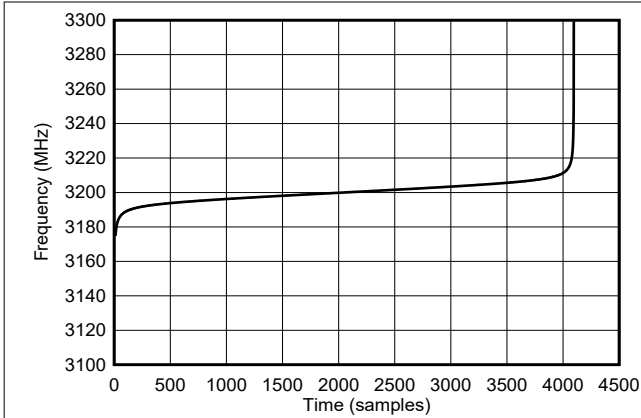
8-13. NLFM Frequency Ramp
