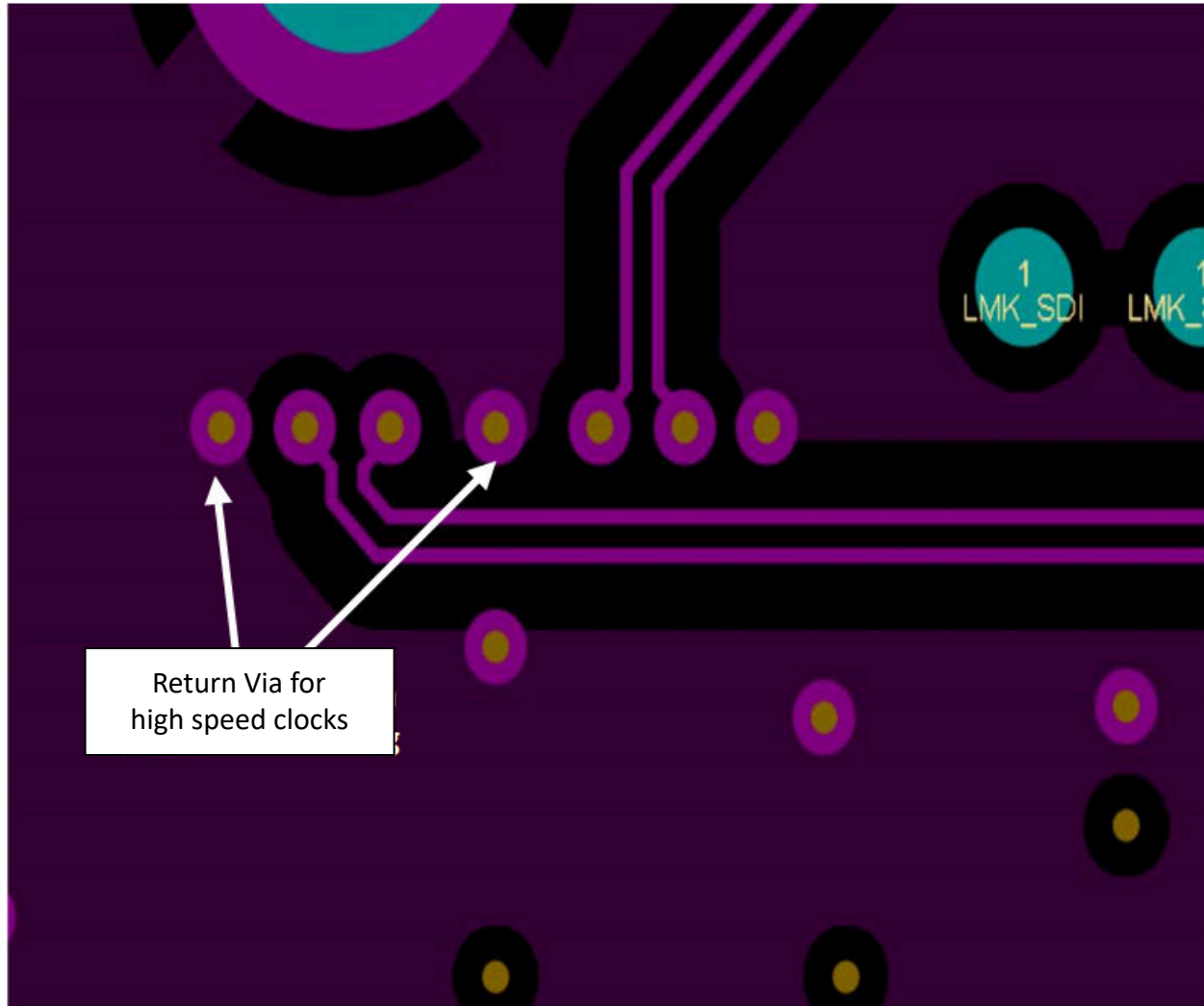
☒ 8-26. Return Vias for High Speed Clock
