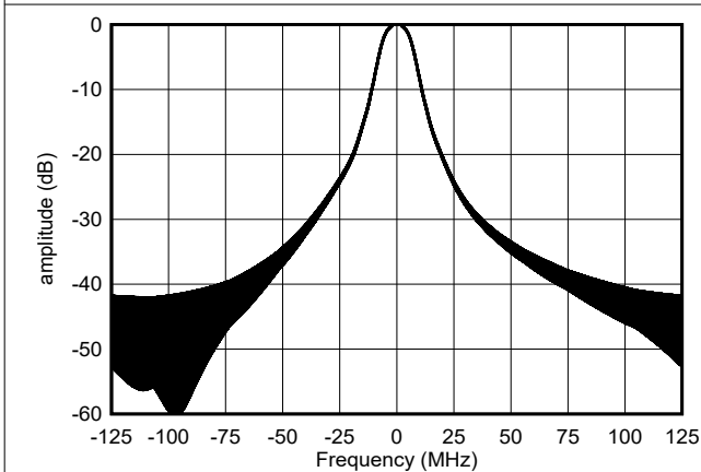
8-15. Digital Spectrum for NLFM Chirp
