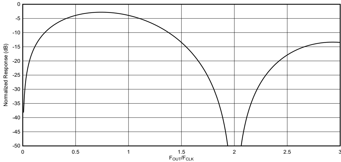
图 7-8. RF Mode Output Frequency Response
