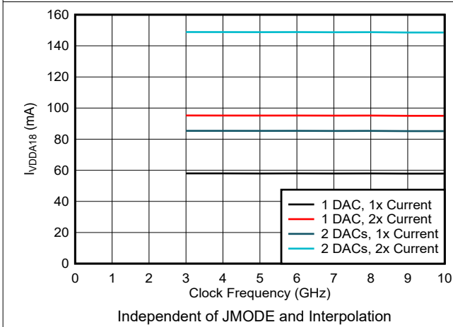
6-46. VDDA18 Current vs Clock Frequency and DAC Mode
