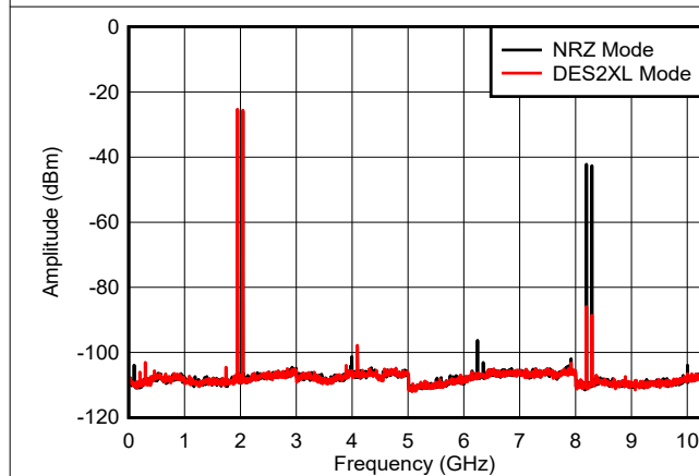
图 6-32. Dual Tone, f_{\text{OUT}} = 1997 \text{ MHz} , 0 dBFS
