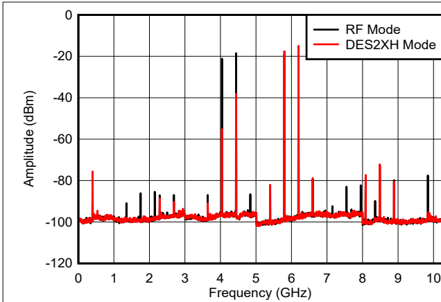
図 6-38. Dual Tone, f_{\text{OUT}} = 5997\text{ MHz} , 0 dBFS
