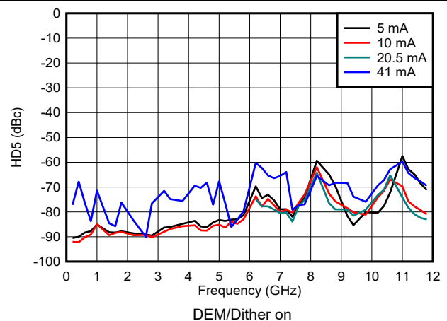
图 6-175. HD5 vs Frequency and Output Current in NRZ/RF Modes
