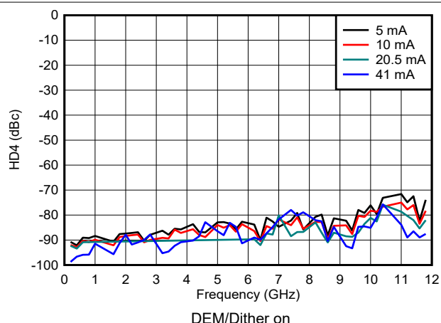
図 6-167. HD4 vs Frequency and Output Current in NRZ/RF Modes
