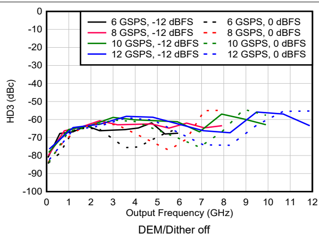
図 6-165. HD3 vs Frequency and Sample Rate in DES2X Modes
