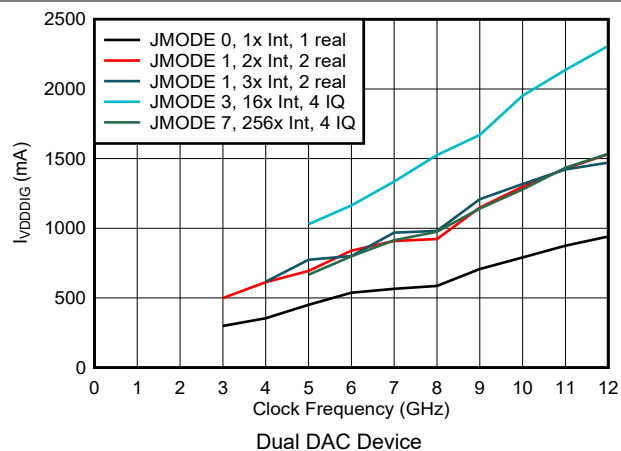
Figure 6-216. VDDDIG Current vs Clock Frequency and Digital Mode
