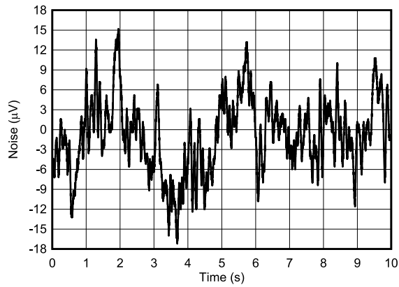
7-45. DAC Output Noise: 0.1 Hz to 10 Hz
