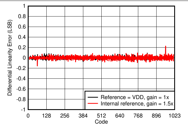
7-2. Differential Linearity Error vs Digital Input Code
