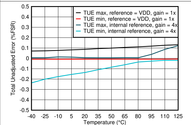
7-16. Total Unadjusted Error vs Temperature
