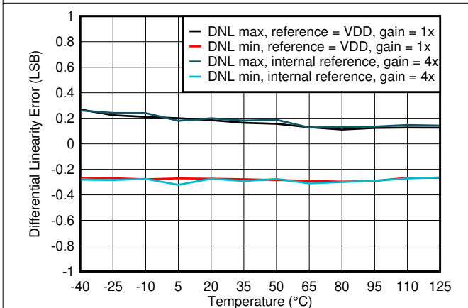
7-15. Differential Linearity Error vs Temperature
