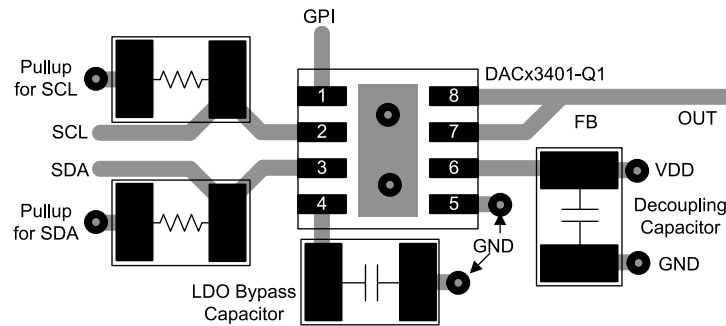
Figure 11-1. Layout Example
