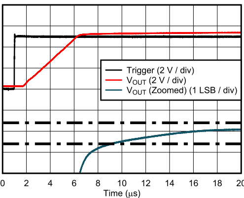
7-35. Glitch Impulse, Rising Edge, 1-LSB Step
