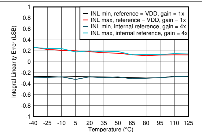
7-14. Integral Linearity Error vs Temperature
