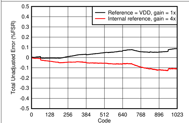
7-13. Total Unadjusted Error vs Digital Input Code
