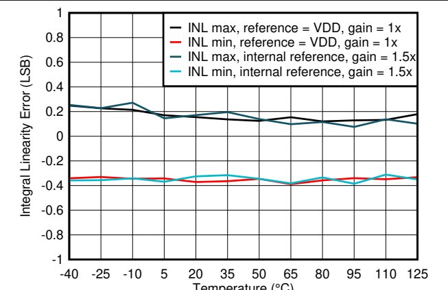
7-4. Integral Linearity Error vs Temperature
