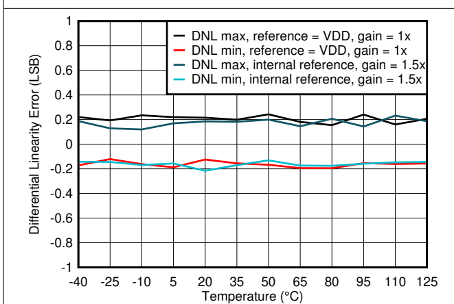
7-5. Differential Linearity Error vs Temperature
