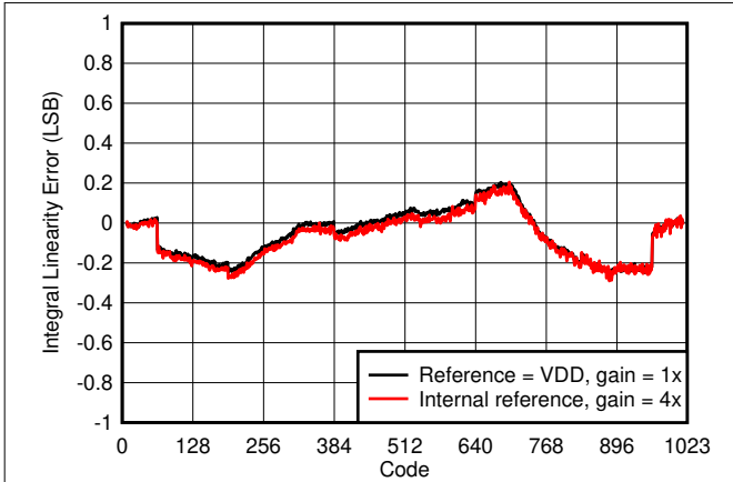
7-11. Integral Linearity Error vs Digital Input Code
