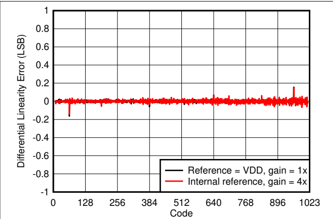
7-12. Differential Linearity Error vs Digital Input Code
