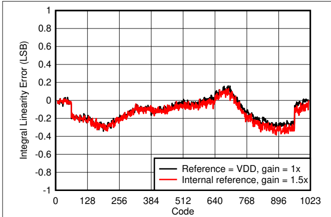
7-1. Integral Linearity Error vs Digital Input Code
