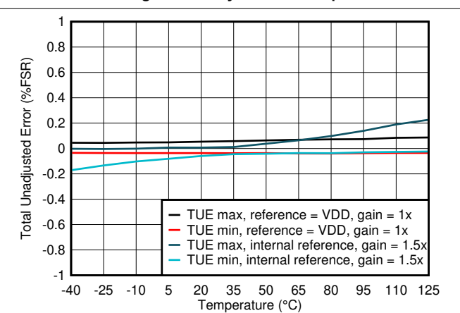
7-6. Total Unadjusted Error vs Temperature
