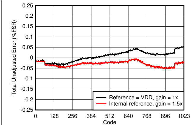
7-3. Total Unadjusted Error vs Digital Input Code
