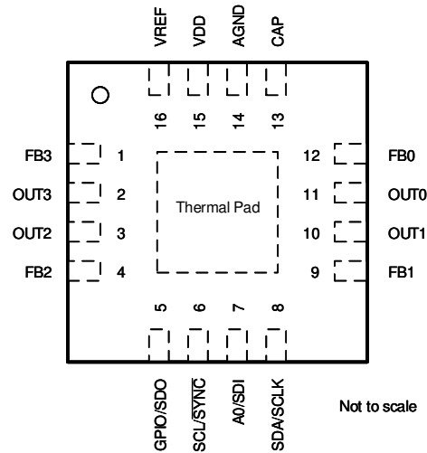
図 5-1. RTE Package, 16-pin WQFN, Top View
