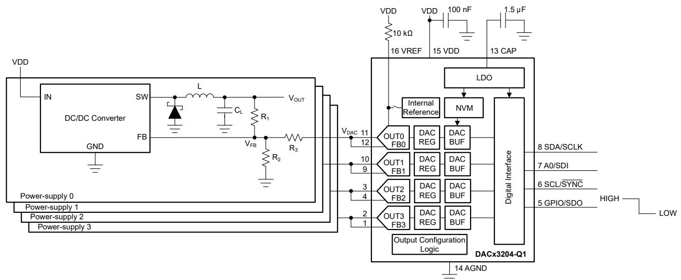
8-1. APD Biasing
