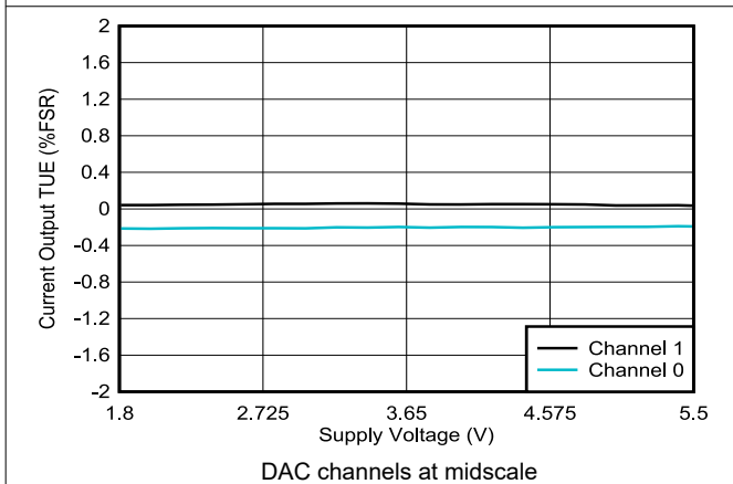
6-44. Current Output TUE vs Supply Voltage
