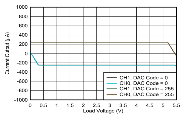
6-47. Current Output vs Load Voltage
