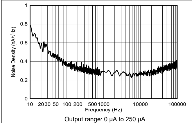
6-52. Current Output Noise Density
