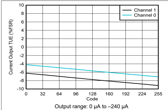
6-42. Current Output TUE vs Digital Input Code
