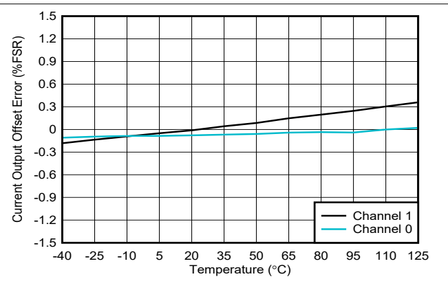
6-45. Current Output Offset Error vs Temperature
