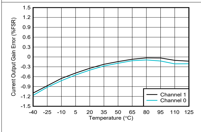
6-46. Current Output Gain Error vs Temperature
