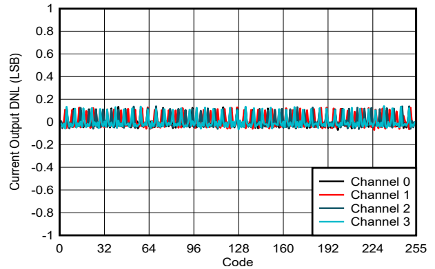
6-38. Current Output DNL vs Digital Input Code
