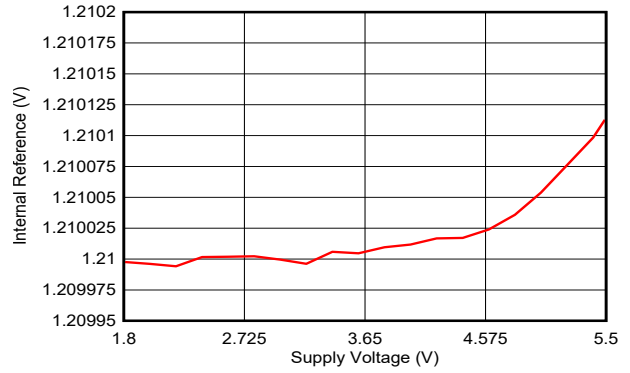
6-63. Internal Reference vs Supply Voltage
