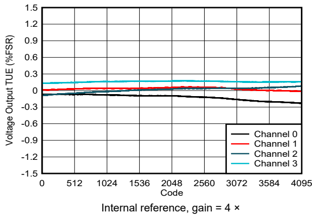
6-12. Voltage Output TUE vs Digital Input Code
