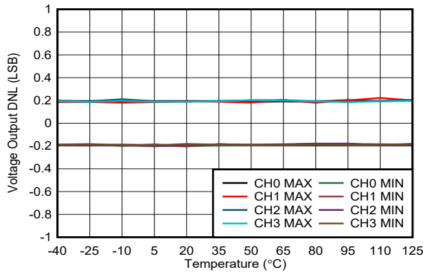
6-10. Voltage Output DNL vs Temperature
