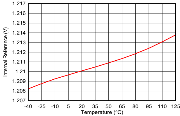
6-62. Internal Reference vs Temperature
