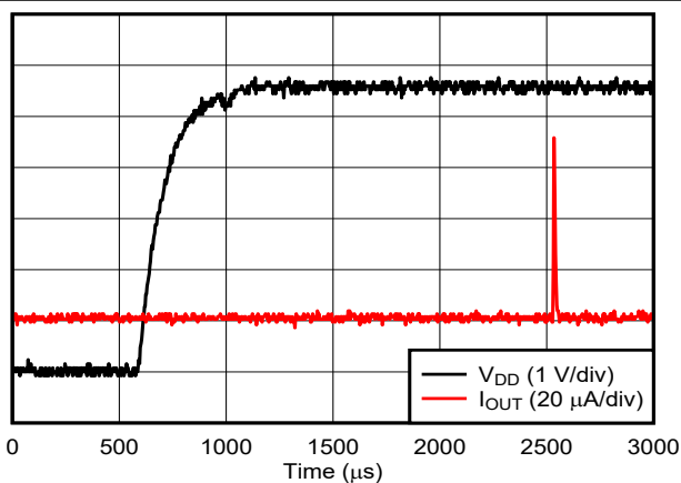
6-49. Current Output Settling Time: Rising Edge ( \frac{1}{4} to \frac{3}{4} scale)
