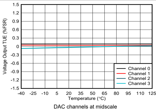
6-14. Voltage Output TUE vs Temperature
