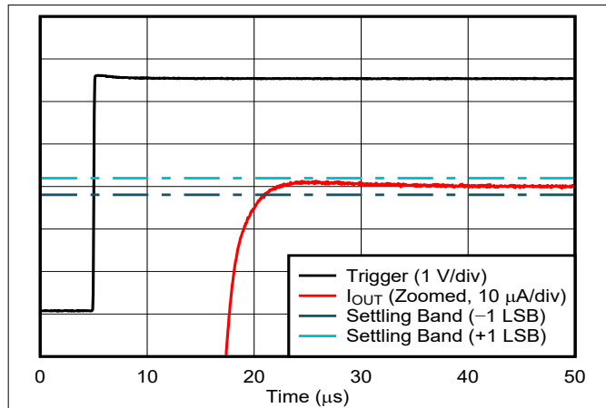
6-49. Current Output Settling Time: Rising Edge ( \frac{1}{4} to \frac{3}{4} scale)
