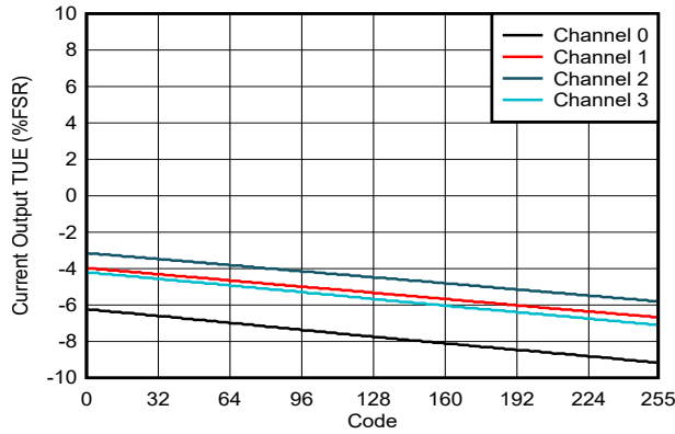
Figure 6-43. Current Output TUE vs Digital Input Code
