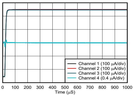
6-51. Current Output Power-On Glitch
