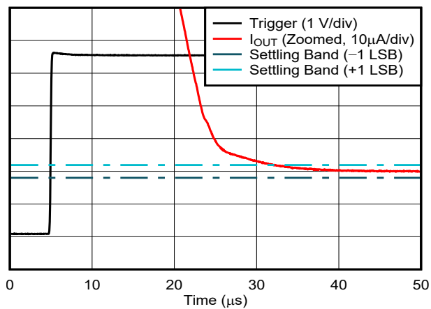
6-50. Current Output Settling Time: Falling Edge ( \frac{3}{4} to \frac{1}{4} scale)
