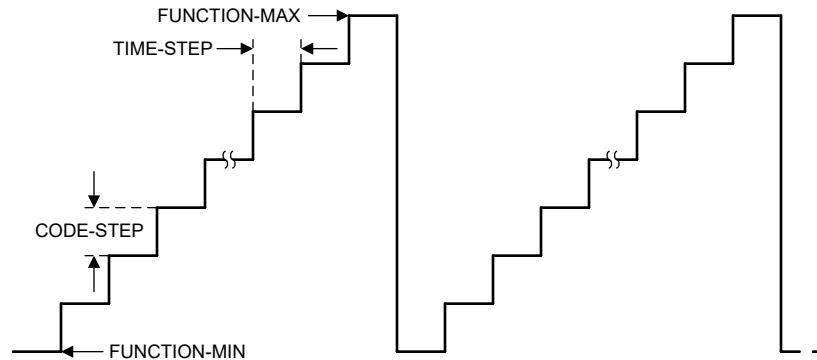
Figure 7-13. Sawtooth Waveform
