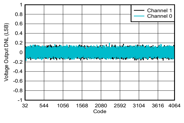
6-9. Voltage Output DNL vs Digital Input Code
