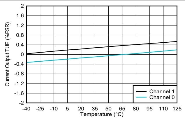
6-37. Current Output TUE vs Temperature
