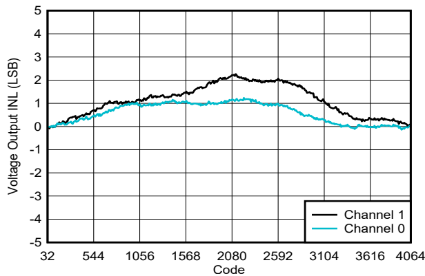
6-4. Voltage Output INL vs Digital Input Code
