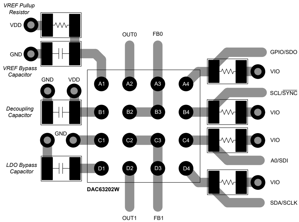
8-4. Layout Example
