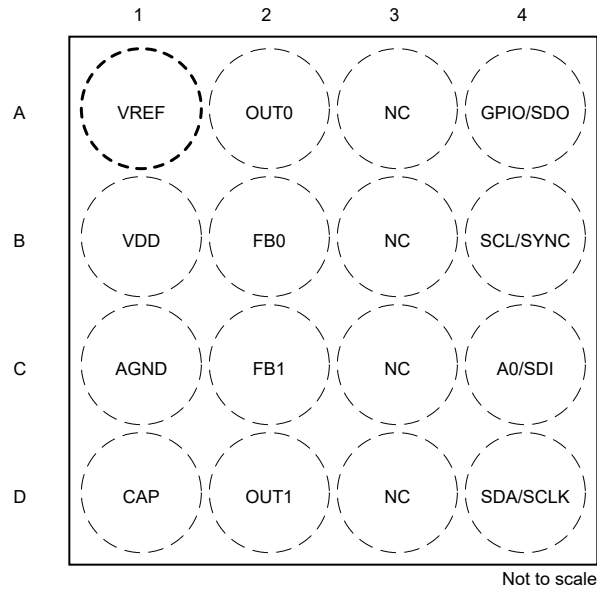
図 5-1. YBH (16-pin DSBGA) Package, Top View
