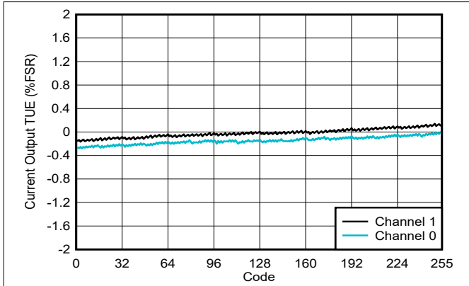
6-36. Current Output TUE vs Digital Input Code
