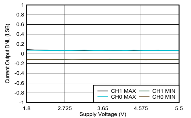
Figure 6-35. Current Output DNL vs Supply Voltage
