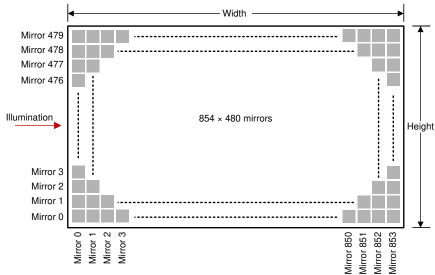
6-15. Micromirror Array Physical Characteristics
