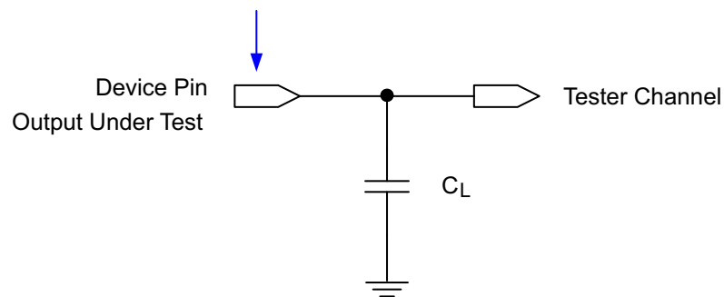
6-13. Test Load Circuit for Output Propagation Measurement
