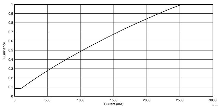
7-2. Luminance vs LED Current
