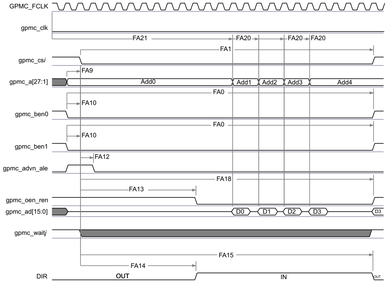
FIG 5-30. GPMC / NOR Flash - Asynchronous Read - Page Mode 4x16-bit Timing (1)(2)(3)(4)
