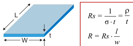
FIG 7-3. Depiction of Sheet Resistivity and Resistance
