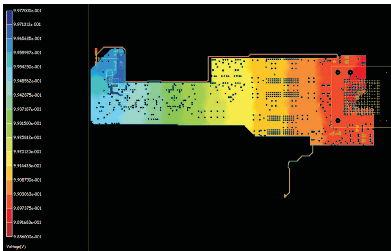
図 7-16. vdd_dspeve Voltage/IR Drop [All Layers]
