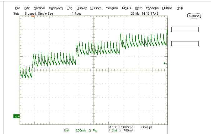
8-3. Microstepping Waveform, Slow Decay on Increasing Steps
