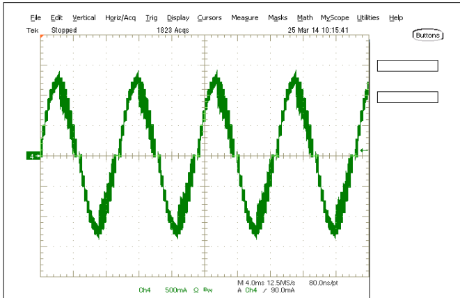
8-2. Microstepping Waveform, Phase A, Mixed Decay
