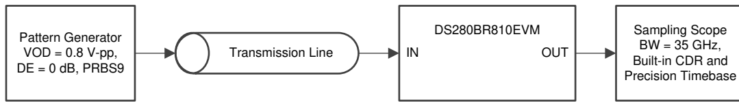
14. 5 in Rx and Minimal Tx Channel Test Setup
