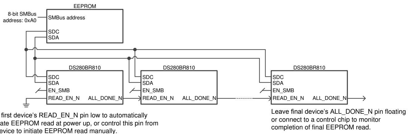
FIG 5. Example Daisy Chain for Multiple Device Single EEPROM Configuration
