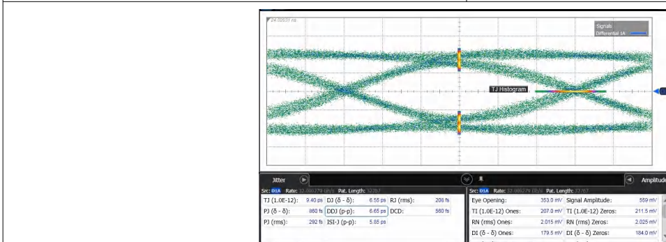
Fig 6-6. Through DS320PR 822 (7 dB Loss and DUT EQ = 0)
