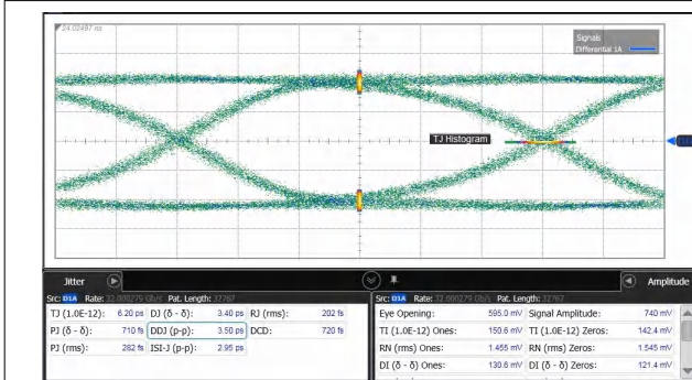
Fig 6-4. At BERT Source Output (1 dB Loss)
