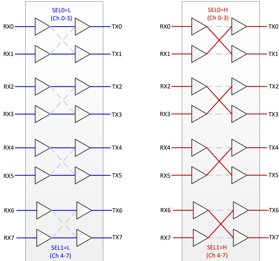
7-1. DS320822 Signal Flow Diagram for Cross-Point Mux Operation
