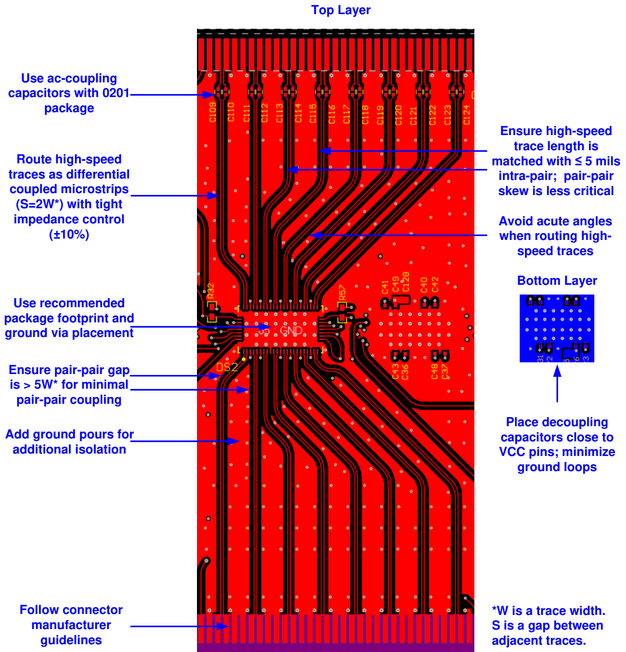
10-1. DS320PR822 Layout Example – Sub-Section of a PCIe Riser Card With CEM Connectors
