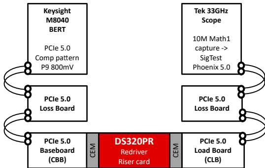
8-5. PCIe 5.0 Link Setup with the DS320PR822 the Link Elements
