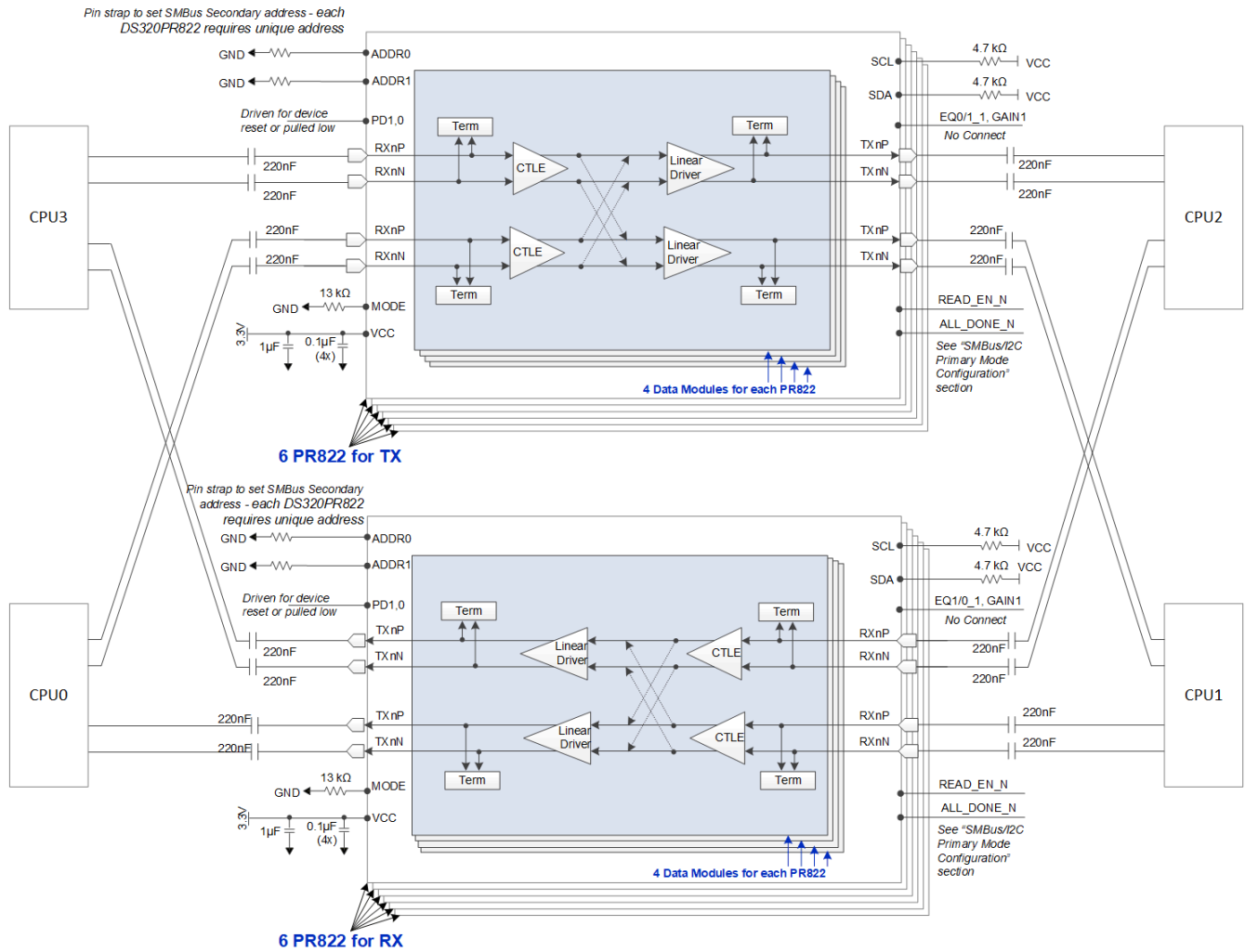
8-2. Simplified Schematic for UPI x24 Lane Configuration in SMBus/I 2 C Primary Mode
