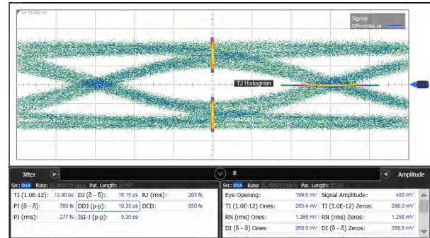
Fig 6-5. Through Baseline Calibration Trace Setup (7 dB Loss)
