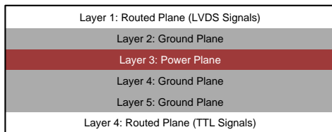
Figure 27. Six-Layer PCB
