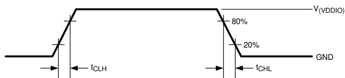
4-1. LVCMOS Transition Times
