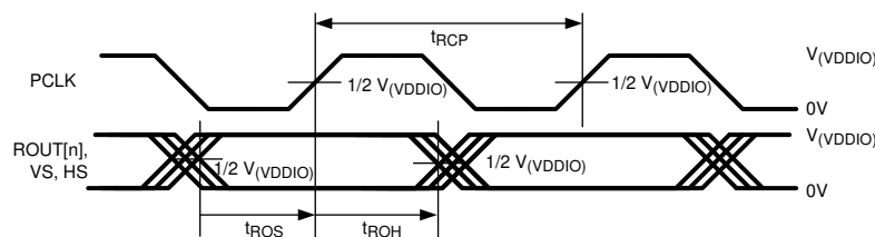
FIG 4-7. Deserializer Output Setup/Hold Times
