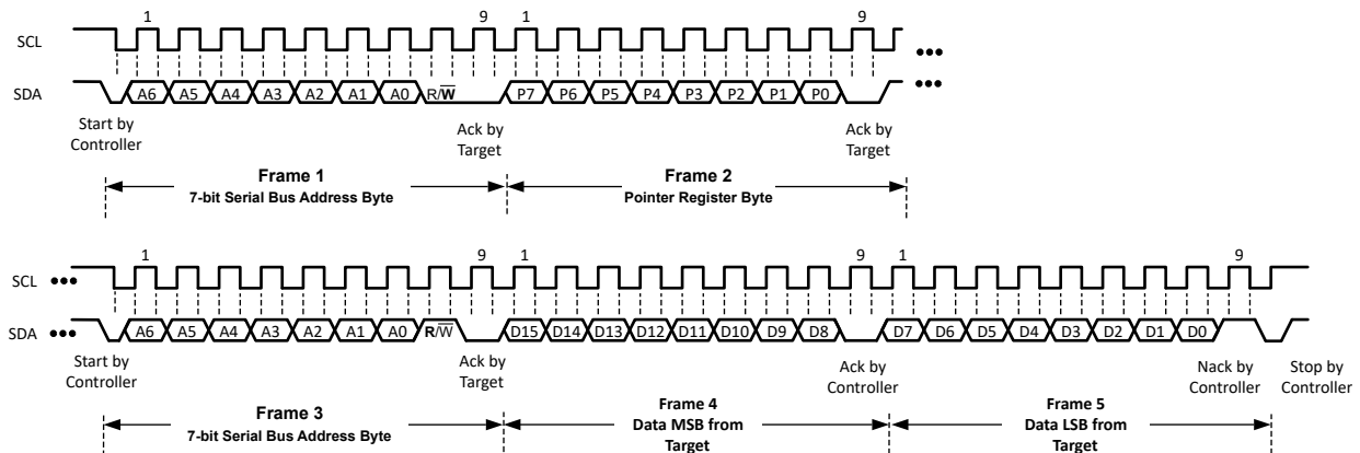
6-5. Read Frame
